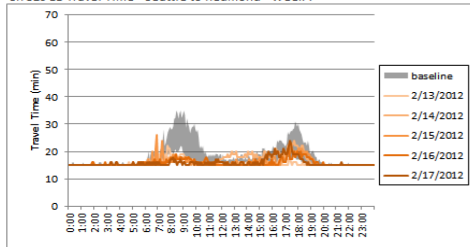
SR 520 EB Travel Time - Seattle to Redmond - Week 7
