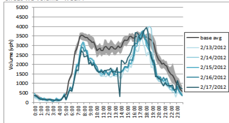
SR 520 EB Volume - Week 7
