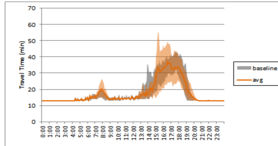
I-405 SB Travel Time - Bellevue to Tukwila - Week 7
