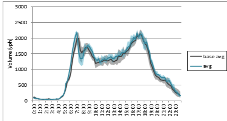
SR 522 EB Volume - Week 7
