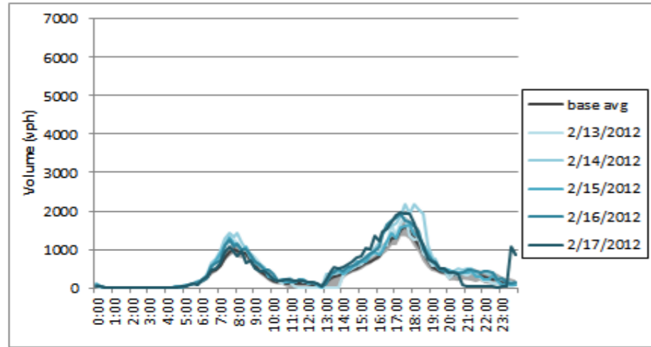
I-90 REV Volume - Week 7
