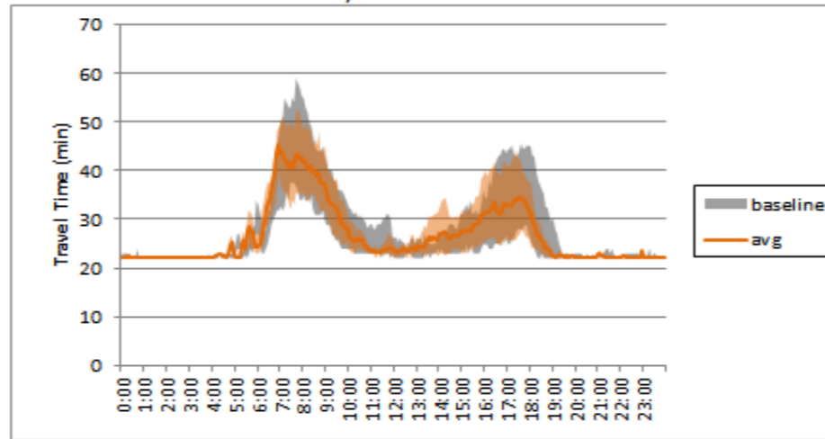
I-5 SB Travel Time - Seattle to Federal Way - Week 7
