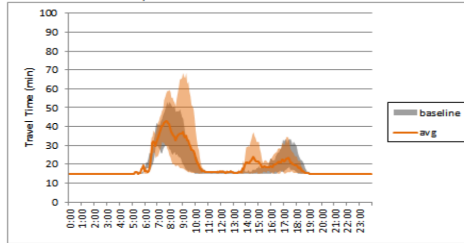
I-405 NB Travel Time - Bellevue to Lynnwood - Week 7
