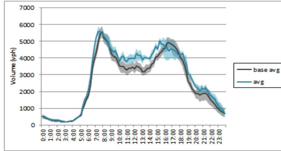
I-90 REV Volume - Week 7
