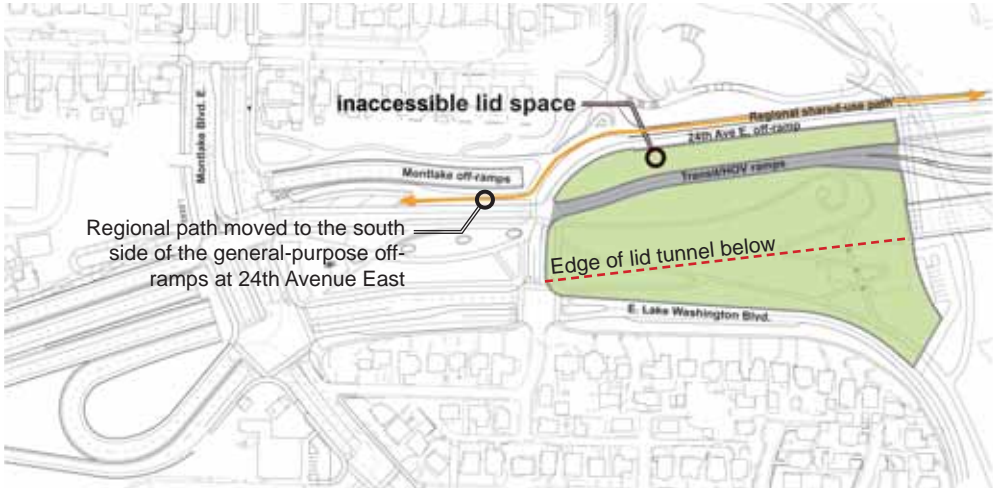
Option A - High Transit/HOV ramps (includes lid over lowered westbound off-ramp)
