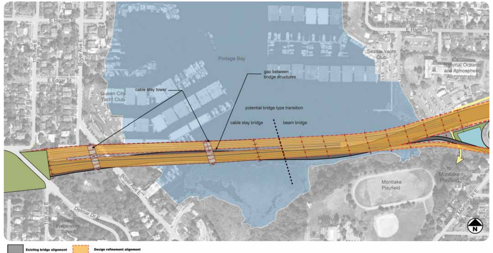
Cable stayed option alignment
