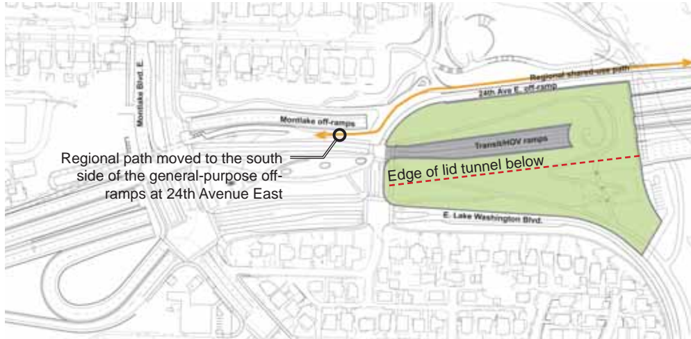
Option B - Lowered Transit/HOV ramps (includes lid over lowered westbound off-ramp)
