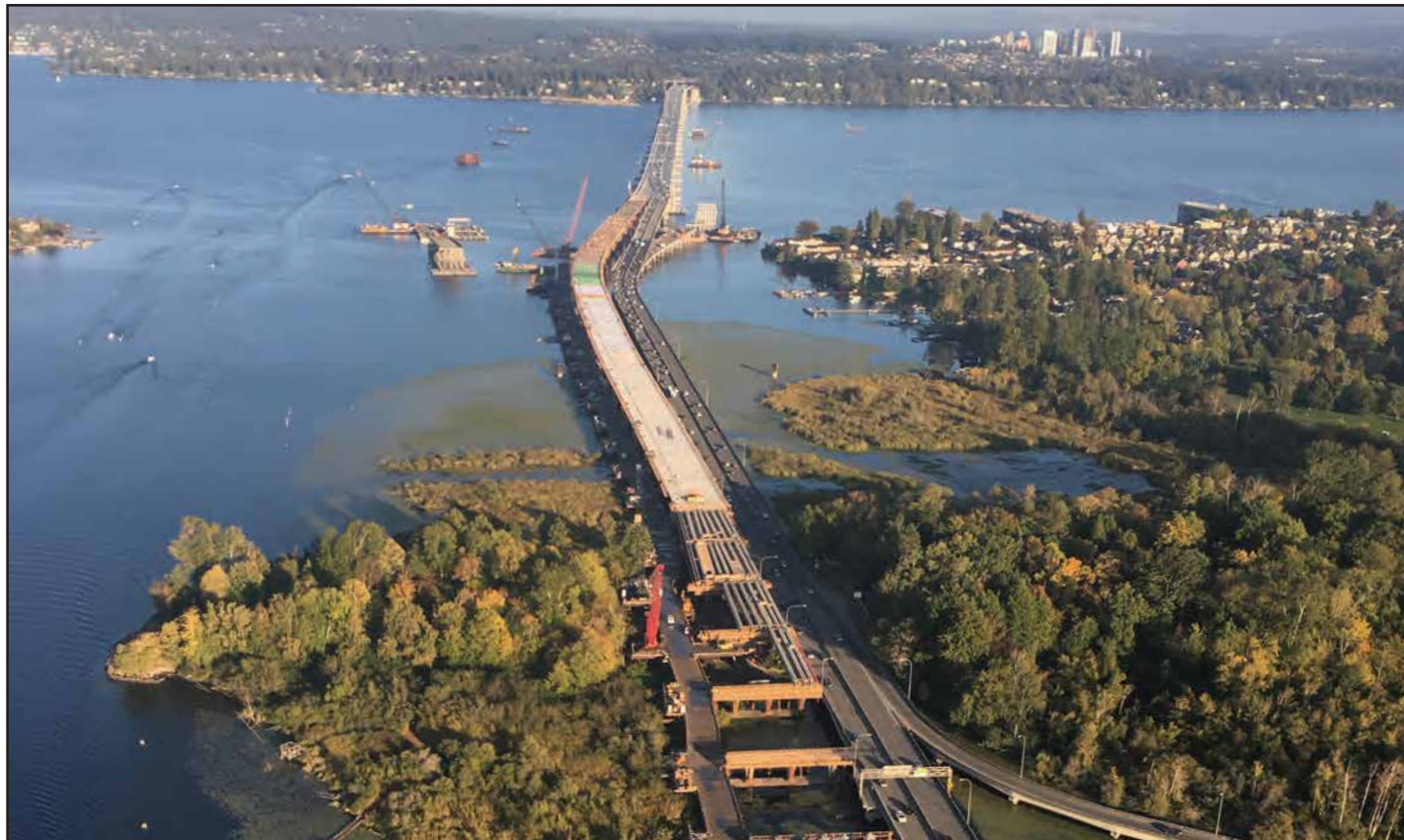
Crews in the foreground of this photo place girders and pour concrete for the West Approach Bridge North, which in the distance connects with the new SR 520 floating bridge. Photo taken: Sept. 28; courtesy of HDR.
