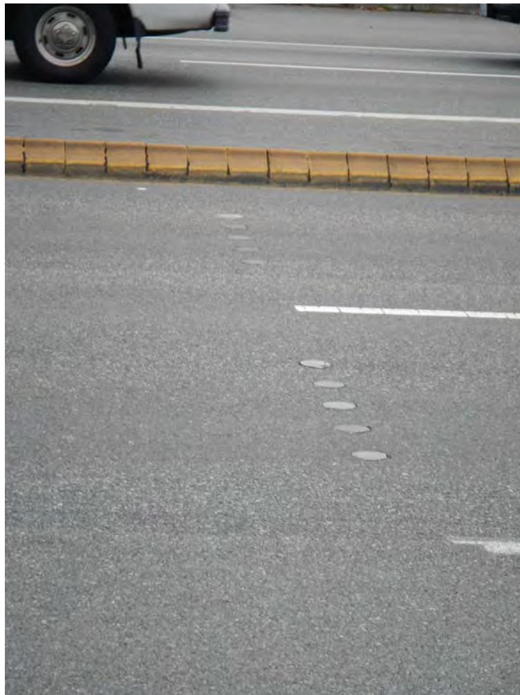
Figure 3-13. Sensys wireless vehicle detection system
