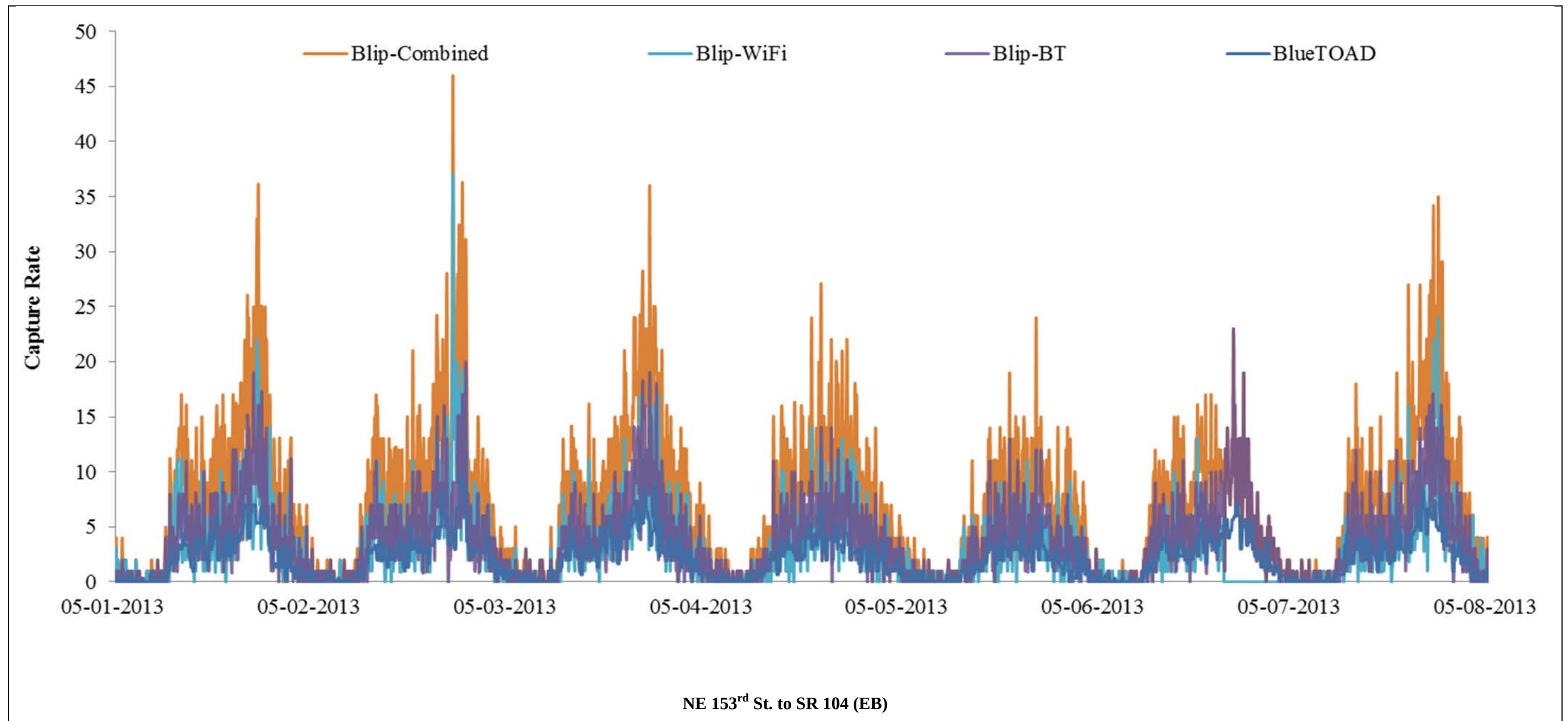
Figure 4-10. Comparing capture rates of different systems from NE 153rd St. to SR 104 (EB) for May 1, 2013, through May 8, 2013,
