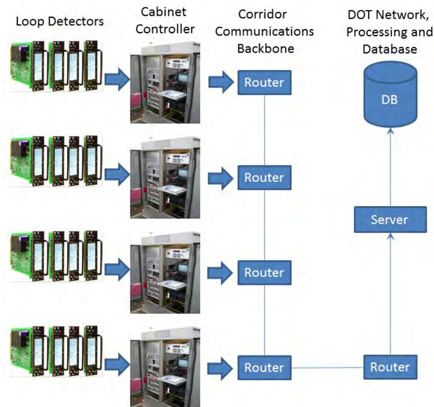
Figure 3-4. Loop detector system architecture
