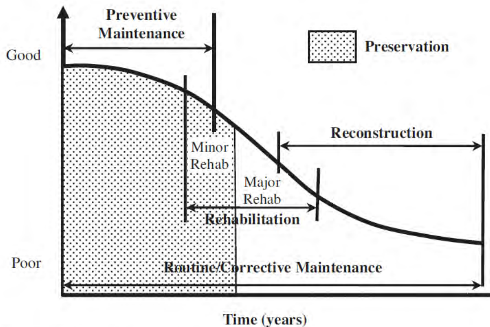
Figure 1. Relationship of Pavement Condition and Different Categories of pavement treatment (FHWA, Peshkin et. al).
