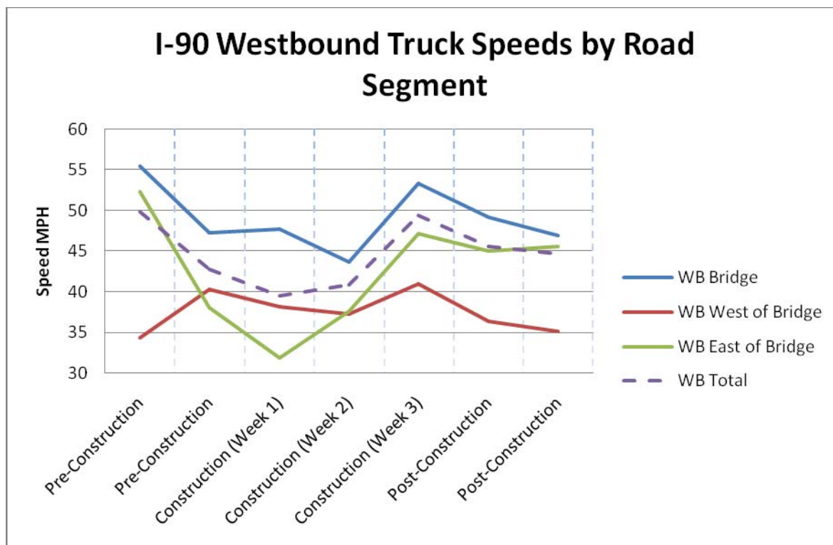
Figure A4-3: Westbound Truck Speed Comparison by Road Segment
