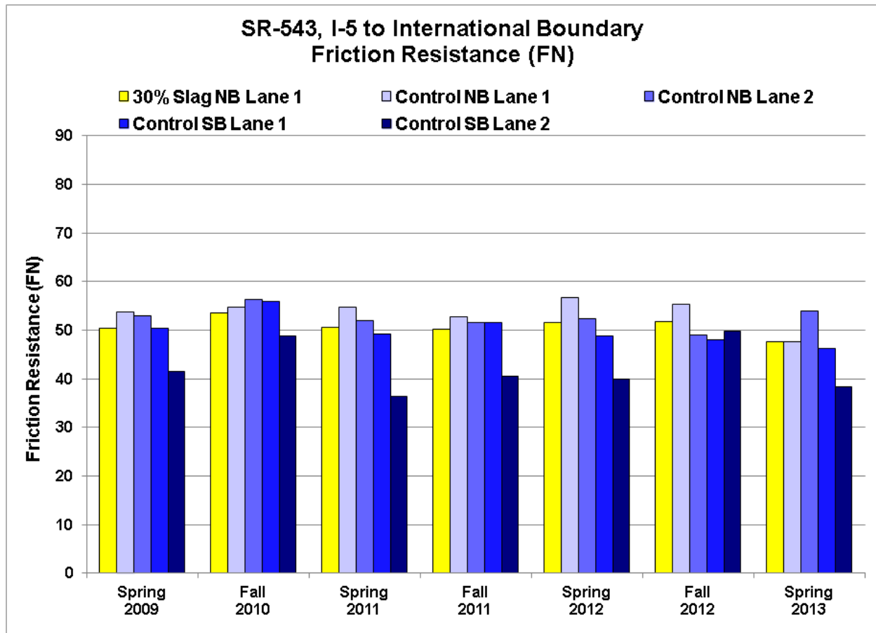
Figure 6. Friction resistance measurements for all lanes.
