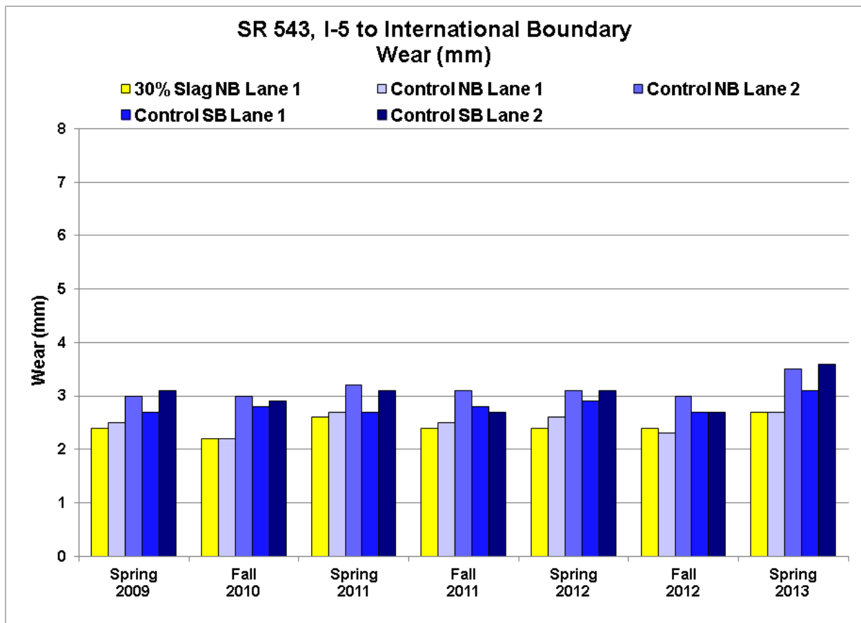
Figure 4. Wear measurements for all lanes.
