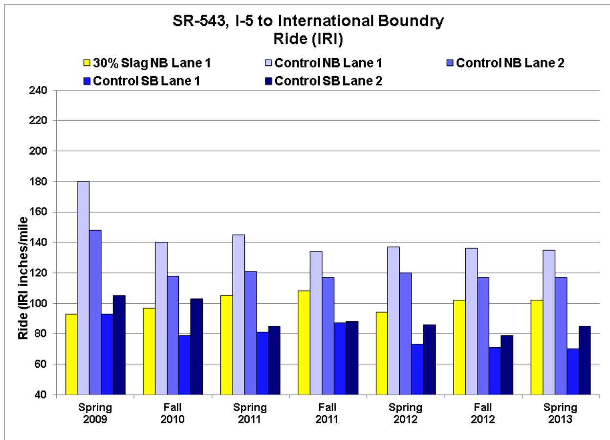
Figure 5. Ride measurements for all lanes.
