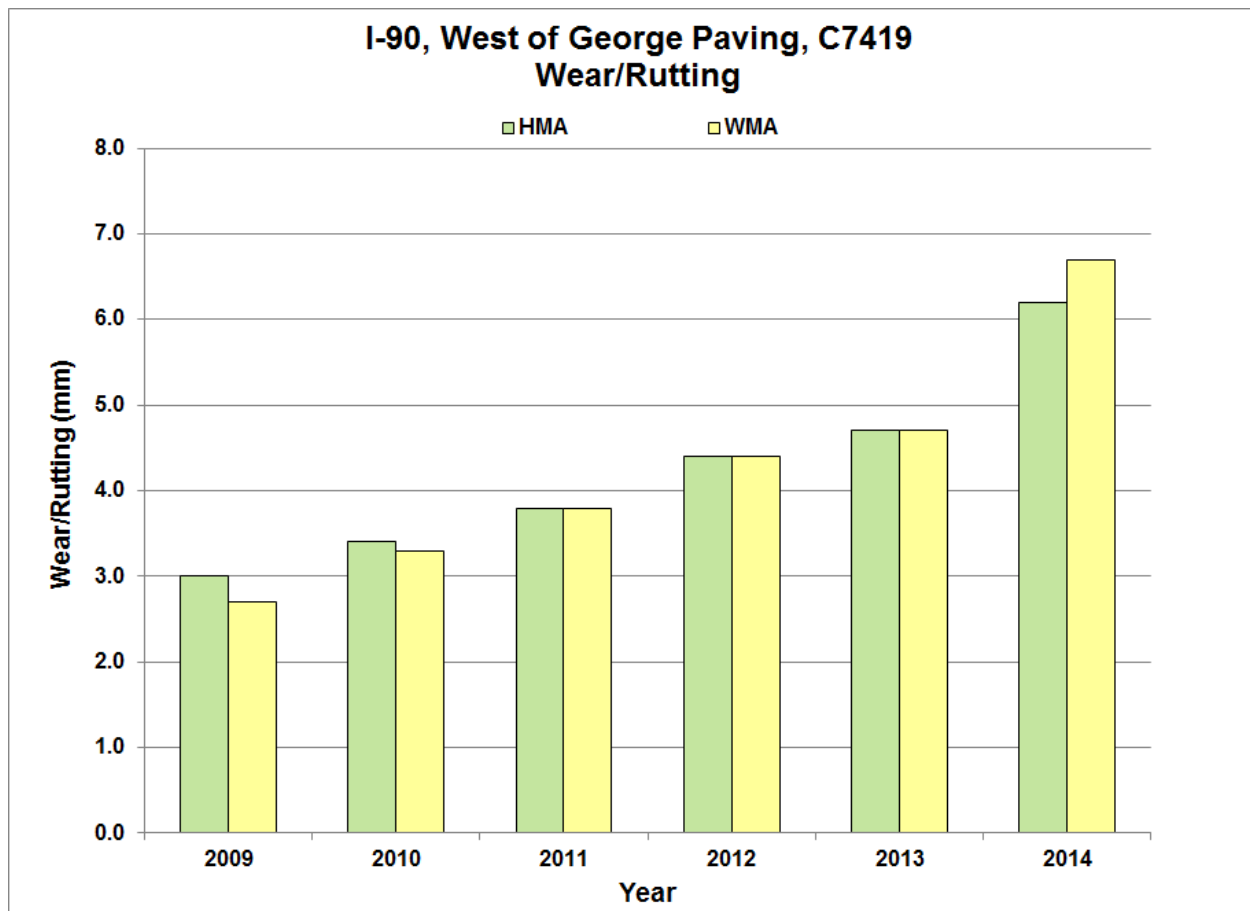
Figure 24. Wear/rutting measurements.
