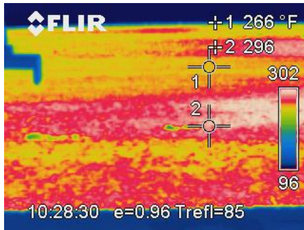
Figure 20. Thirty degree temperature differential in HMA.
