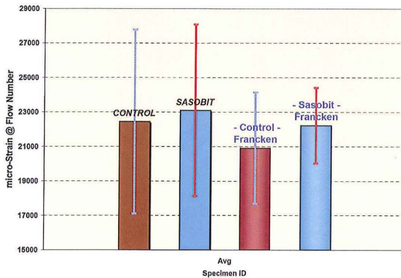
Figure 5: Accumulated Strain at Flow Number
