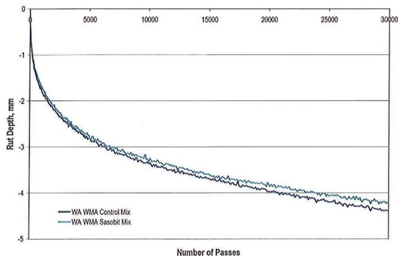
Figure 11: Comparison of Hamburg results of Control and WMA Sasobit Mixes
