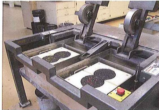
Figure 7: Hamburg Wheel Tracking Device
