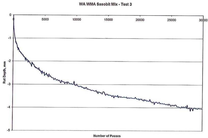
Figure A6: Hamburg Wheel Track Test Results of Washington WMA Sasobit Mix Test 3
