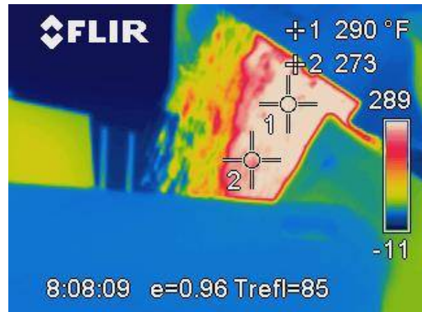
Figure 18. Thermal image of windrow elevator delivering WMA to the hopper.
