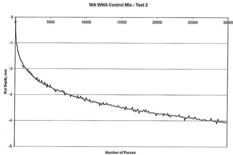
Figure A3: Hamburg Wheel Track Test Results of Washington WMA Control Mix Test 2
