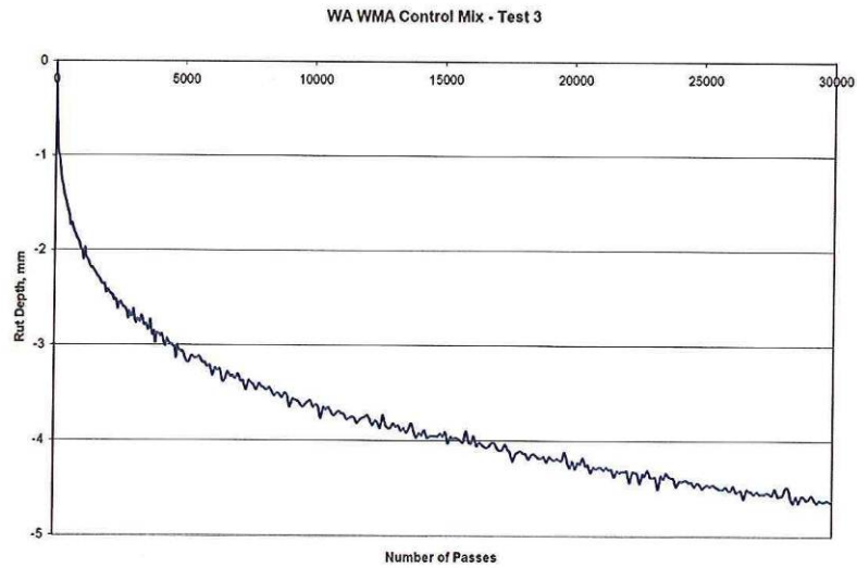
Figure A5: Hamburg Wheel Track Test Results of Washington WMA Control Mix Test 3
