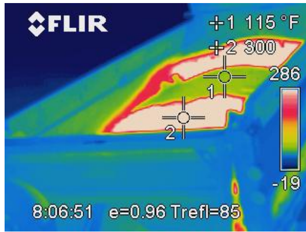
Figure 15. WMA crust temperature of 115°F leaving truck.
