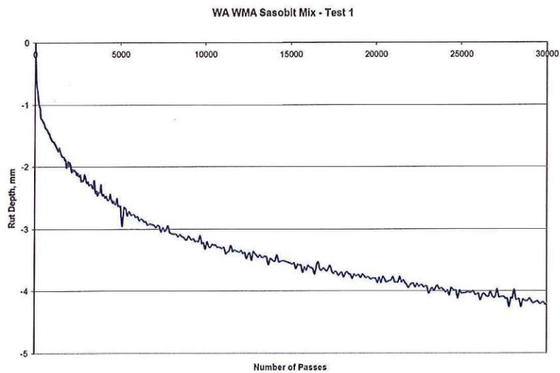
Figure A2: Hamburg Wheel Track Test Results of Washington WMA Sasobit Mix Test 1
