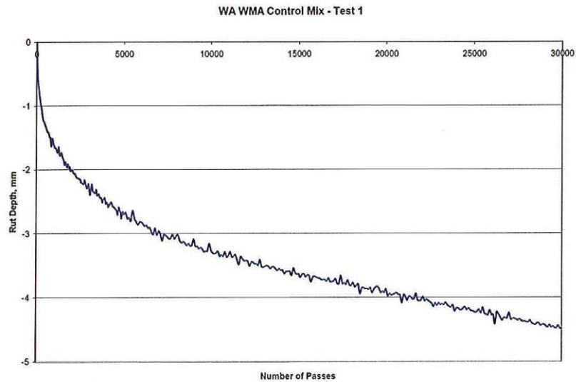
Figure A1: Hamburg Wheel Track Test Results of Washington WMA Control Mix Test 1
