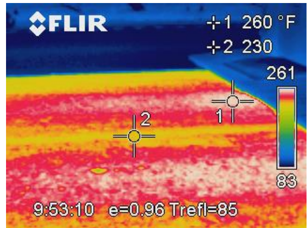
Figure 21. Thirty degree temperature differential in WMA.
