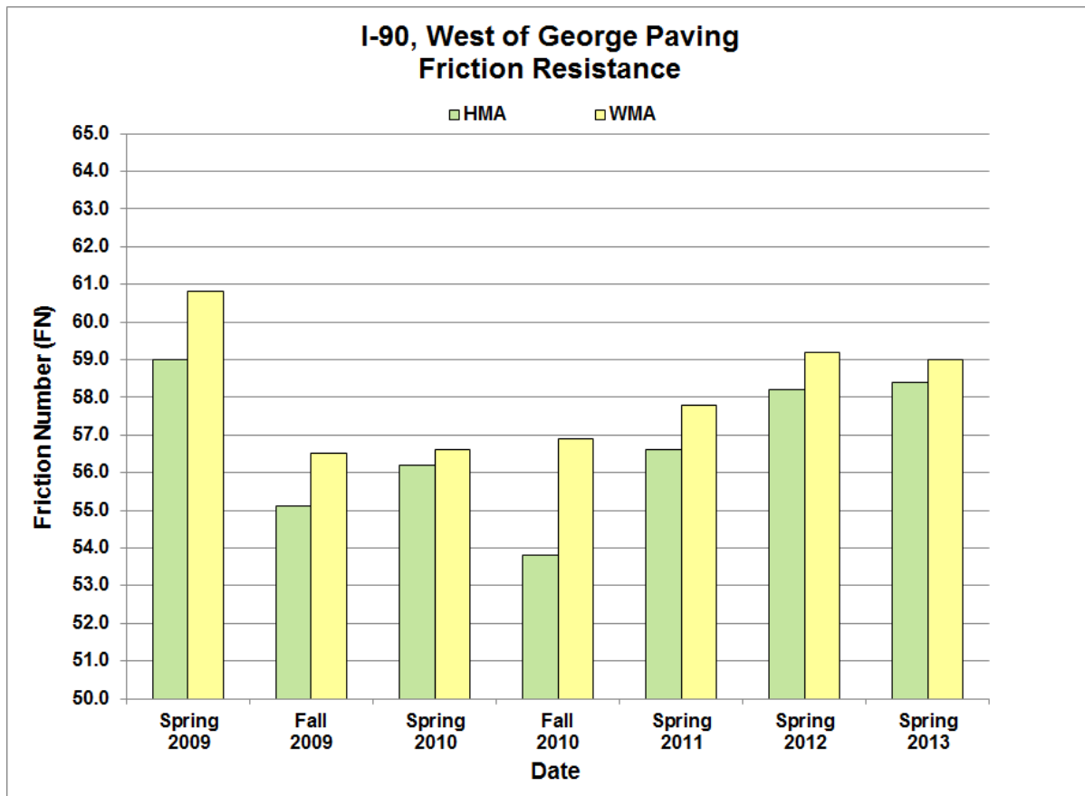
Figure 23. Friction resistance measurements over time for HMA and WMA sections.
