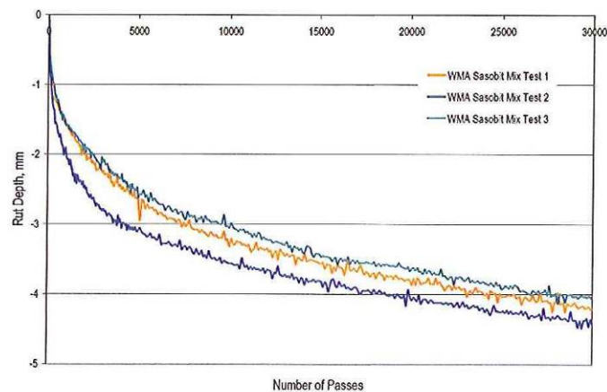
Figure 10: Hamburg Wheel Track Test Results of Washington WMA Sasobit Mix
