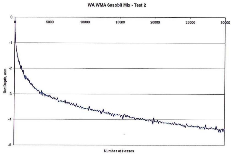
Figure A4: Hamburg Wheel Track Test Results of Washington WMA Sasobit Mix Test 2
