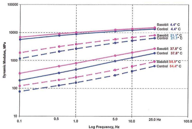
Figure 3: Dynamic Modulus, |E^*|
