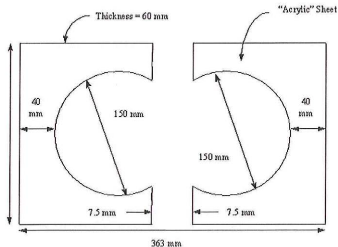
Figure 8: Test Specimen Configuration for the Hamburg Wheel-Tracking Device
