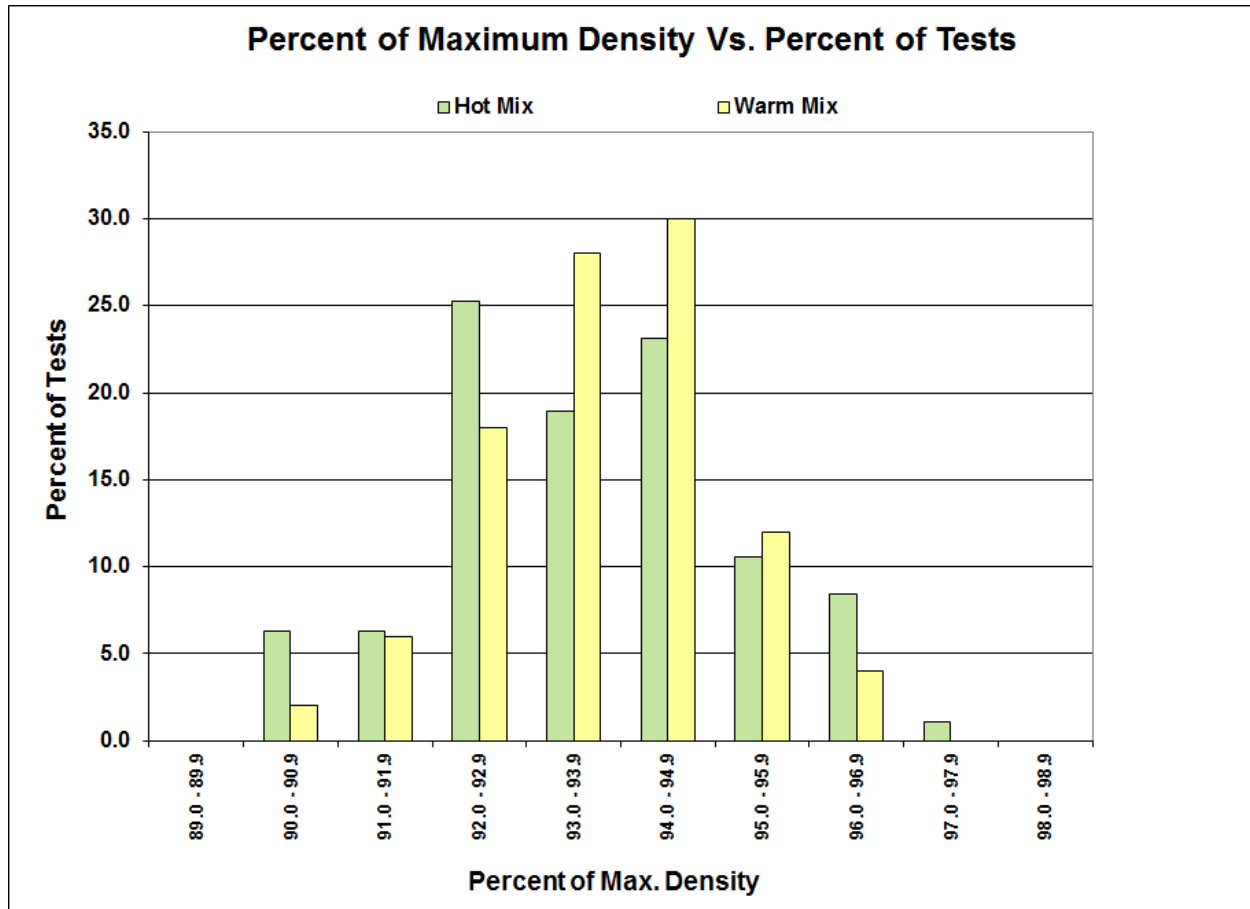
Figure 22. Distribution of compaction test results.
