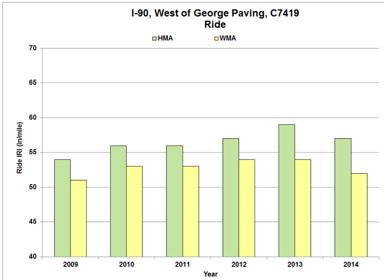
Figure 25. Ride measurements.
