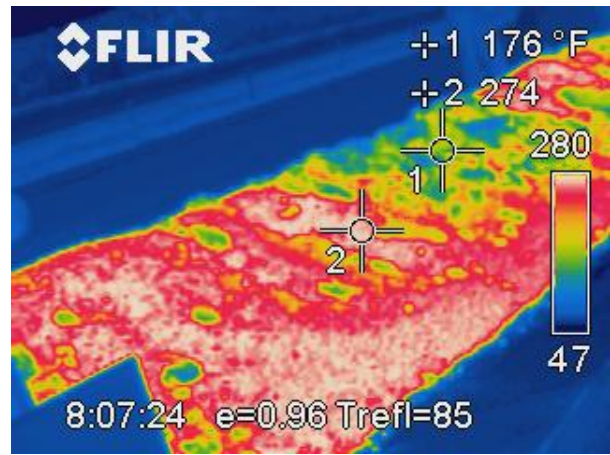
Figure 16. Cool WMA in windrow.
