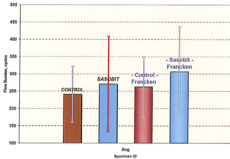
Figure 4: Flow Number, F_n
