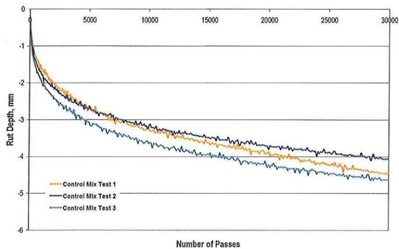
Figure 9: Hamburg Wheel Track Test Results of HMA Control Mix
