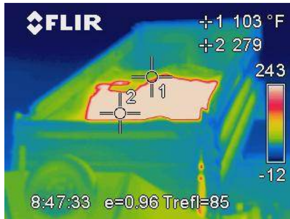
Figure 17. Thermal image of first load of WMA as it is being dumped into windrow device.
