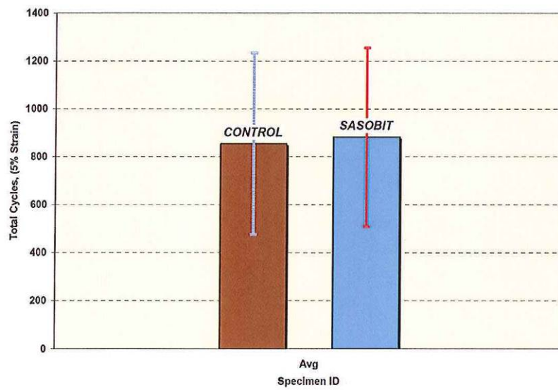
Figure 6: Total cycles at 5% Strain
