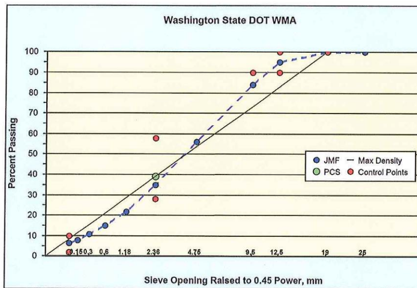
Figure 1: .45 power chart Warm Mix/Control JMF
