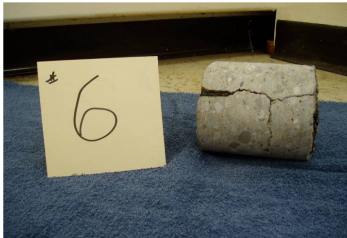
Figure 11. Side view showing panel joint and cracks. 8/04
