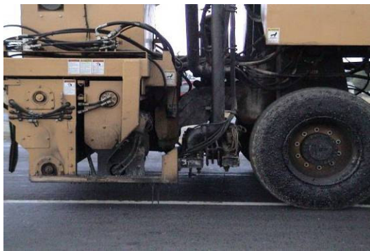
Image C. Paving machine showing spray bar for binder in the center of the photo. Aggregate is spread from the box behind the spray bar.
