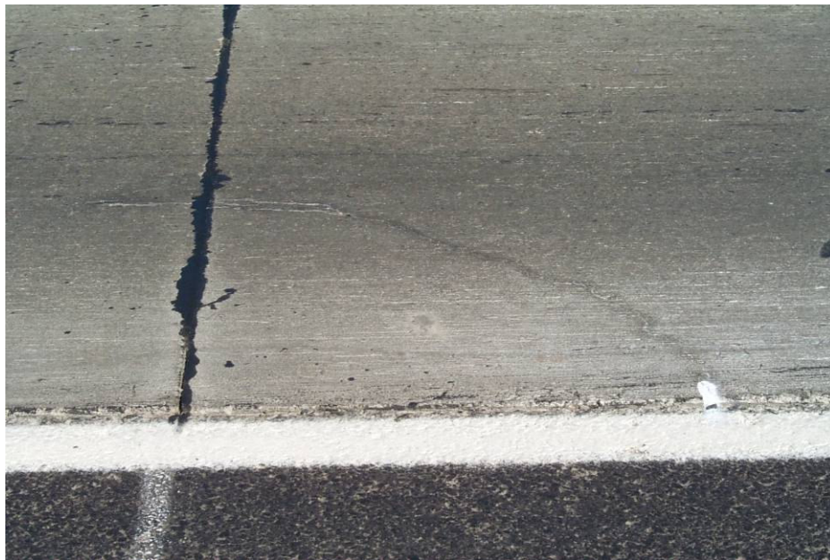
Image 5. Typical corner crack within the 3-inch ultra thin whitetopping test section.
