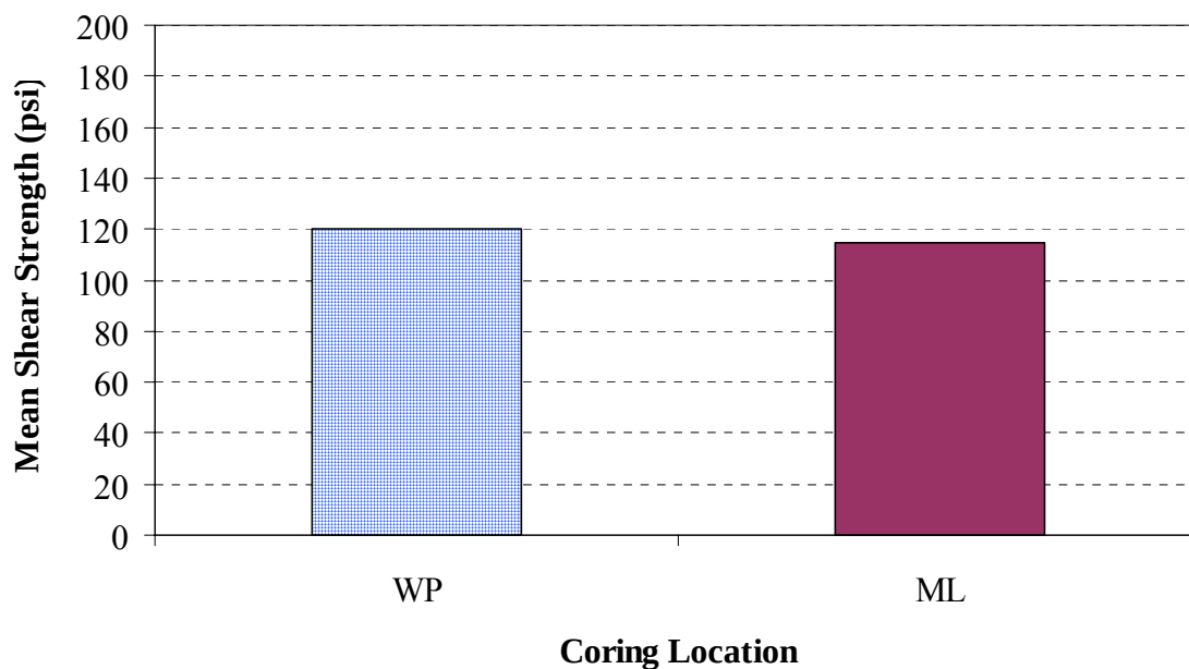
Figure 4.4: Effect of coring Location on the FDOT shear strength (factor insignificant).
