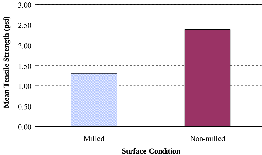
Figure 4.8: Effect of Surface Condition on the UTEP Pull-Off tensile strength.
