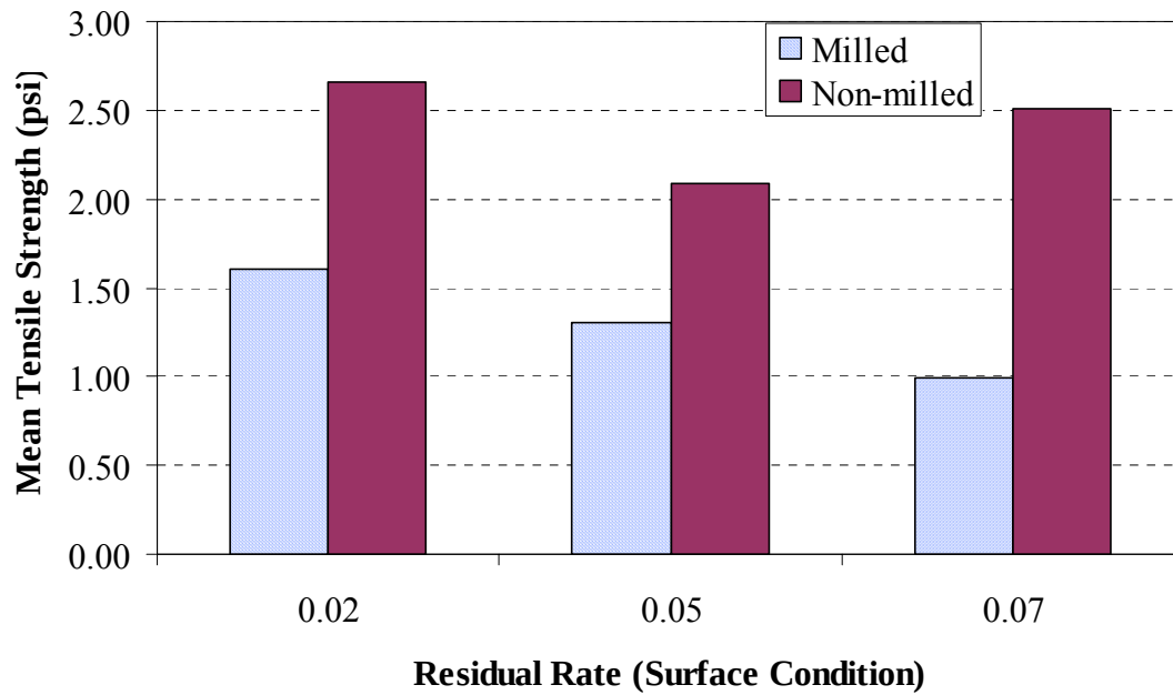
Figure 4.10: Effect of Residual Rate nested within Surface Condition on the UTEP Pull-Off tensile strength (factor insignificant).
