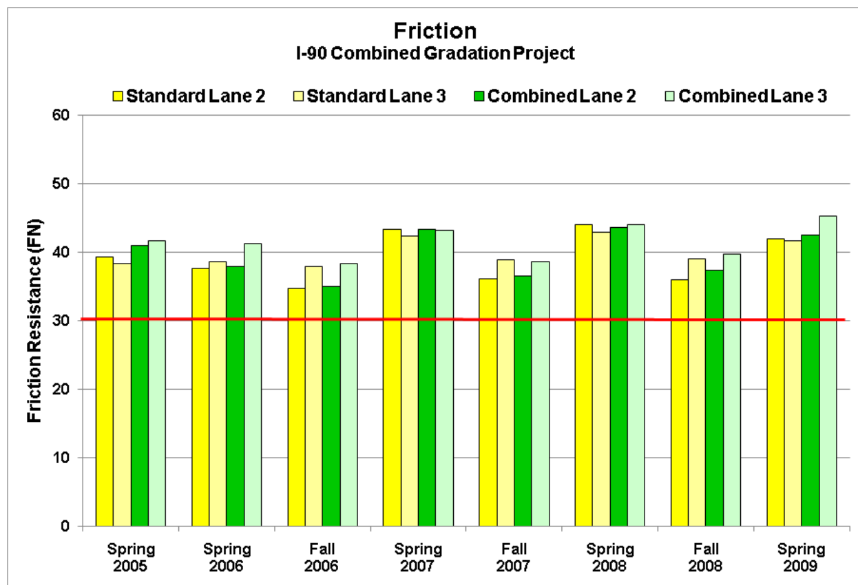
Figure 21. Friction resistance data for the I-90 Combined Gradation Project.
