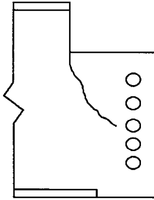
Figure 19. Specimen 0A Cracking
