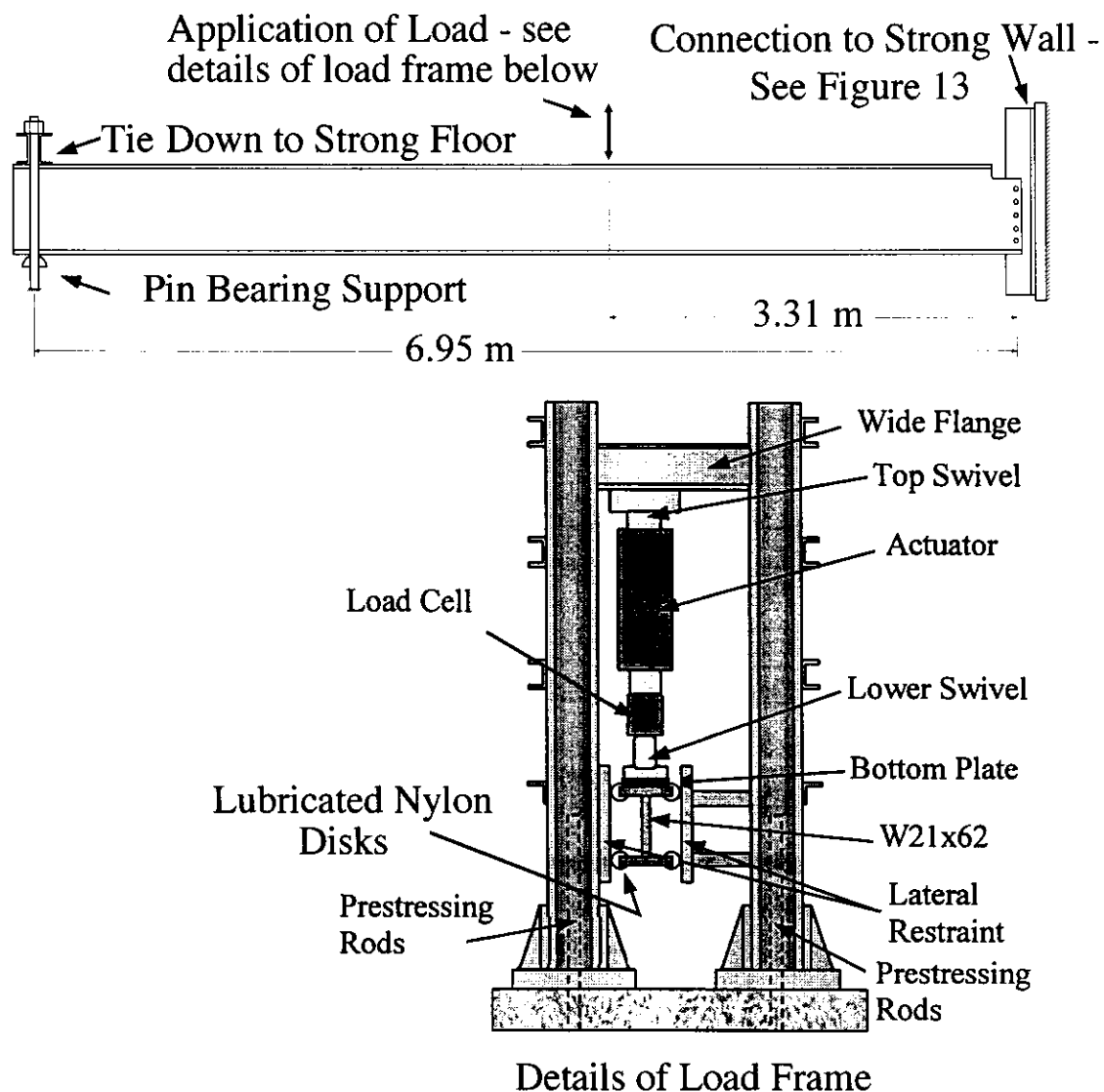
Figure 12. Test Set-Up
