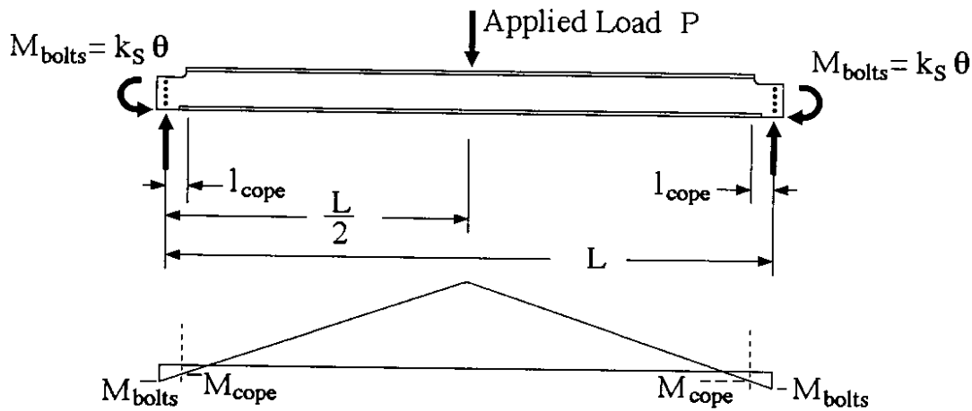
Figure 29. Geometry and Moment Diagram for Internal Stringer
