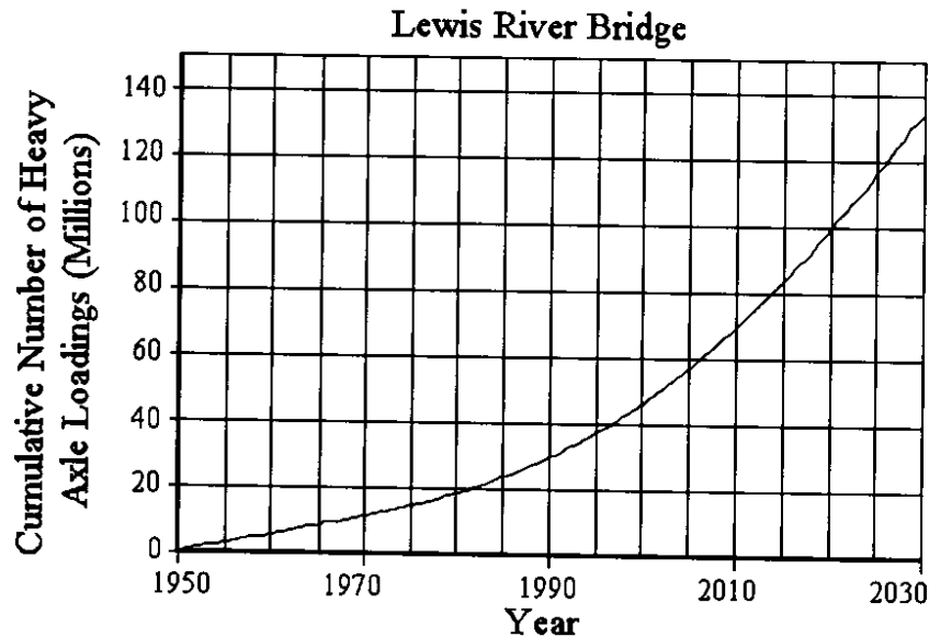
Figure 35. Cumulative Number of Heavy Axle Loadings vs. Time
