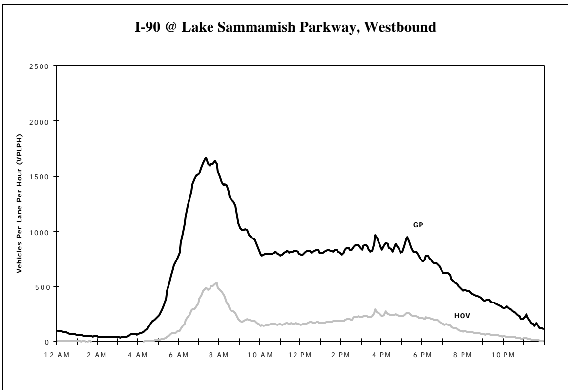
Figure 2-26. Average Weekday GP and HOV Volume Profile (1998): I-90 @ Lake Sammamish Parkway
