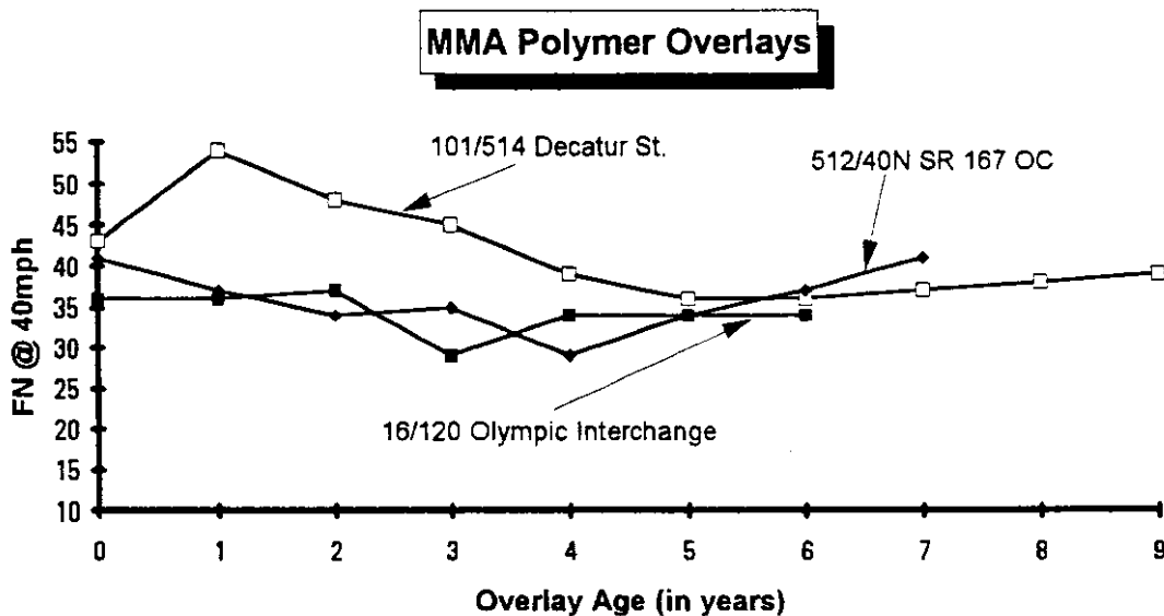
FIGURE 17 Friction Number vs. Polymer Overlay Age.
