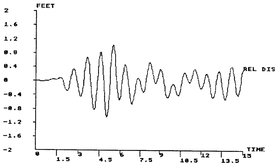
Figure C.2 Transverse Bridge and Ground Nodal Displacements and Relative Transverse Displacement, Lake Hughes Earthquake, Section 2 Sixty-Four-Span Model
