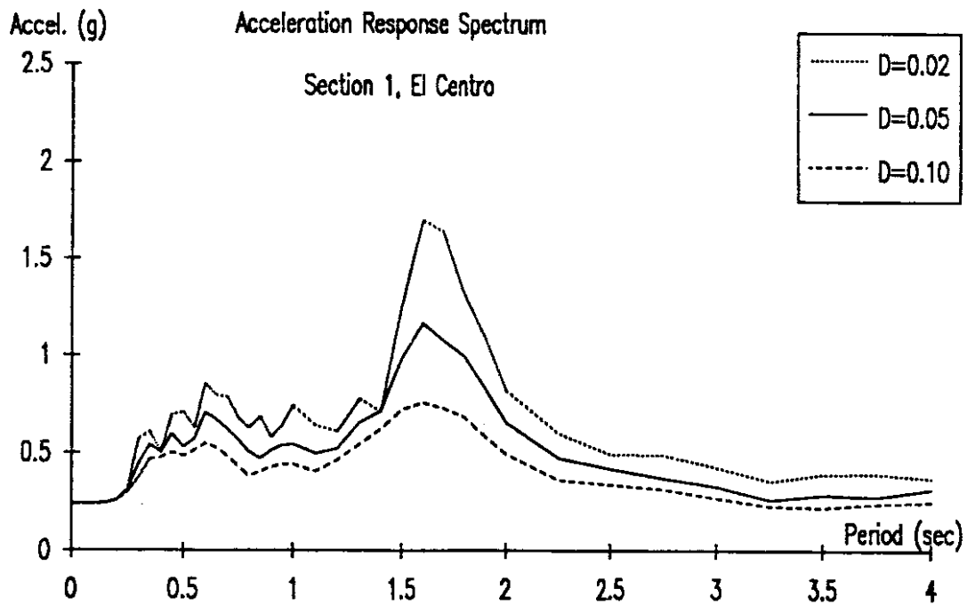
Figure A.6 Acceleration Time-History and Response Spectra for El Centro Earthquake, Section 1 Soil Profile
