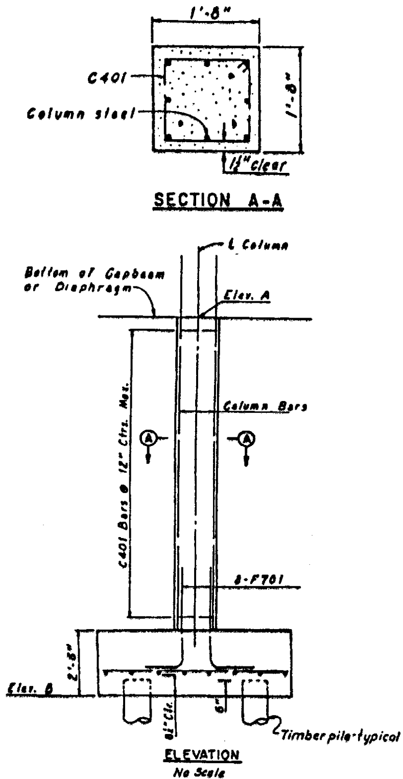
Figure 6. Typical Column Cross-section and Elevation
