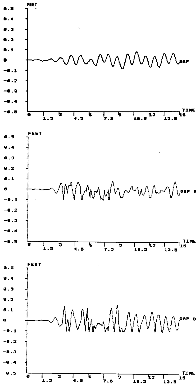
Figure F.4 Relative Longitudinal Gap Displacement for Simple Joint Model (GAP) and Nonlinear Joint Model (GAP A and GAP B), Section 3-4
