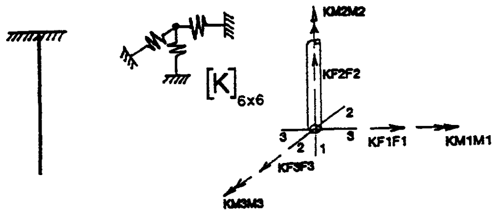
Seisab Pile Model
