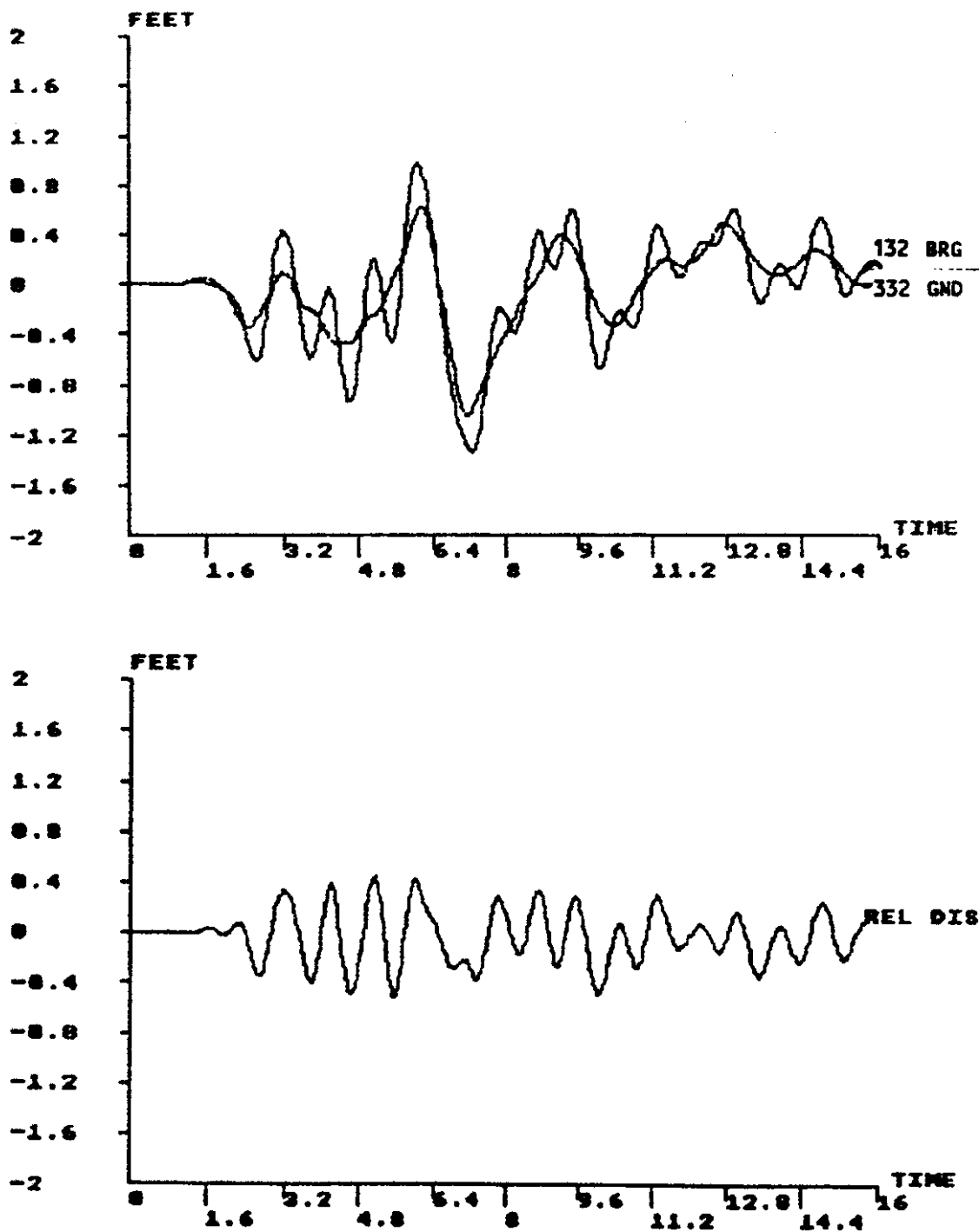
Figure D.5 Transverse Bridge and Ground Nodal Displacements and Relative Transverse Displacement, Lake Hughes Earthquake, Section 5 Sixty-Four-Span Model, Time-Delayed Input
