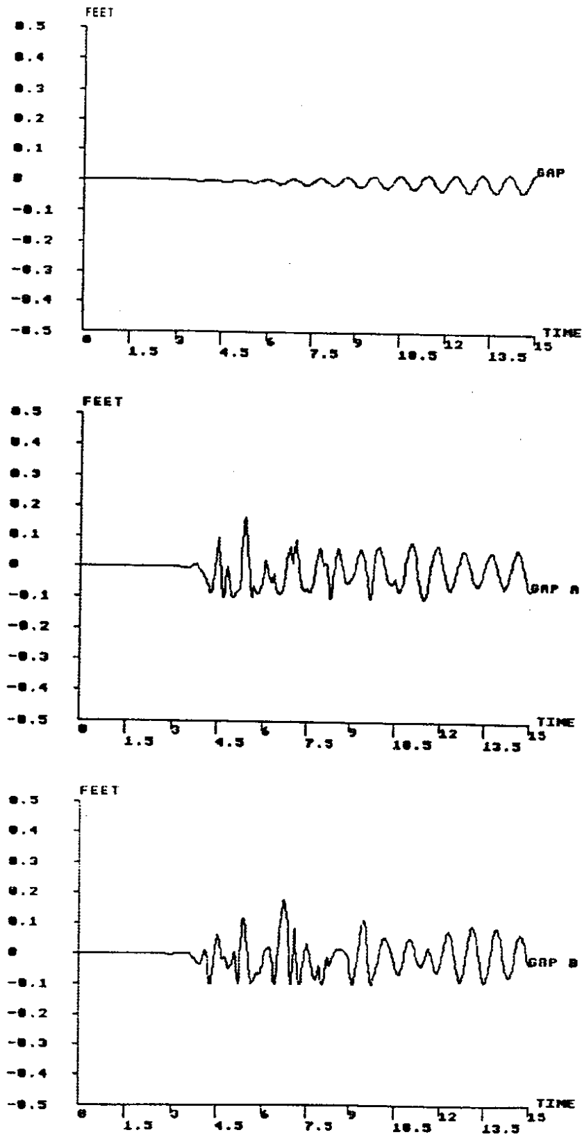
Figure F.3 Relative Longitudinal Gap Displacement for Simple Joint Model (GAP) and Nonlinear Joint Model (GAP A and GAP B), Section 3
