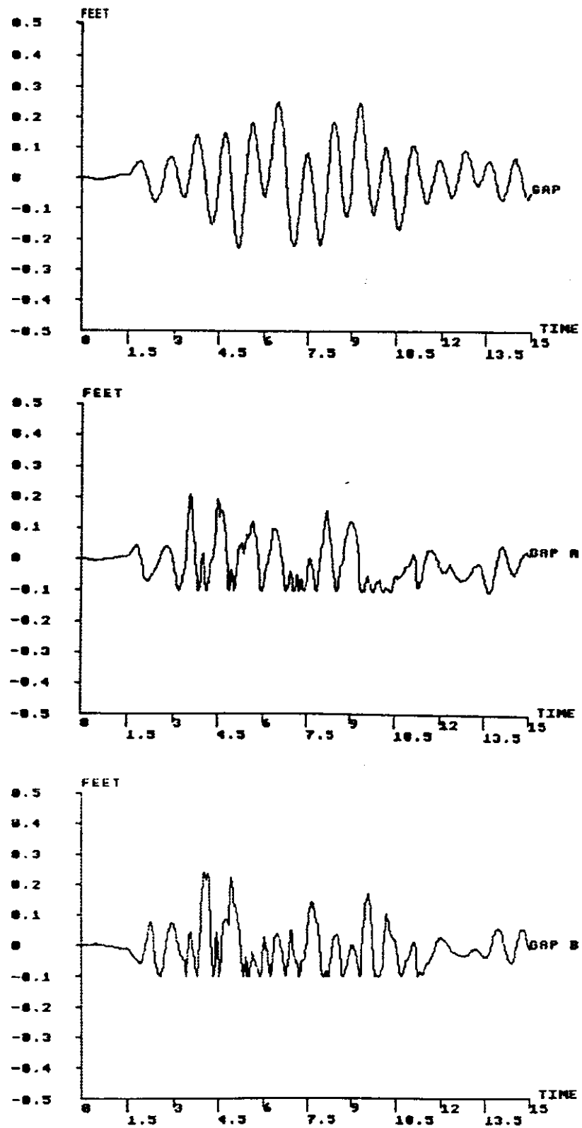
Figure F.1 Relative Longitudinal Gap Displacement for Simple Joint Model (GAP) and Nonlinear Joint Model (GAP A and GAP B), Section 1-2
