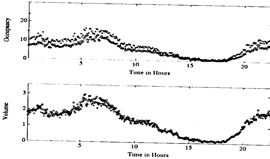
Figure 4.5: Occupancy and volume as a function of time.
