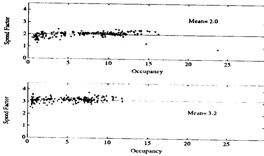
Figure 4.8: Cross correlation coefficient as a function of occupancy.
