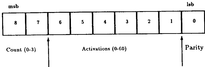
Figure 3.1: TSMC data byte bit format.
