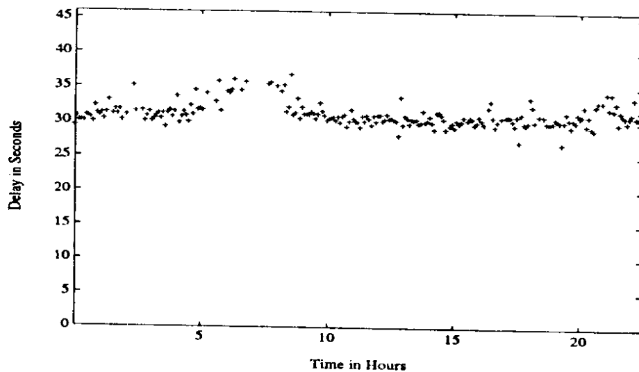
Figure 4.2: Delay verses time.
