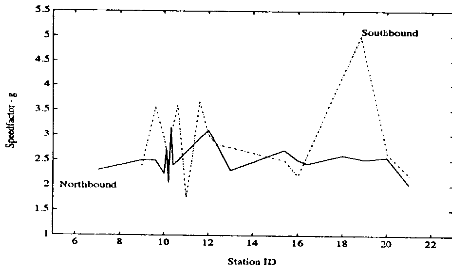
Figure 4.9: Estimated mean speed factor ( g ) as a function of location.
