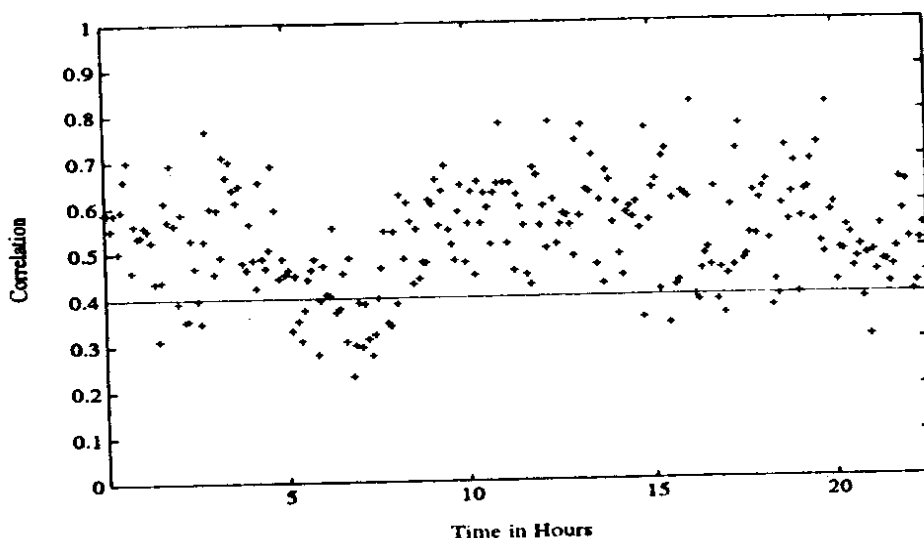
Figure 4.3: Maximum value in the cross correlation coefficient function.
