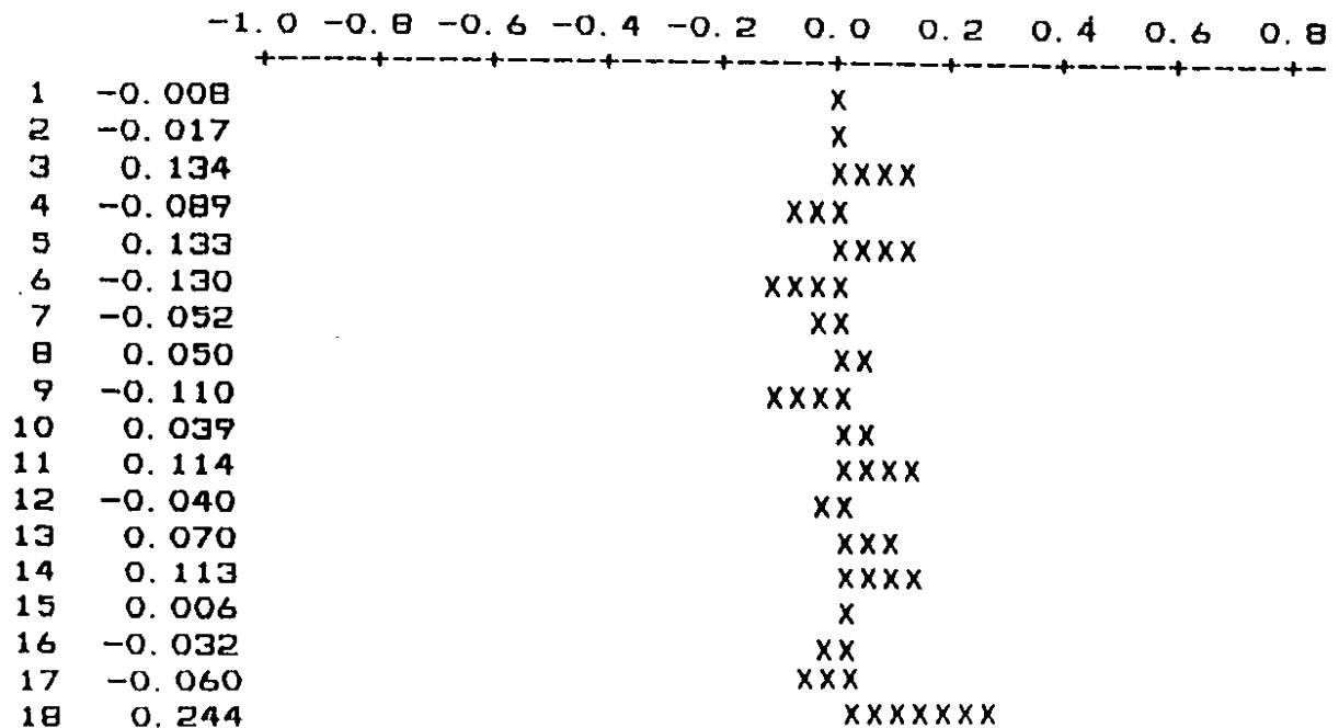
FIGURE 2.2 AUTOCORRELATION PLOT
