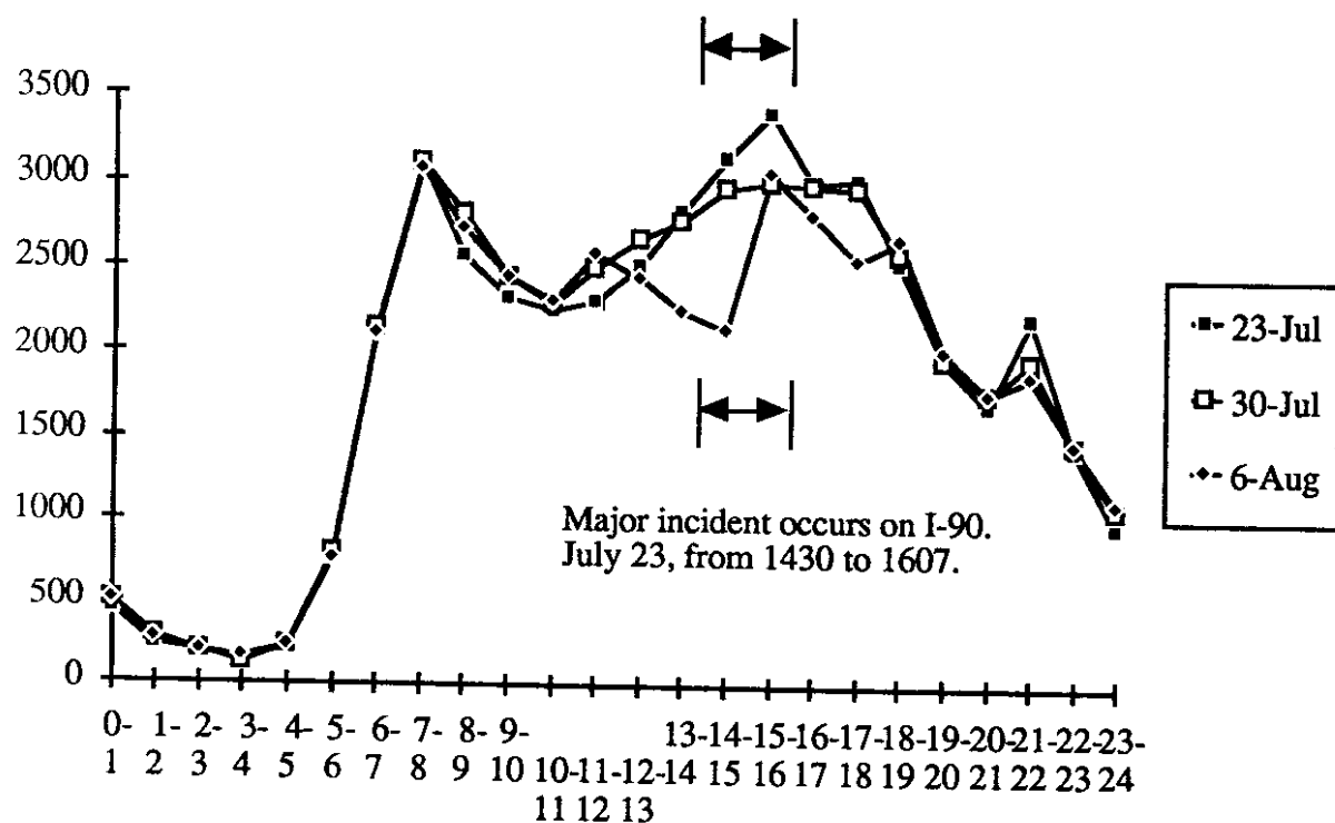
Figure 16. Eastbound Traffic Volumes on SR-520 at 10th
