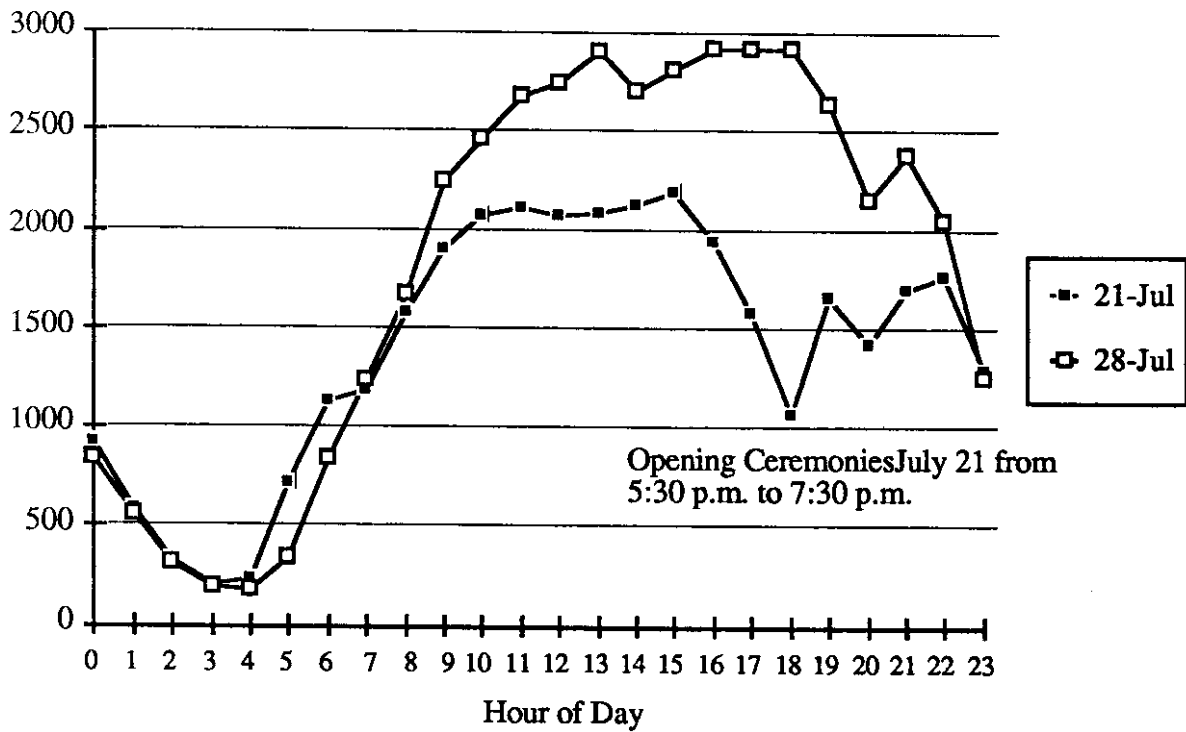
Figure 9. Westbound SR-520 Traffic Volumes
