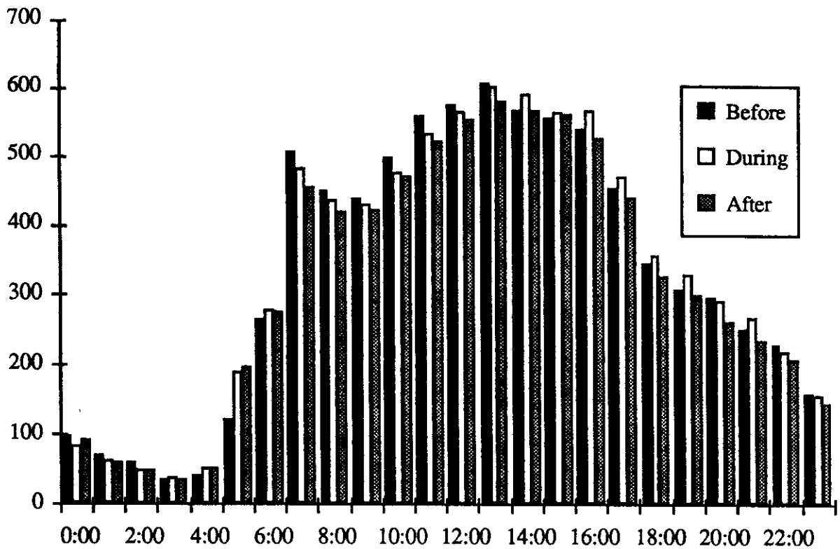
Figure 7. Weekday Average Hourly Traffic Volumes Before, During and After the Goodwill Games - SR-509 Northbound at Union Station
