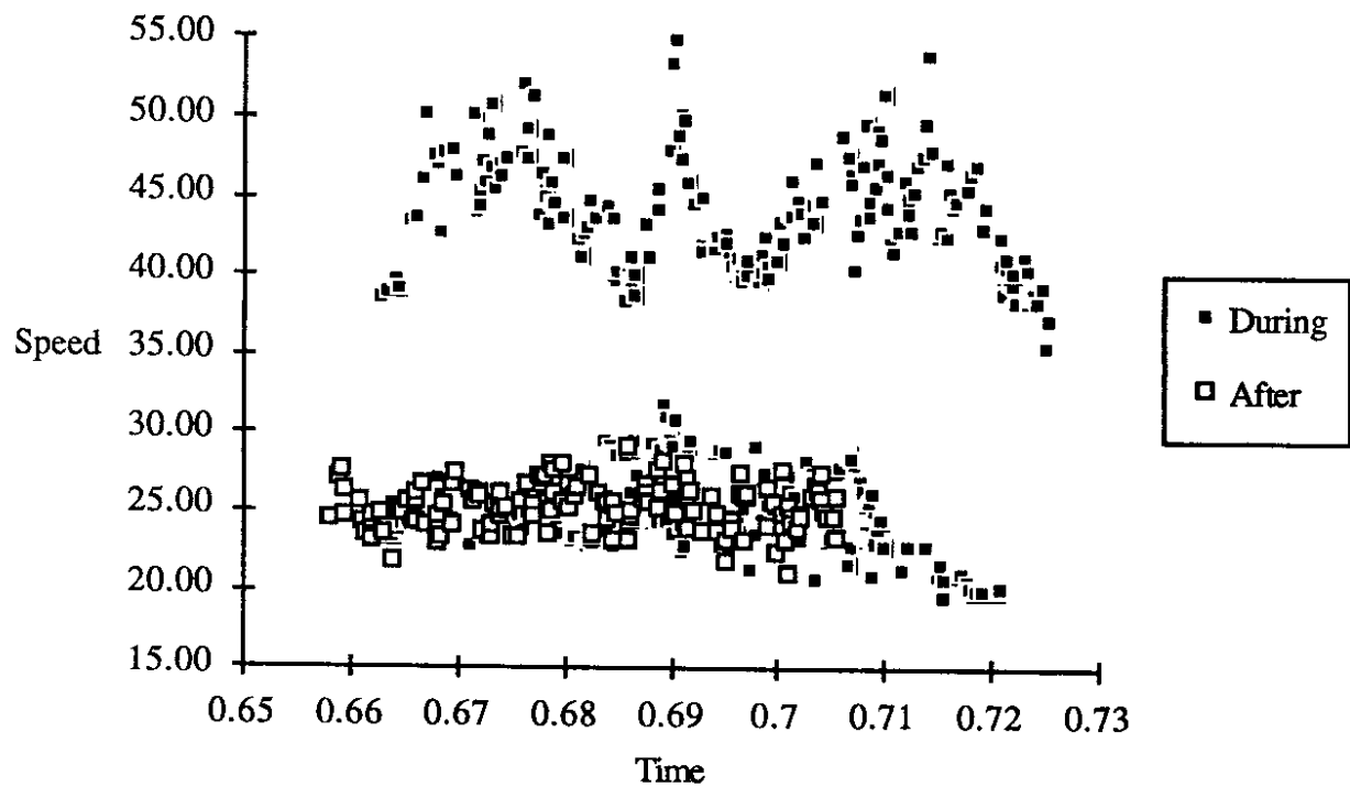
Figure 27. Vehicle Speeds Eastbound on SR-520 From Montlake to the Old Toll Plaza
