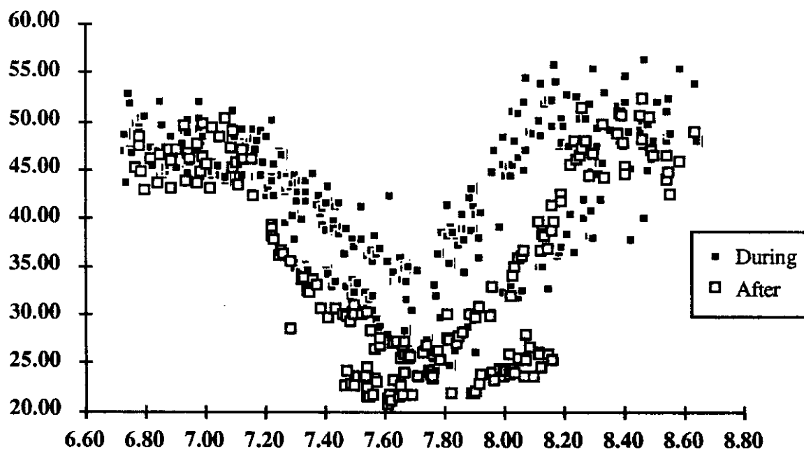
Figure ix. During and After Vehicle Speeds on WB SR-520 in the AM Commute Period
