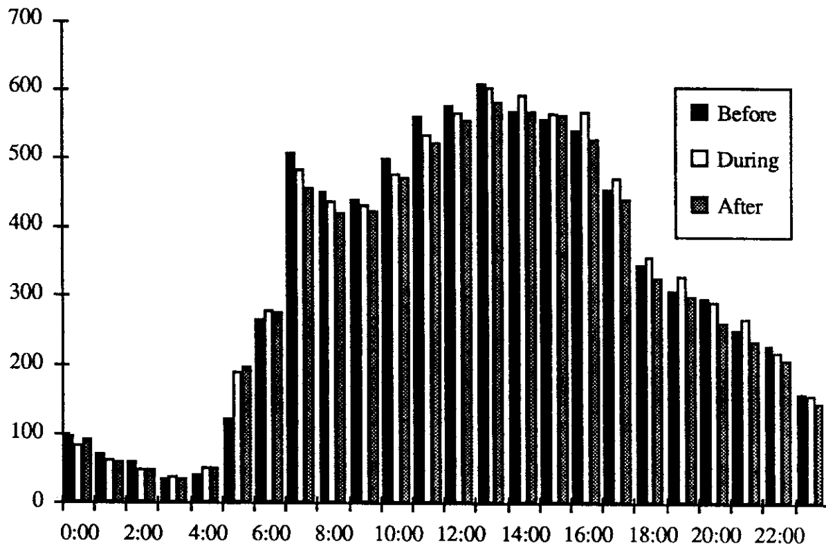
Figure ii. Weekday Average Hourly Traffic Volumes Before, During and After the Goodwill Games - SR-509 Northbound at Union Station
