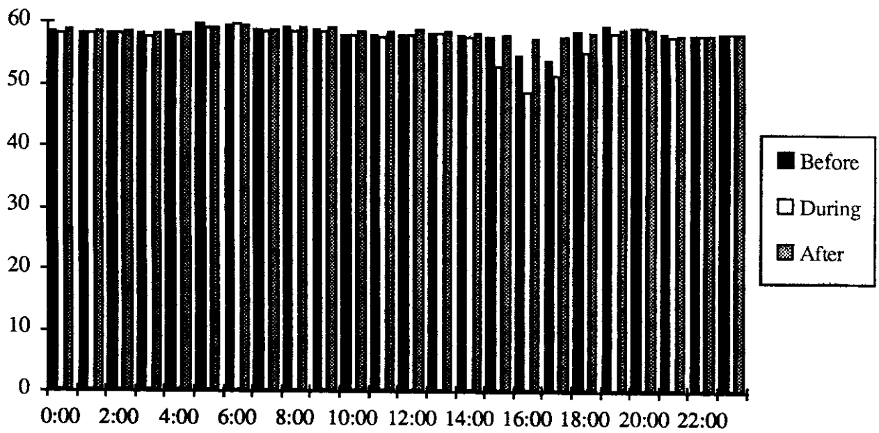
Figure vii. Weekday Hourly Traffic Speeds Before, During and After the Goodwill Games — Interstate 5, Southbound at Fife
