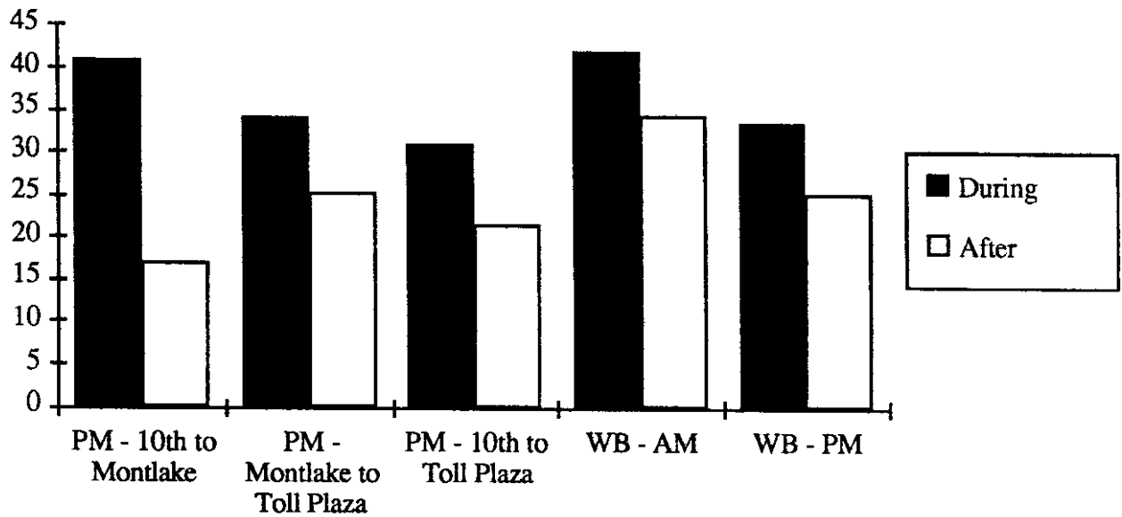
Figure viii. Average Speeds Before and After the Goodwill Games on SR-520
