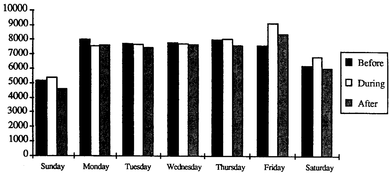
Figure 6. Daily Traffic Volumes by Day of Week - Before, During and After the Goodwill Games SR-509, Northbound at Union Station in Tacoma
