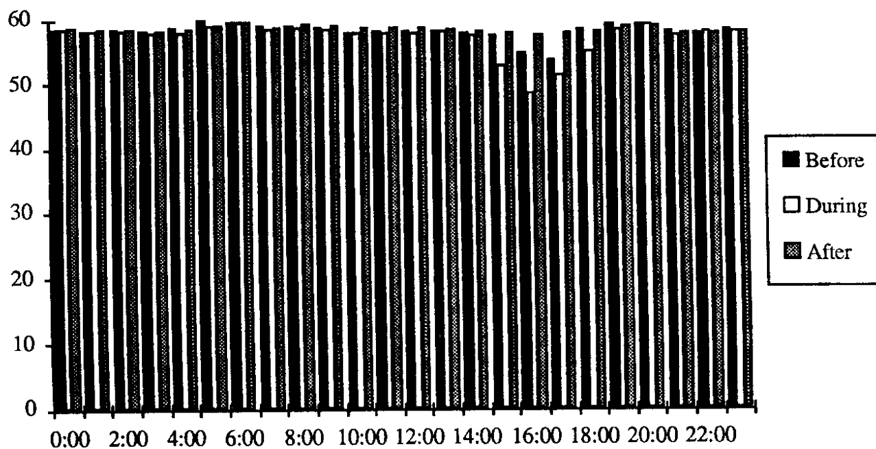
Figure 19. Weekday Hourly Traffic Speeds Before, During and After the Goodwill Games - Interstate 5, Southbound at Fife
