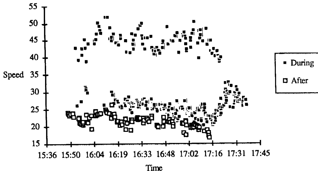
Figure 28. Eastbound Traffic Speeds on SR-520 From 10th to the Toll Plaza During and After the Goodwill Games
