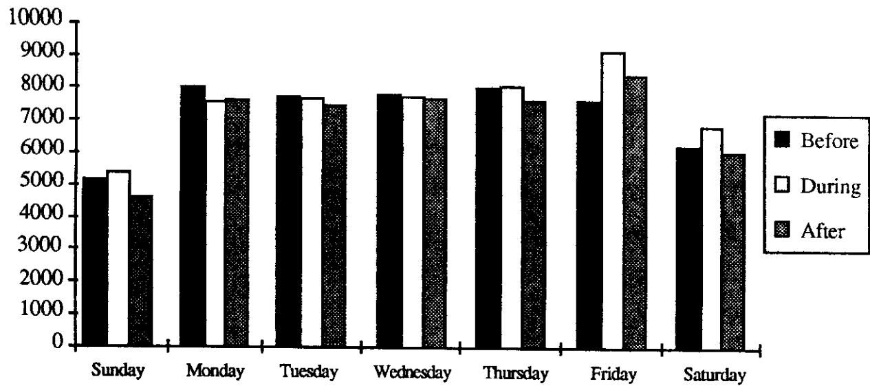
Figure i. Daily Traffic Volumes by Day of Week - Before, During and After the Goodwill Games SR-509, Northbound at Union Station in Tacoma
