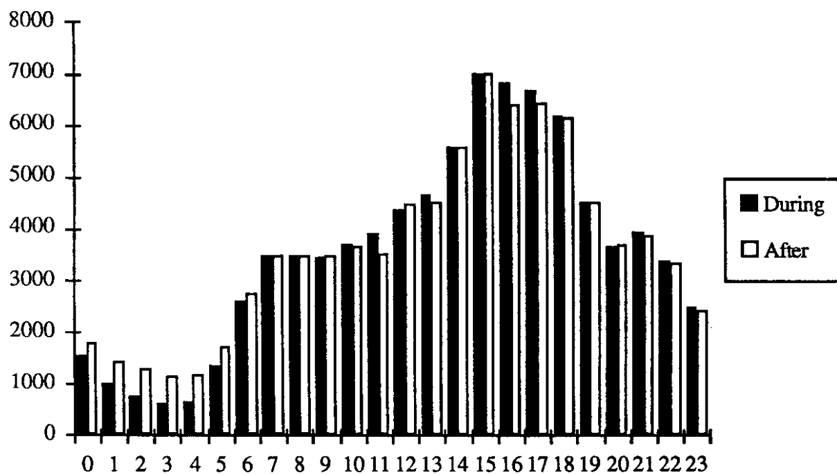
Figure 15. Northbound Traffic Volumes on I-5 at NE 107th Street
