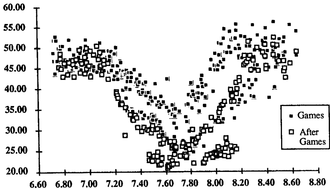
Figure 24. During and After Vehicle Speeds On WB SR-520 in the AM Commute Period
