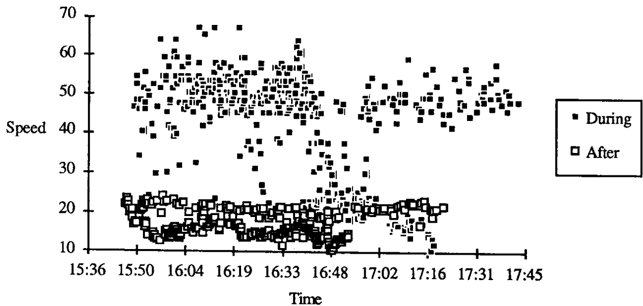
Figure 26. Eastbound Traffic Speeds On Sr-520 From 10th to Montlake During and After the Goodwill Games
