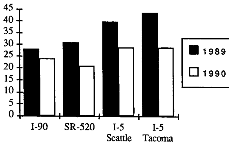
Figure 33. Duration of Tow Truck Involved Incidents
