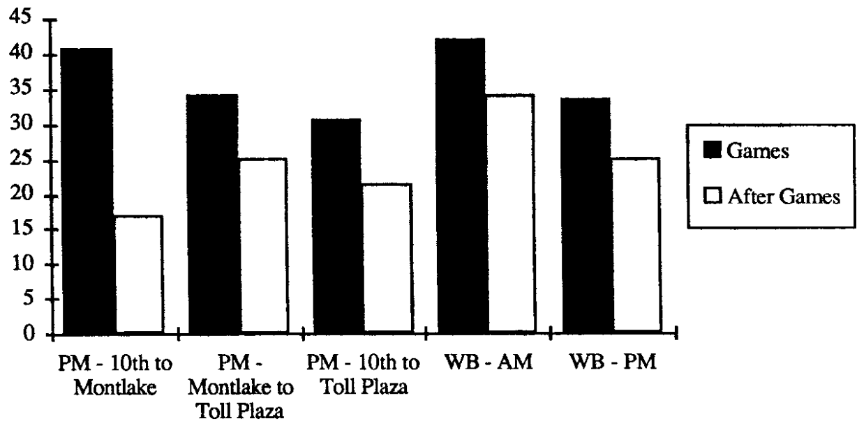
Figure 22. Average Speeds Before and After The Goodwill Games on SR-520
