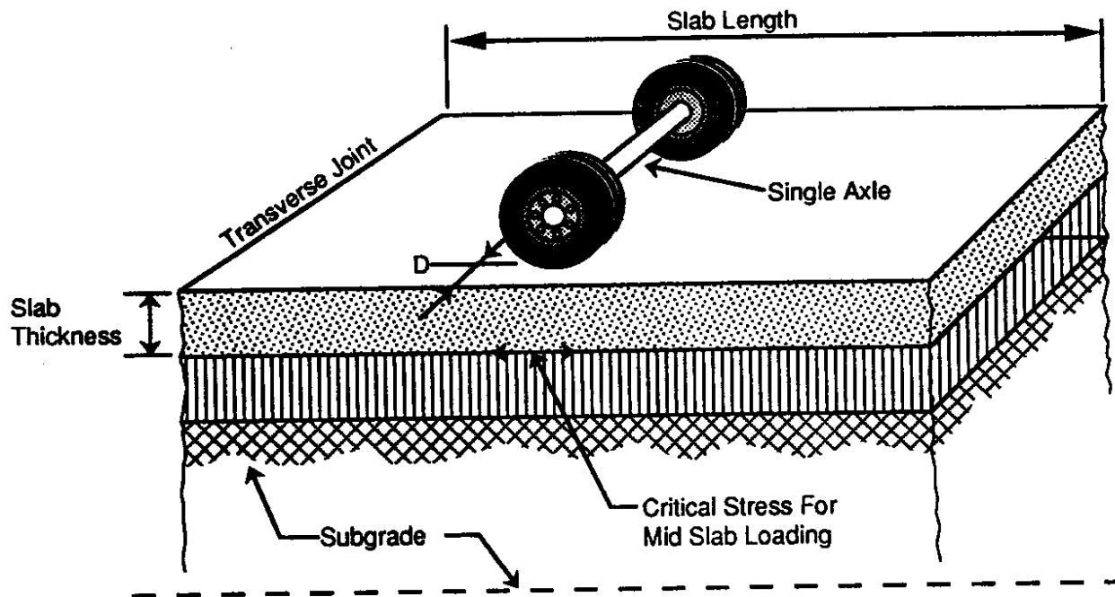
Figure 4.1 Critical Fatigue Damage Location and Tensile Stress Direction for Mid-Slab Loading
