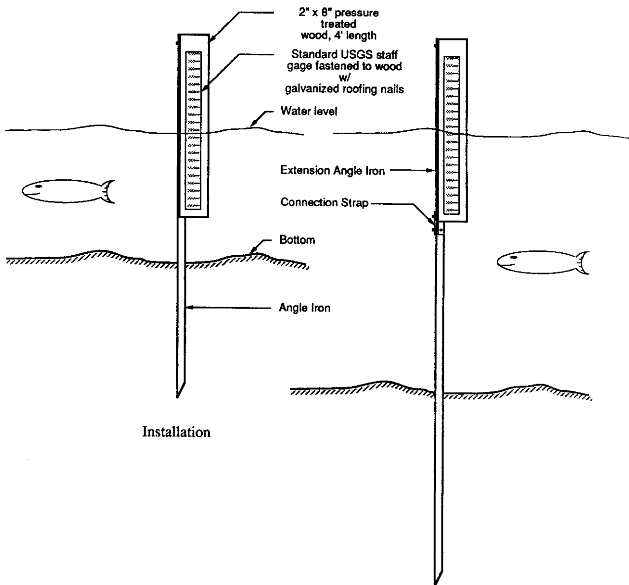
Alternative Installation Using Extension Angle Iron (for relatively deep water or loose soil)
