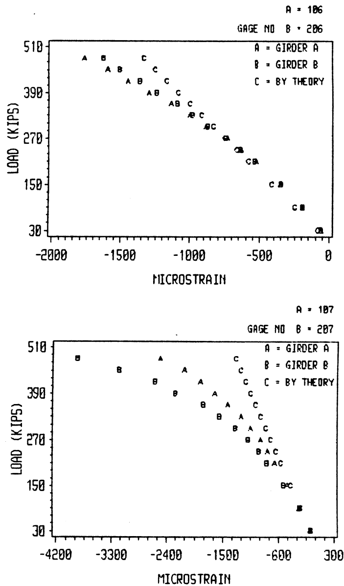
Figure 7.16 Laboratory Test - Comparison of Experimental and Theoretical Results: Gages 106, 206, 107, and 207
