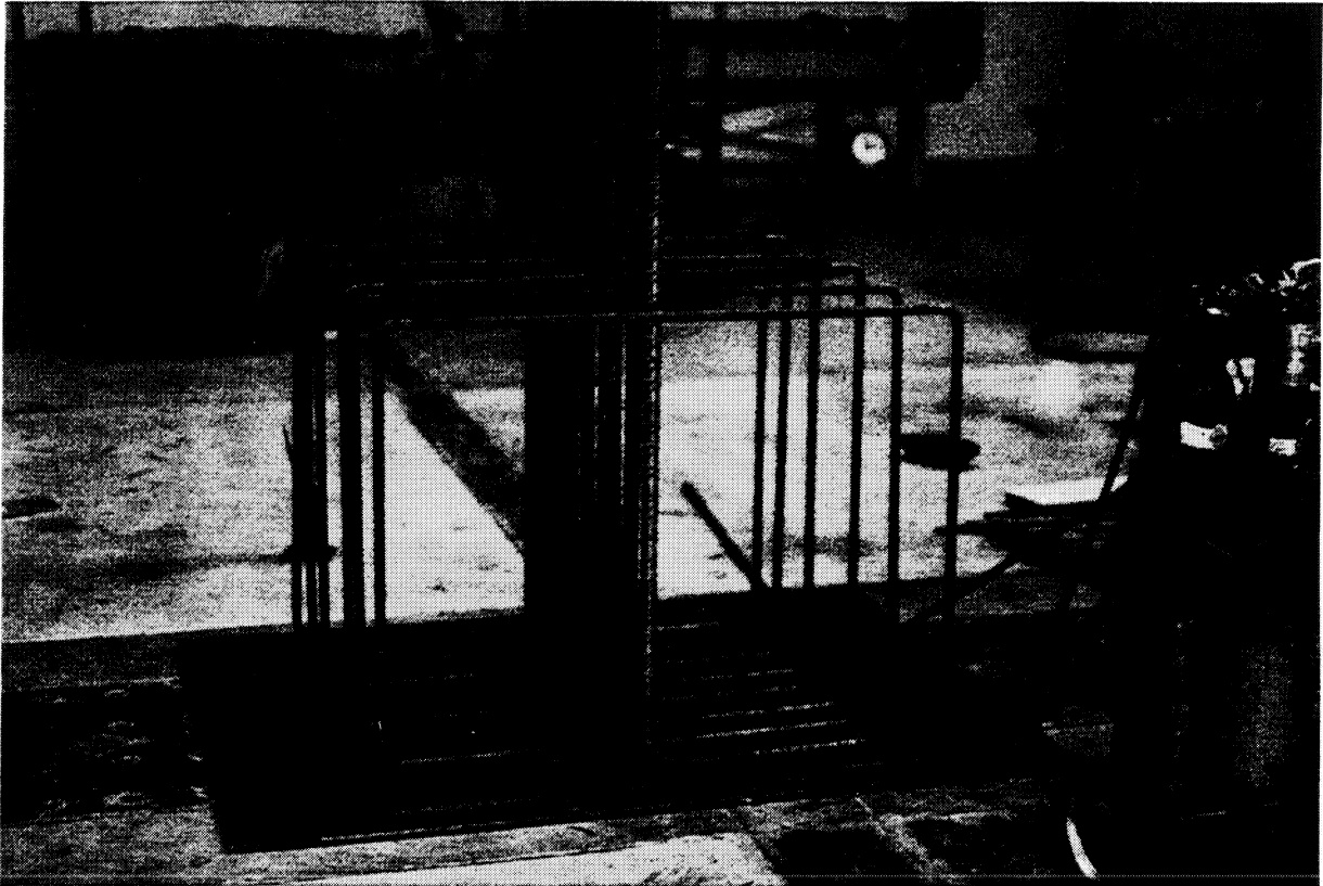
Figure 6.8 Laboratory Test - Reinforcement in the Pedestal and the Hinge Bars
