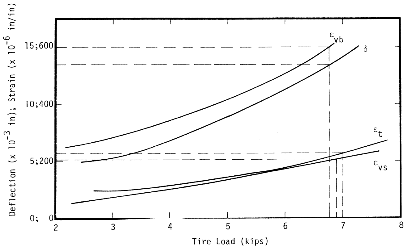
Figure D11. SR 2, Sunnyslope - Tire Size 11-22.5.
