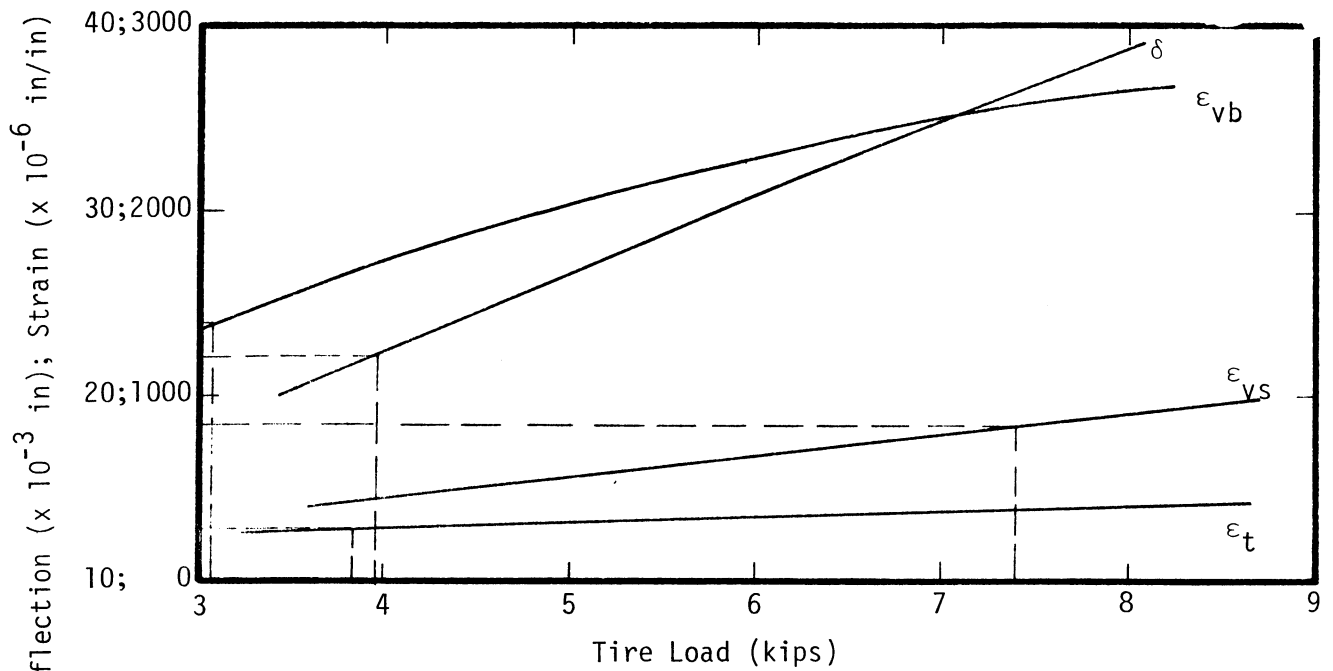
Figure D48. SR 172, MP 21.4 - Tire Size 12-24.5, Tire Pressure 95 psi.
