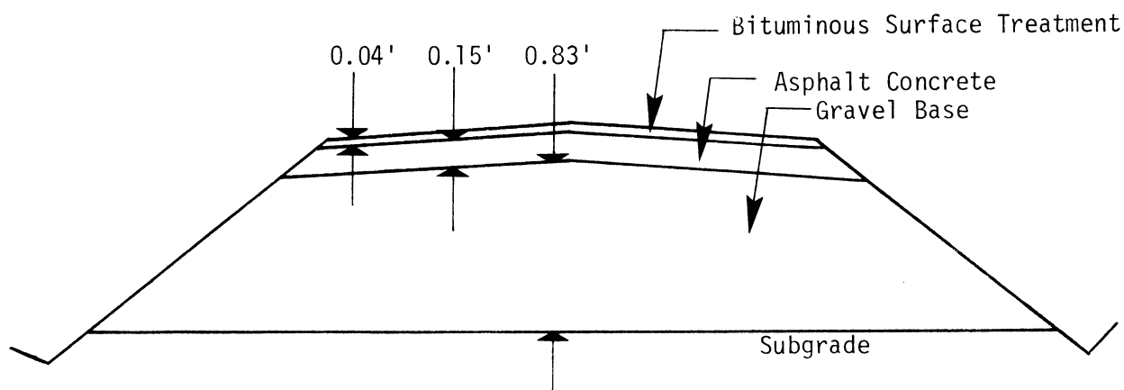
Figure 6. SR 174, MP 2.3-2.0 - Cross Section
