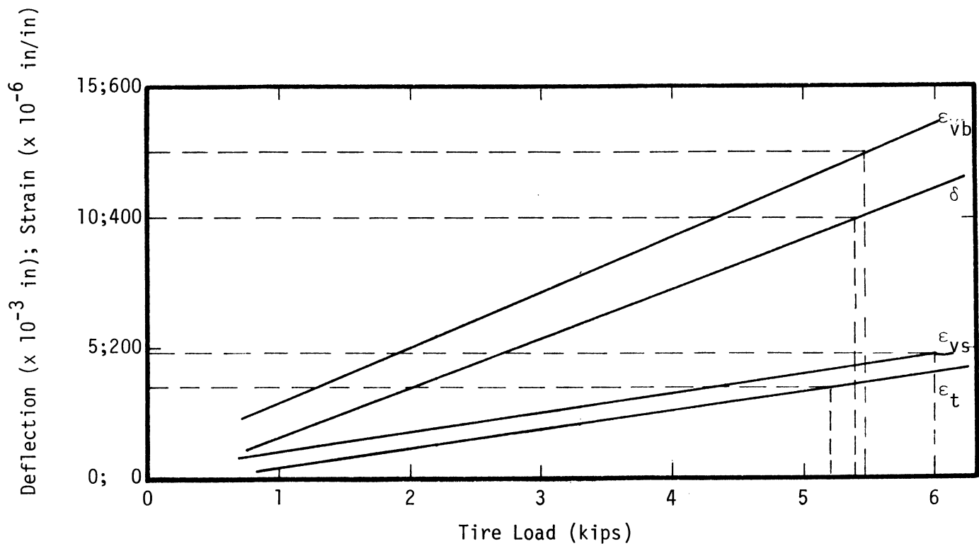
Figure D8. SR 2, Sunnyslope - Tire Size 8-22.5.
