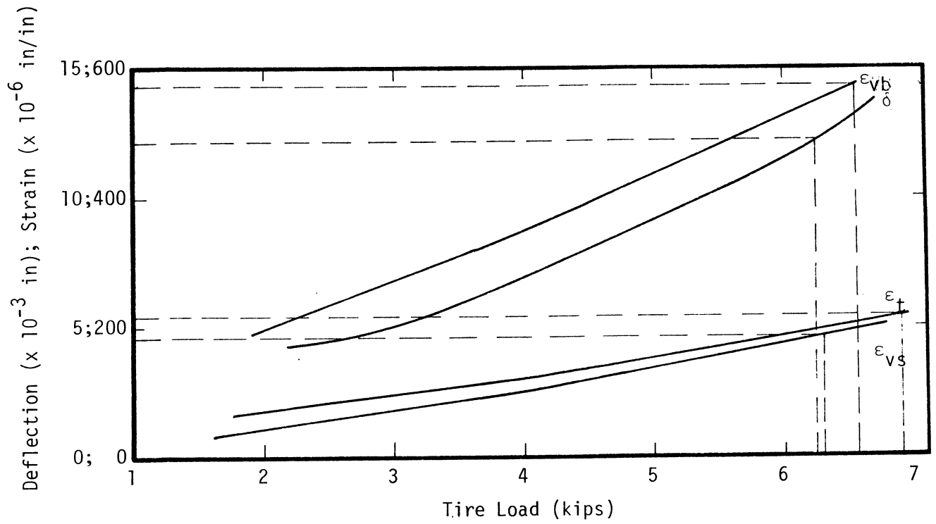
Figure D10. SR 2, Sunnyslope - Tire Size 10-22.5.
