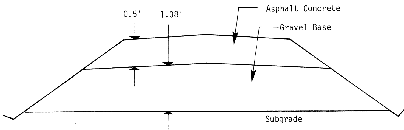
Figure 7. SR 2, MP 117.38-117.52 (Sunnyslope) - Cross Section.
