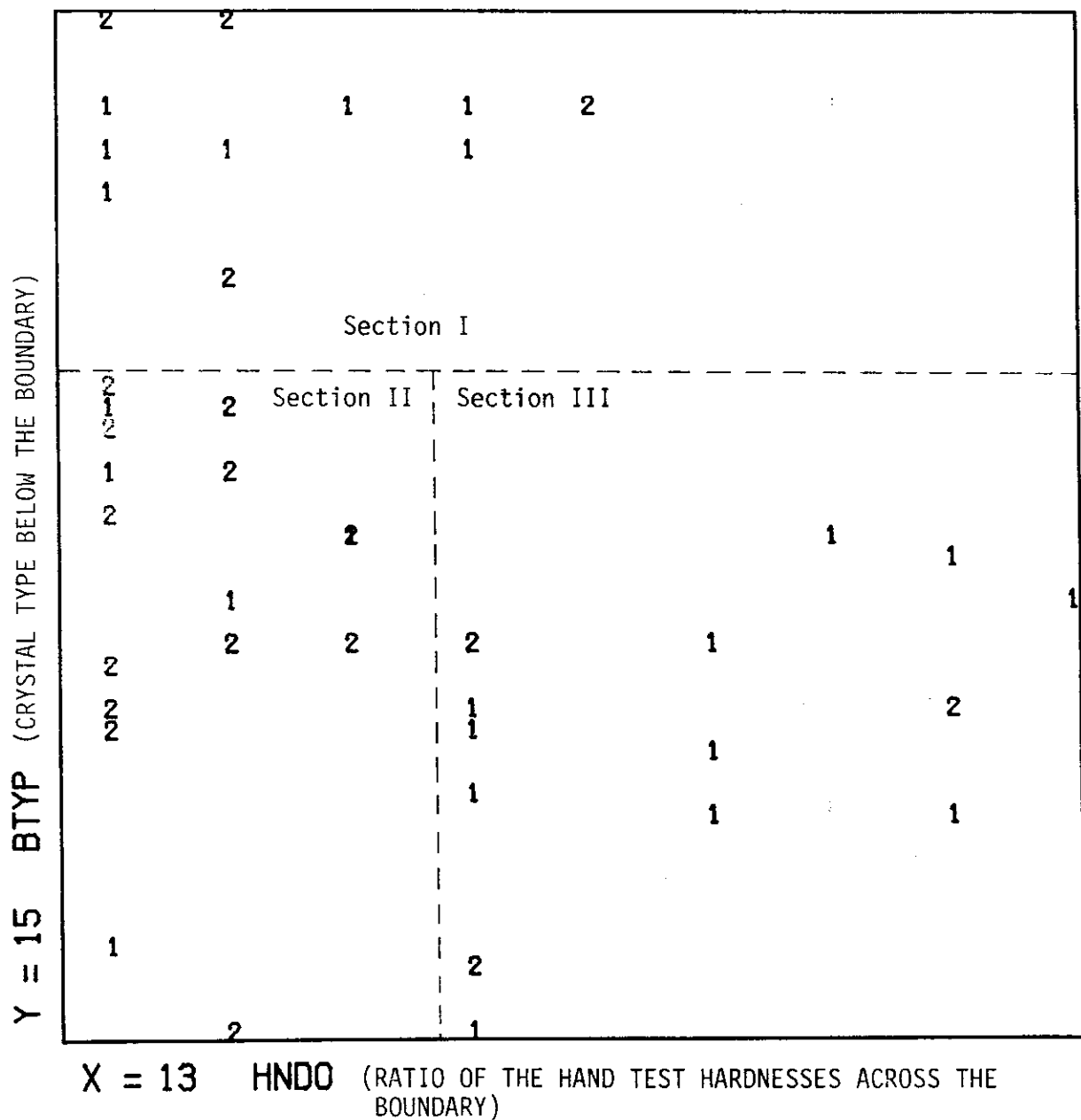
FIGURE 5.10 Crystal type of the snow layer below the boundary vs. the ratio of hand test hardnesses across the boundary (irrespective of direction). Dashed lines divide the plot into three arbitrary regions containing clusters of bed surface boundaries (1) and stable layer boundaries (2).
