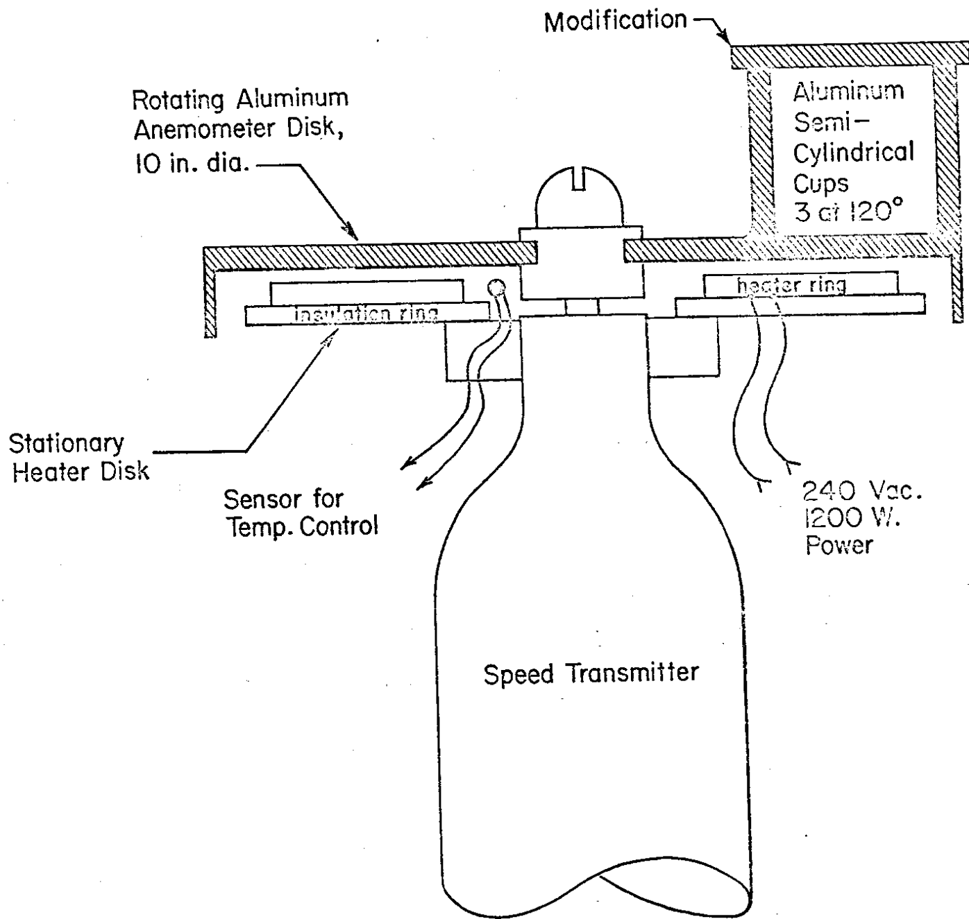
FIGURE 10.1 Wind speed sensor.
