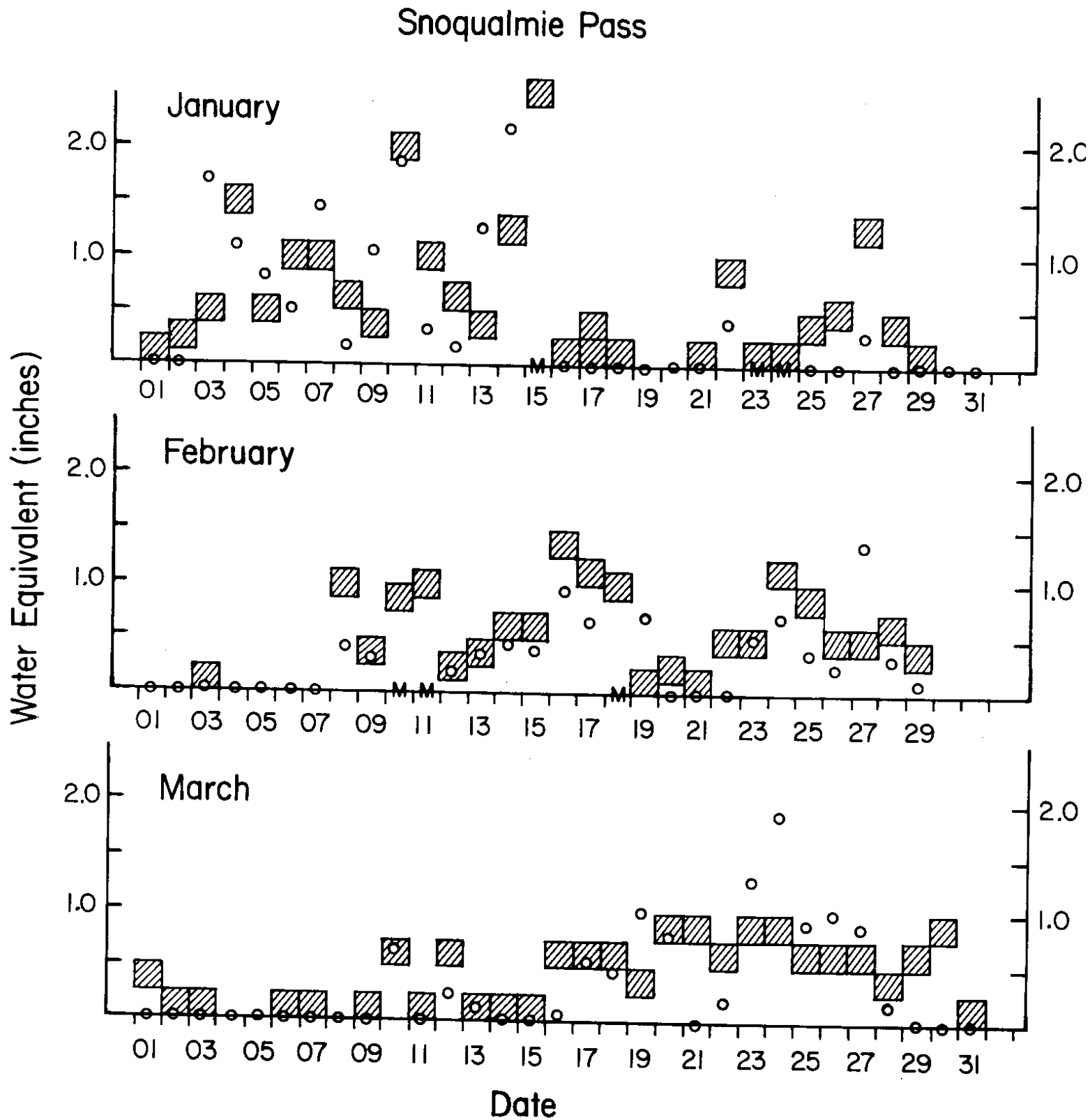
Figure 12. Forecast and observed 24-hour water equivalents for Snoqualmie Pass. (Shaded box indicates forecast ranges; no box indicates 0" water equivalent forecast; 0 indicates measured water equivalent; M indicates missing data.)
