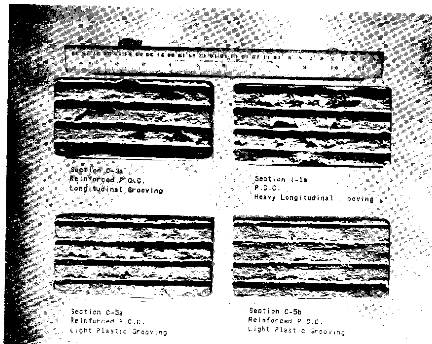
Figure 8: Plaster castings of P.C.C. surface textures showing the different types of longitudinal grooving.
