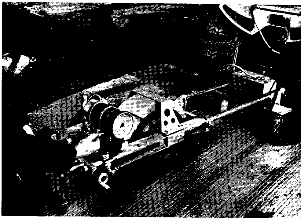
Figure 18: A view of the California Skid Tester being used on a grooved section of P.C.C. Note the tractor as the source of power and braking device.
