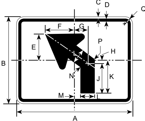
DIMENSIONS (MILLIMETERS)
