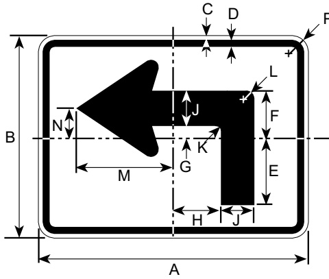
DIMENSIONS (MILLIMETERS)
