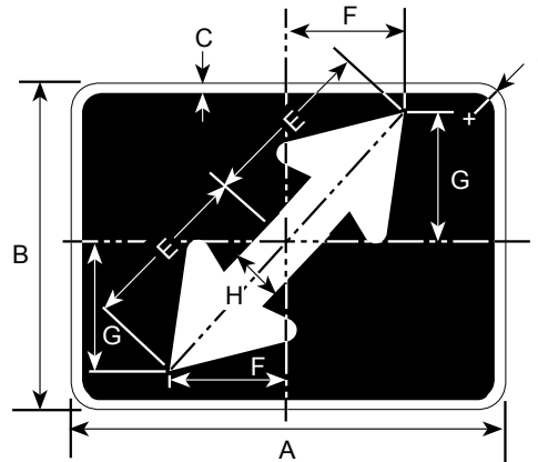
DIMENSIONS (MILLIMETERS)
