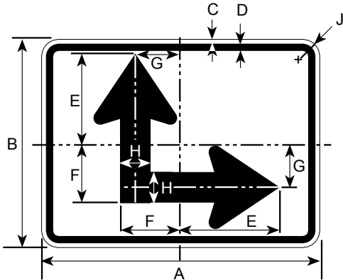
DIMENSIONS (MILLIMETERS)
