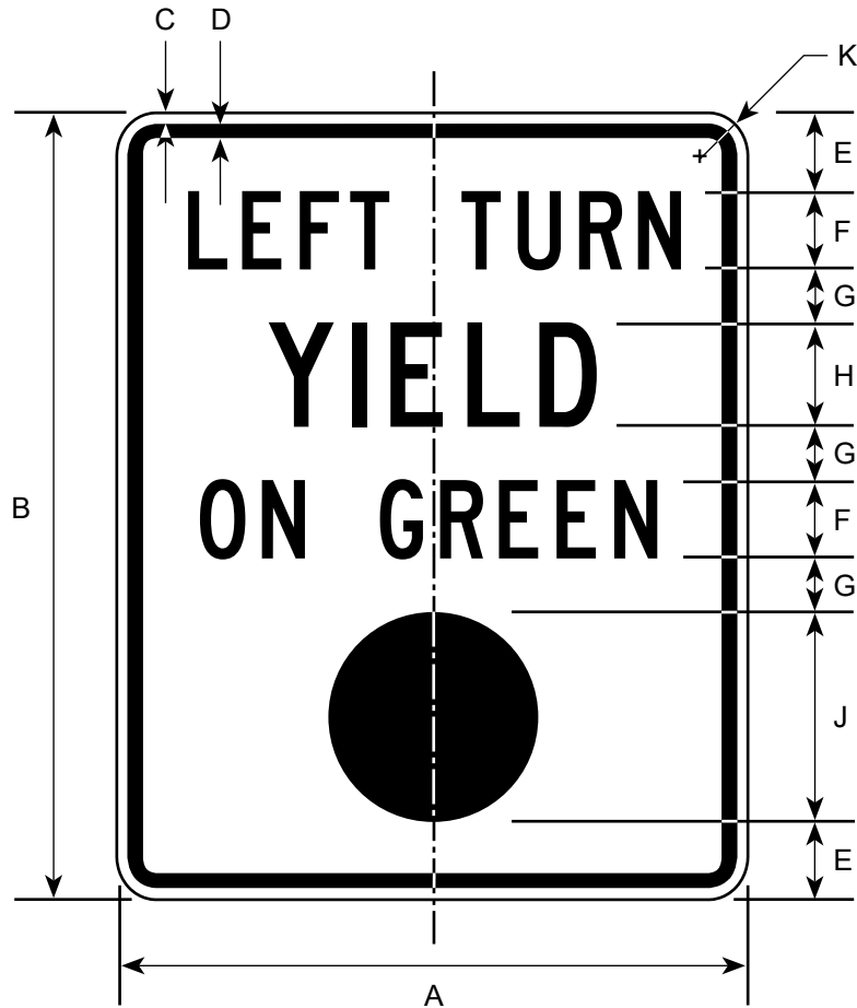
DIMENSIONS (MILLIMETERS)
