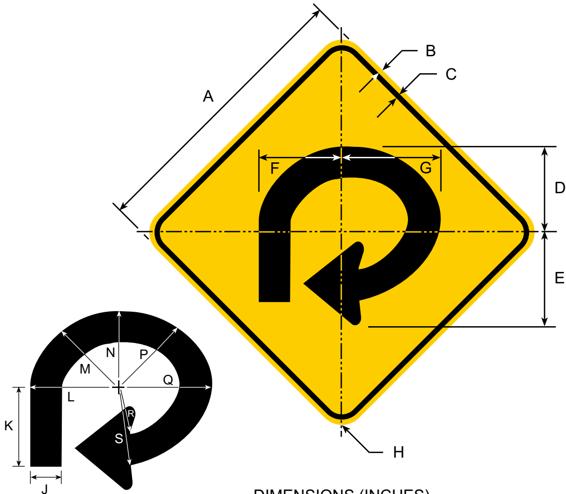
DIMENSIONS (INCHES)
