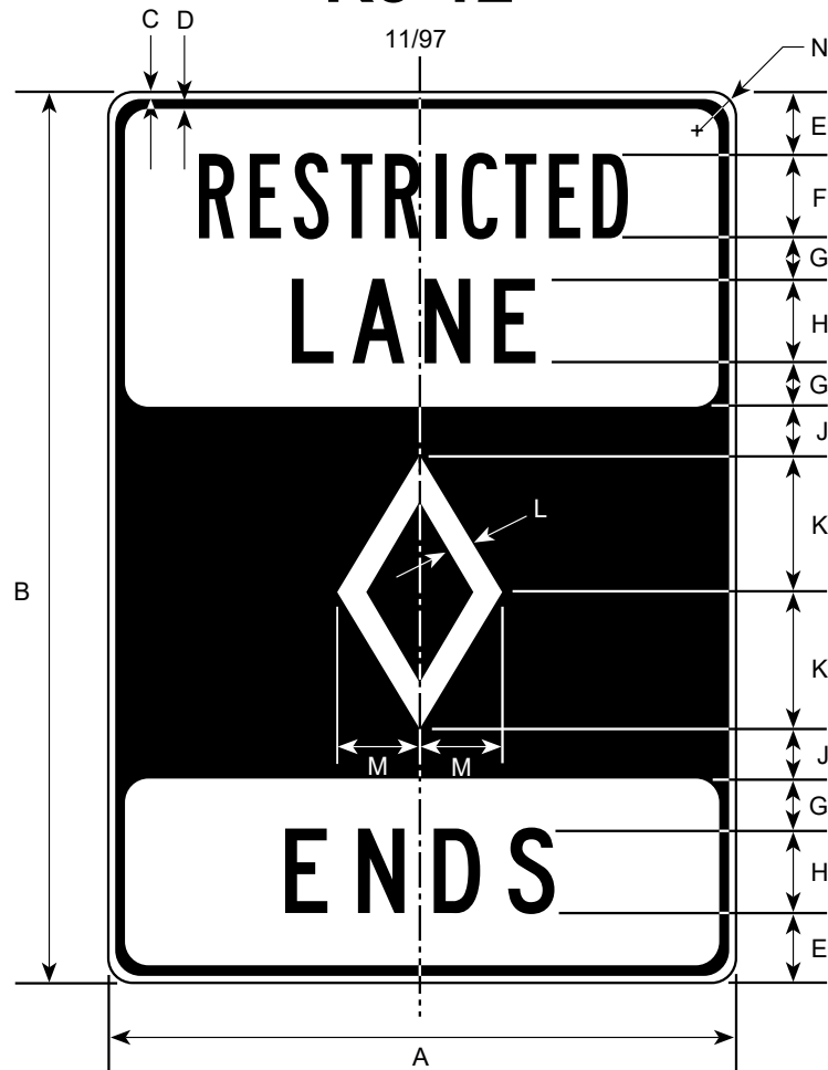
DIMENSIONS (MILLIMETERS)
