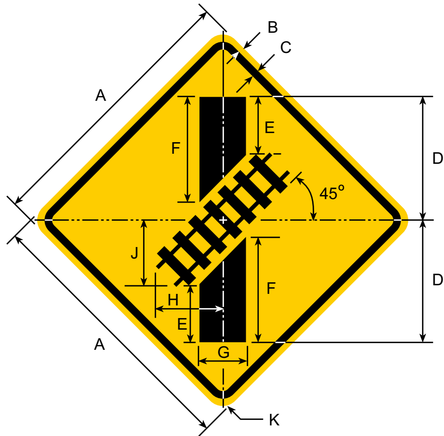
DIMENSIONS (MILLIMETERS)
