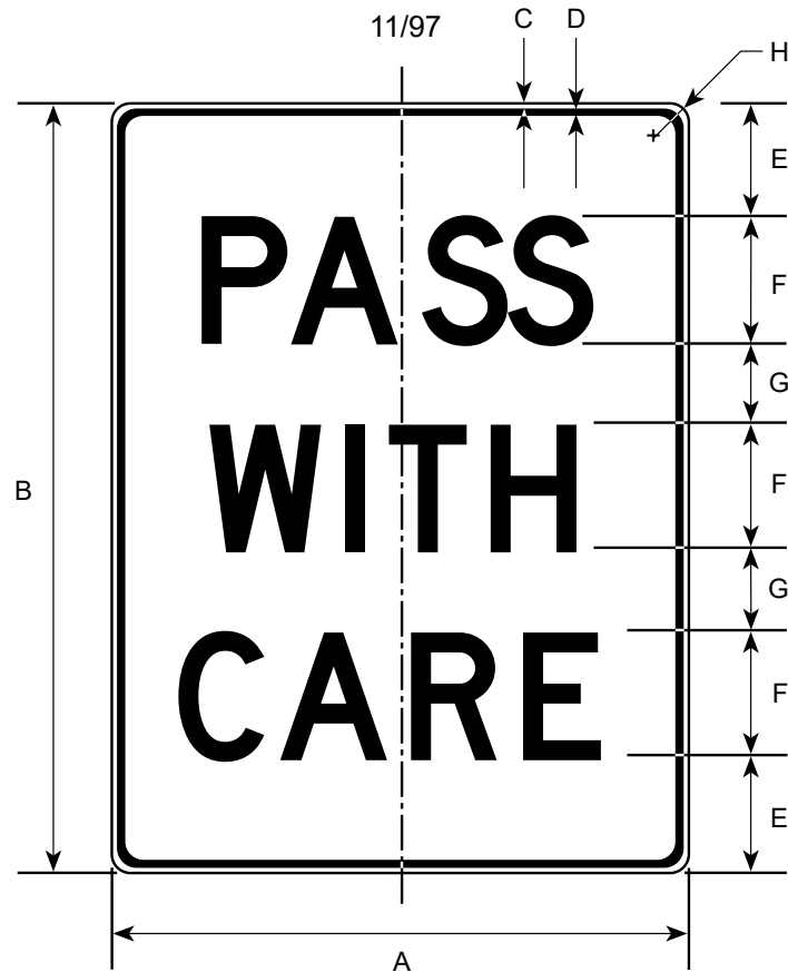
DIMENSIONS (MILLIMETERS)
