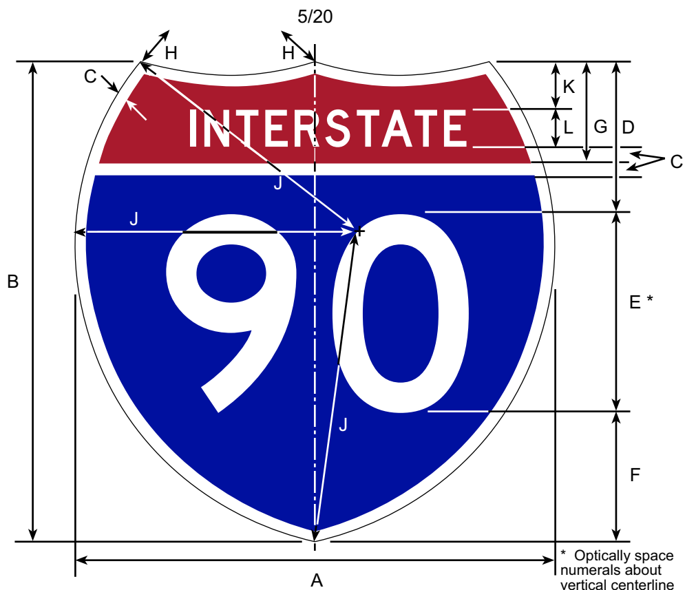
INTERSTATE SHIELD FOR INDEPENDENT & GUIDE SIGN USE
