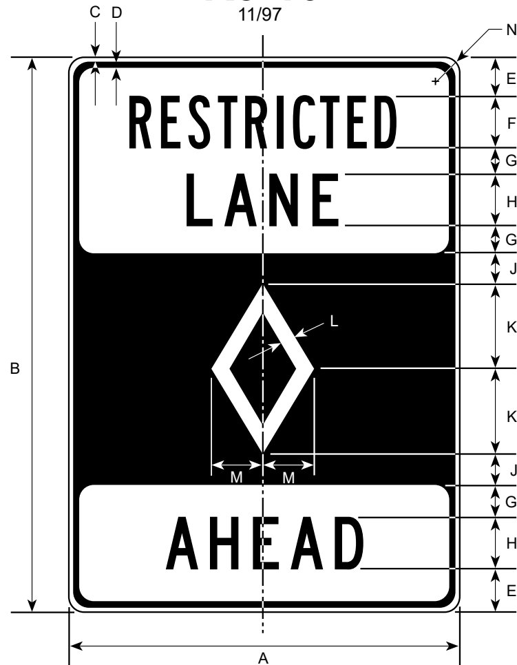
DIMENSIONS (MILLIMETERS)
