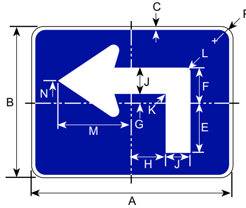
DIMENSIONS (MILLIMETERS)
