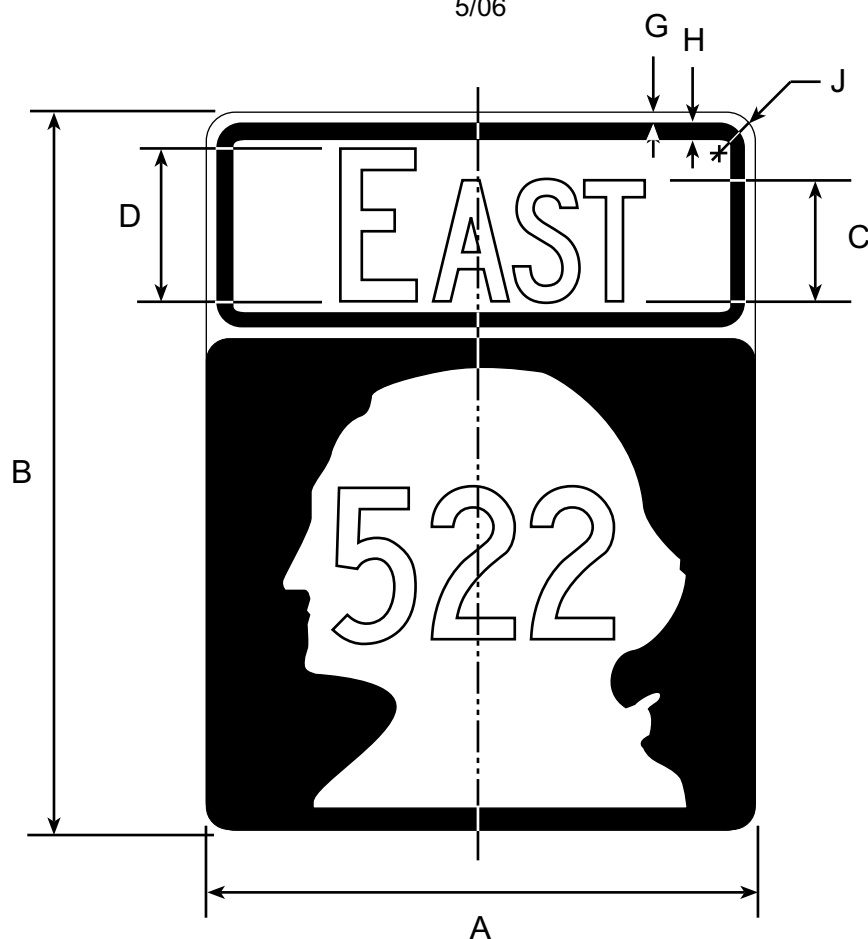
DIMENSIONS (MILLIMETERS)
