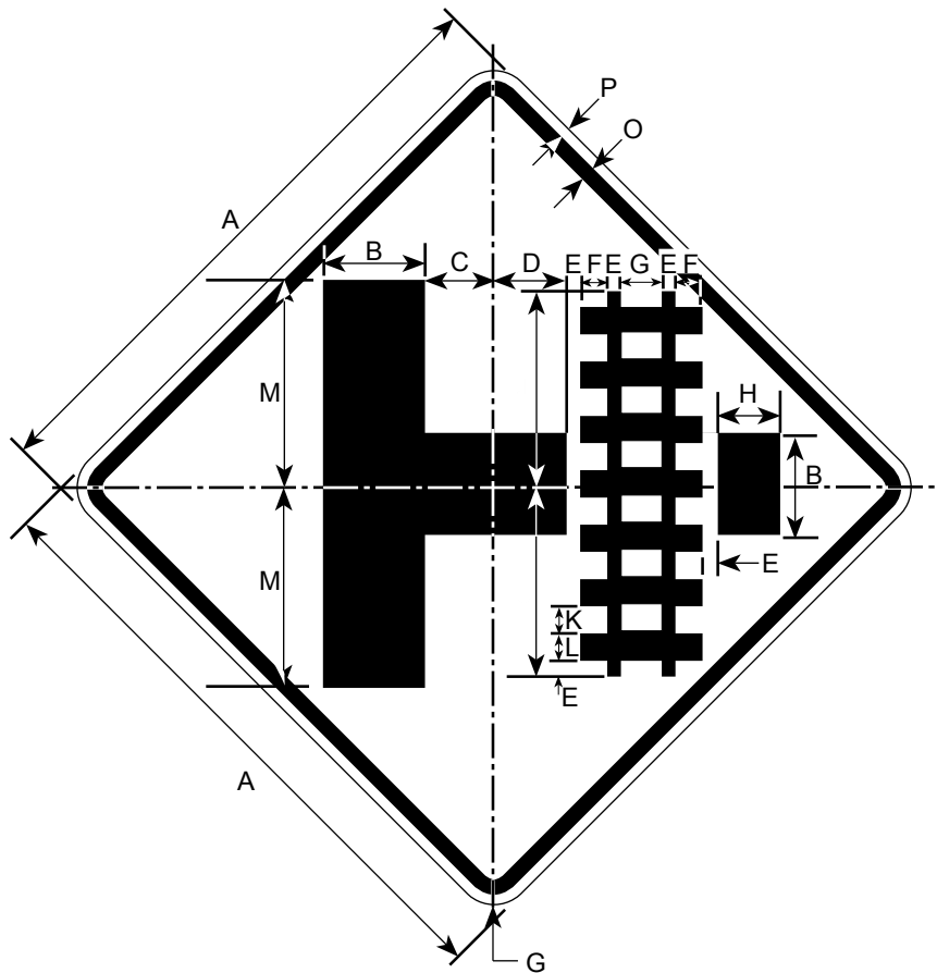
DIMENSIONS (MILLIMETERS)
