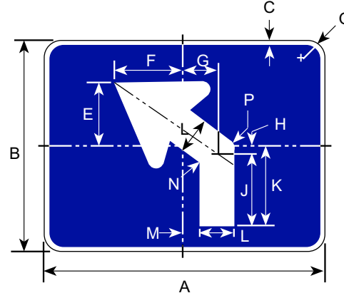
DIMENSIONS (MILLIMETERS)
