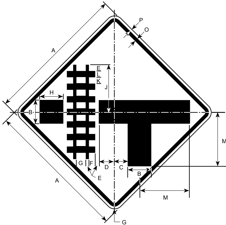
DIMENSIONS (MILLIMETERS)
