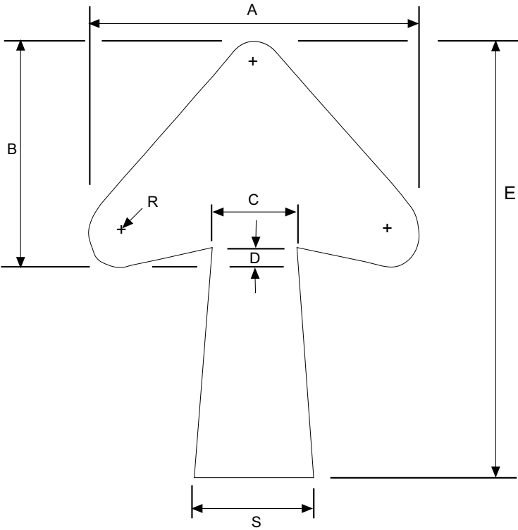
8 1/2 " X 10" ARROW DETAILS
