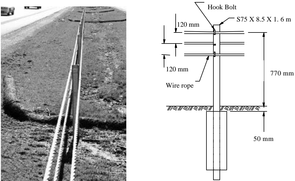
FIGURE 2 Typical cable median barrier installation and details.
