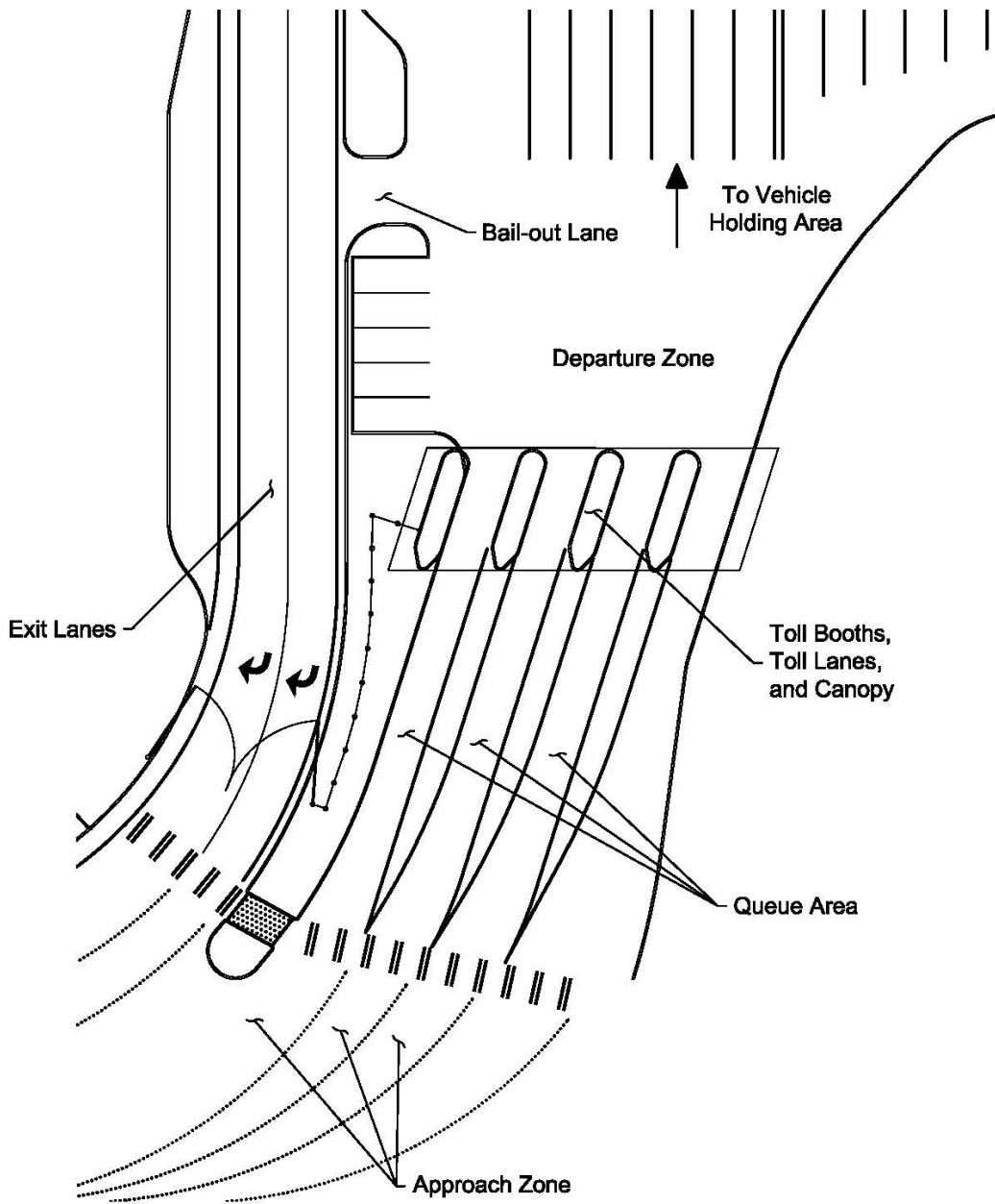
Example Toll Plaza Layout Exhibit 510-2
