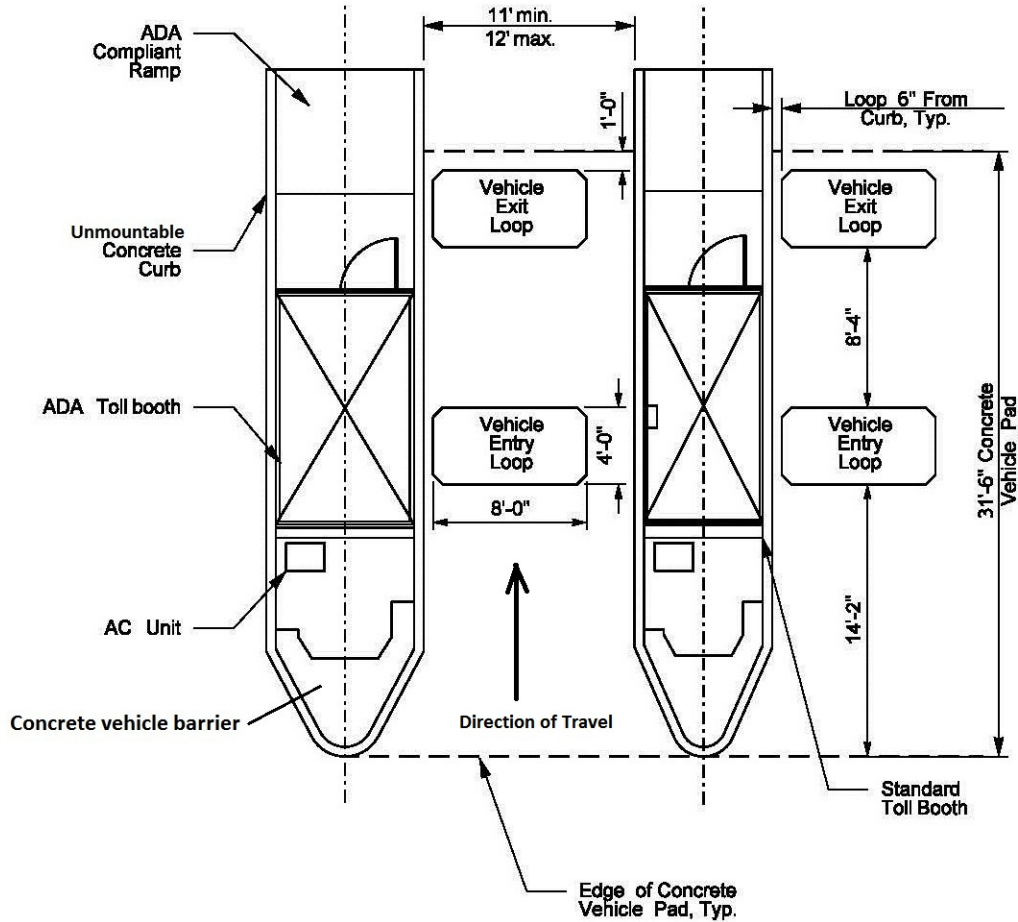
WSF Toll Booth Layout Exhibit 510-4
