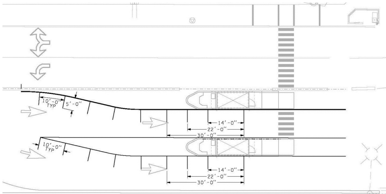
WSF Toll Booth Tariff Line Striping Exhibit 510-3
