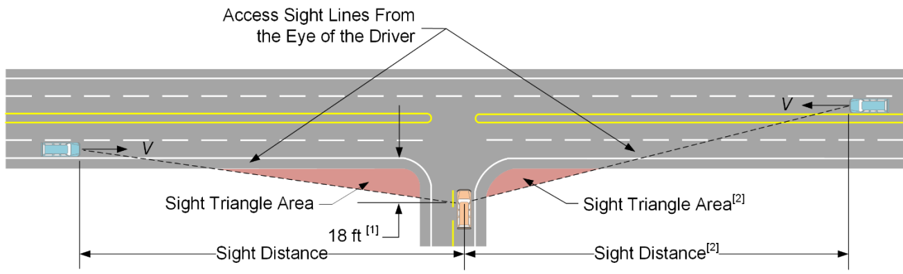
Exhibit 1340-3 Driveway Sight Distance
