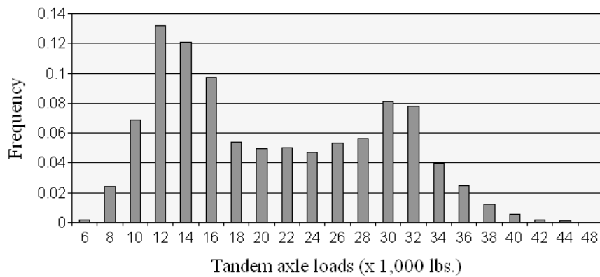
Figure C-14. Tandem axle load spectrum for Class 9 vehicles (Station P18-SB-2002)
