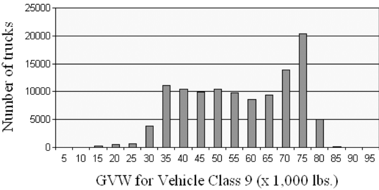
Figure 5-3. GVW distributions for station P4N (2000) (ideal GVW)
