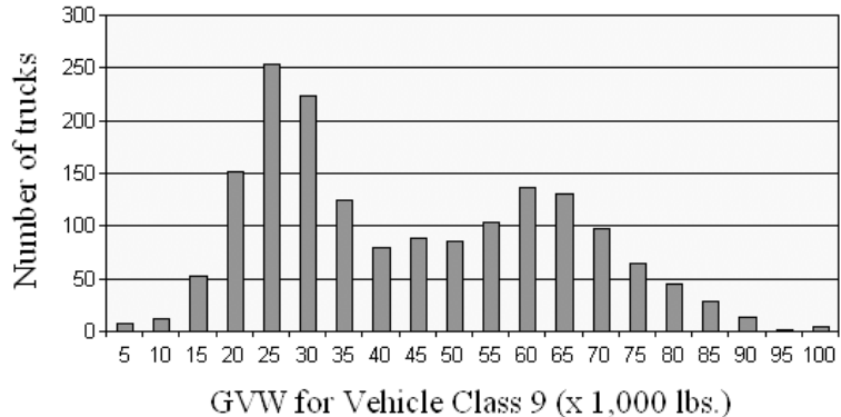
Figure 5-2. GVW distributions for station P18 (2001) (underestimated GVW)
