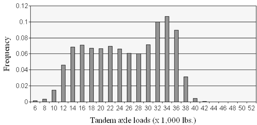
Figure C-24. Tandem axle load spectrum for Class 9 vehicles (Station P4N-2002)
