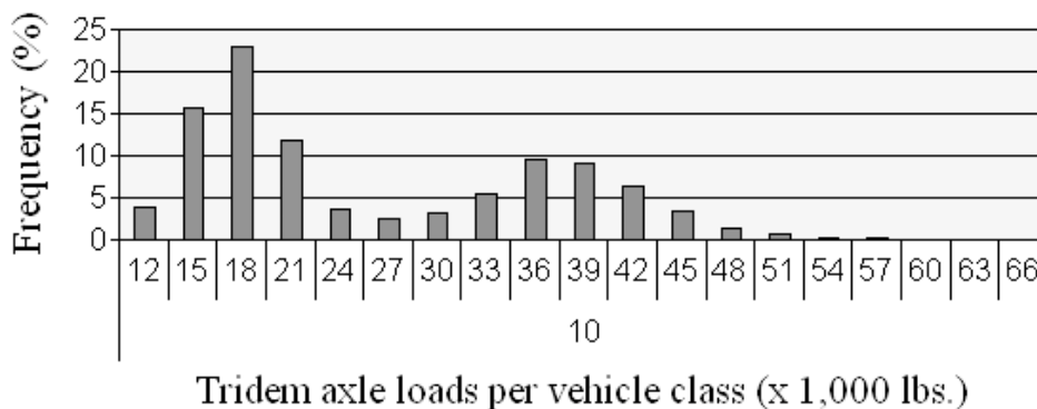
Figure E-2. Tridem axle load spectrum for Class 10 vehicles (Station B04-SB-2002)
