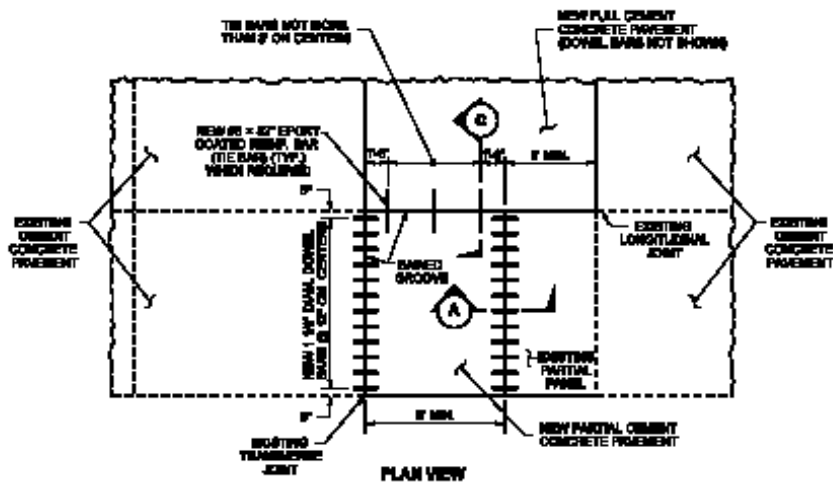
PLAN VIEW PARTIAL PANEL REPLACEMENT WITH TIE BARS
