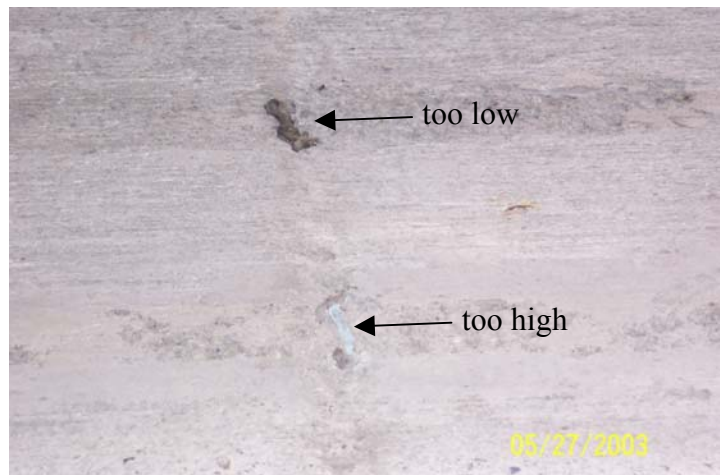
Photo 27. Foam core board placed too high and too low in slot.
