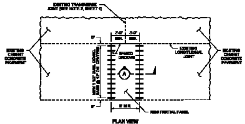
PLAN VIEW PARTIAL PANEL REPLACEMENT WITHOUT TIE BARS
