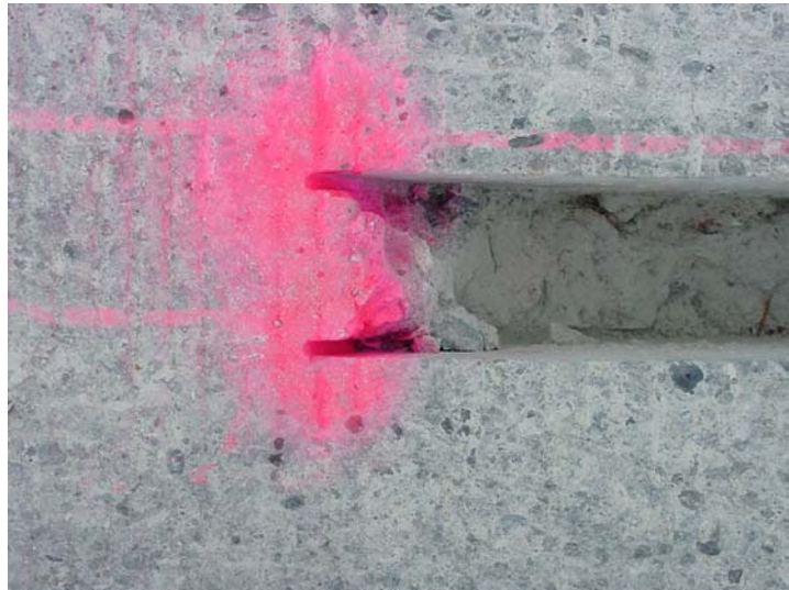
Photo 11. Concrete improperly removed from the end of the slot.
