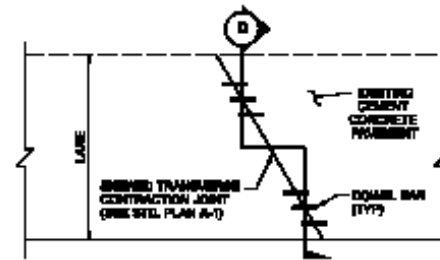
PLAN VIEW SKEWED JOINT DETAIL
