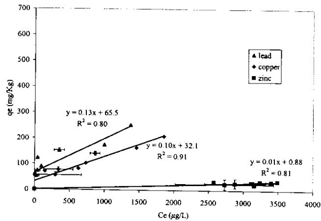
Figure 7. Sand/Clay multi-component isotherm data.
