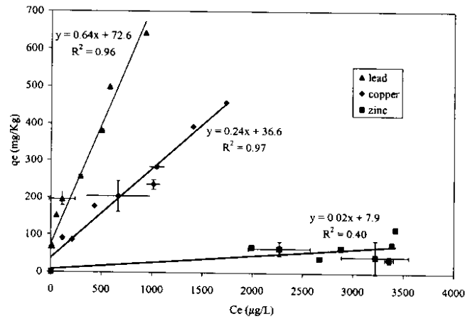
Figure 6. SPRIB multi-component isotherm data.
