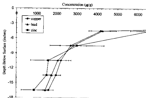
Figure 19. SPRIB column core results.
