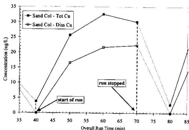
Figure 12. Results from an individual “storm.”
