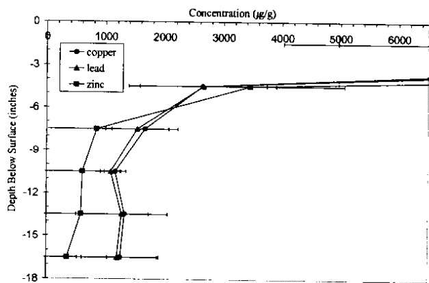
Figure 18. Sand column core results.
