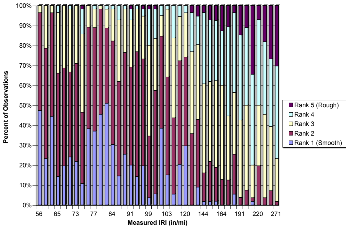
Figure 16. Cumulative Percentage Plot of Roughness Rankings on Each Test Section vs. Corresponding Ordered IRI Measurements
