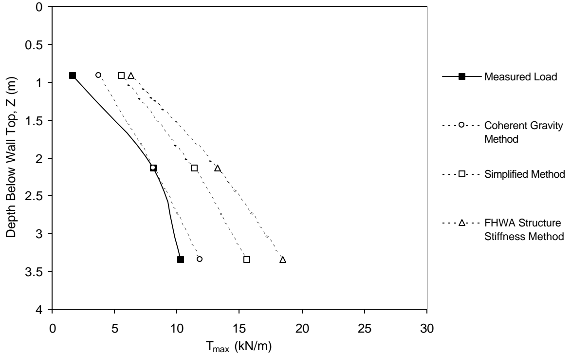
Figure A-21. Predicted and measured reinforcement peak loads for Hayward bar mat reinforced wall, Section 2, no surcharge (BM2).
