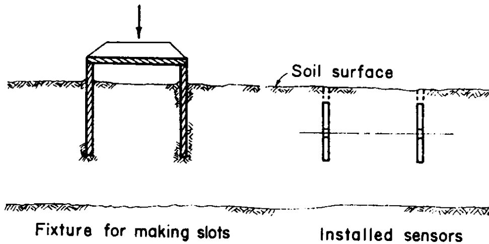
Figure 7-2. Installation for Horizontal Strain
