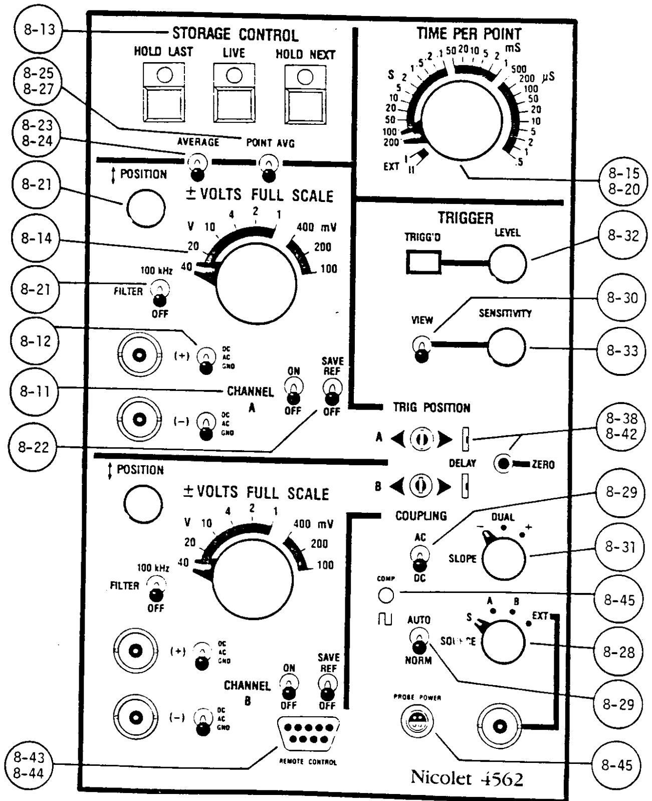
Figure 11 Nicolet Plug-in Amplifier Unit
