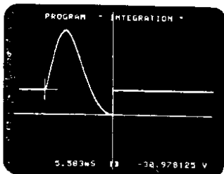
Fig. 17. Integration of cursor-indicated section of waveform in Figure 16.
