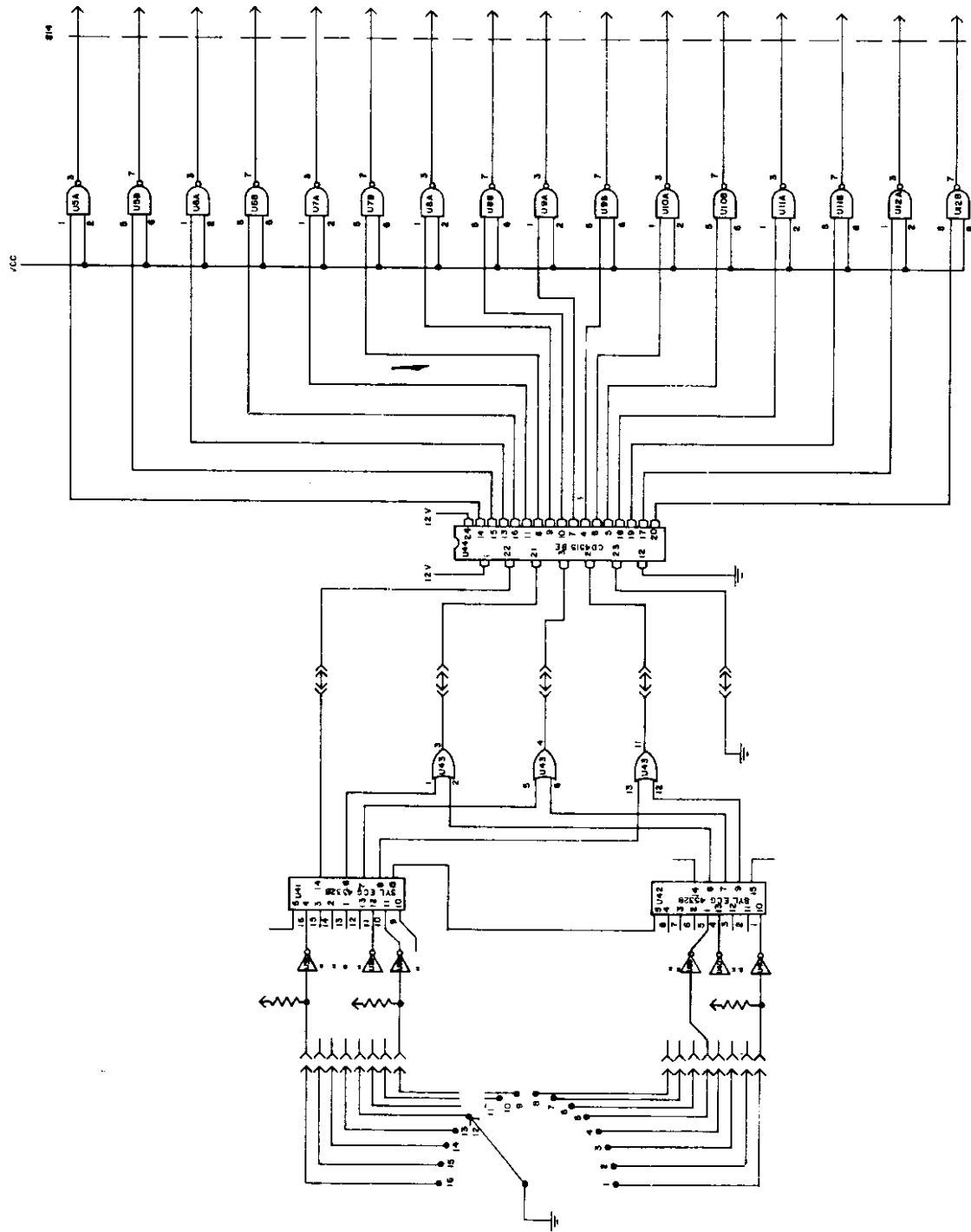
Figure 9 Switching Circuit and Control Diagram
