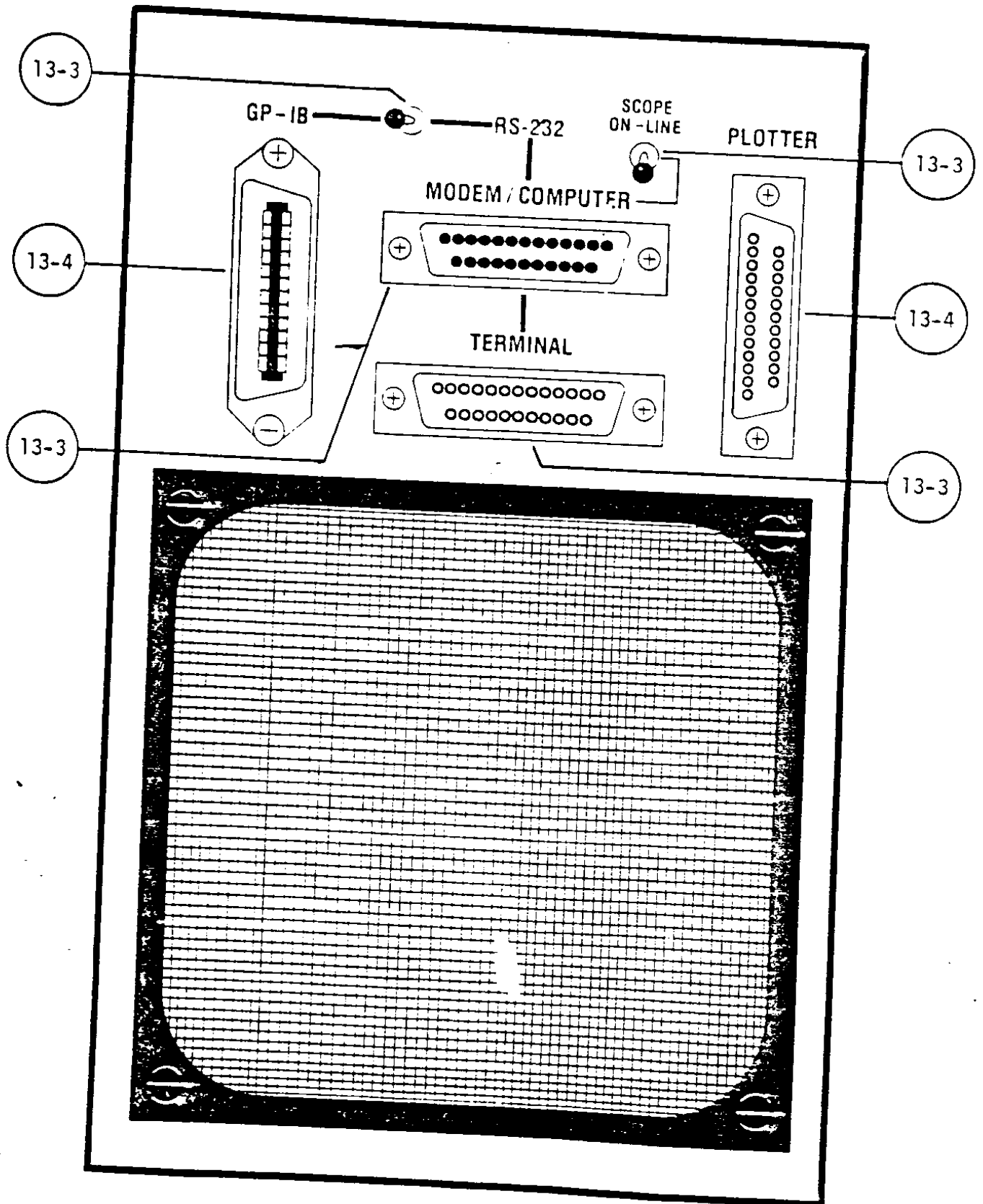
Figure 14 Nicolet Input/Output
