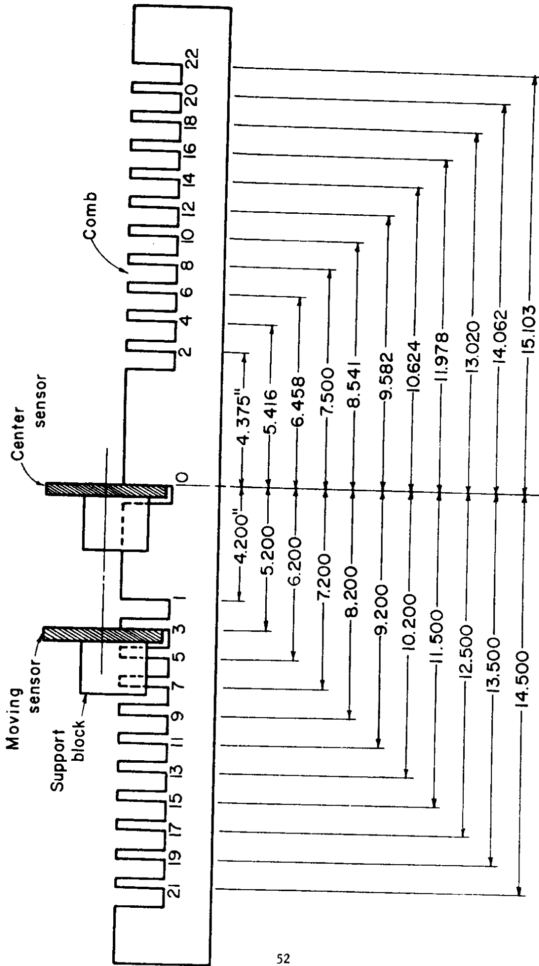
Figure 6-4. Calibration Comb Dimensions for 4-in. Sensor
