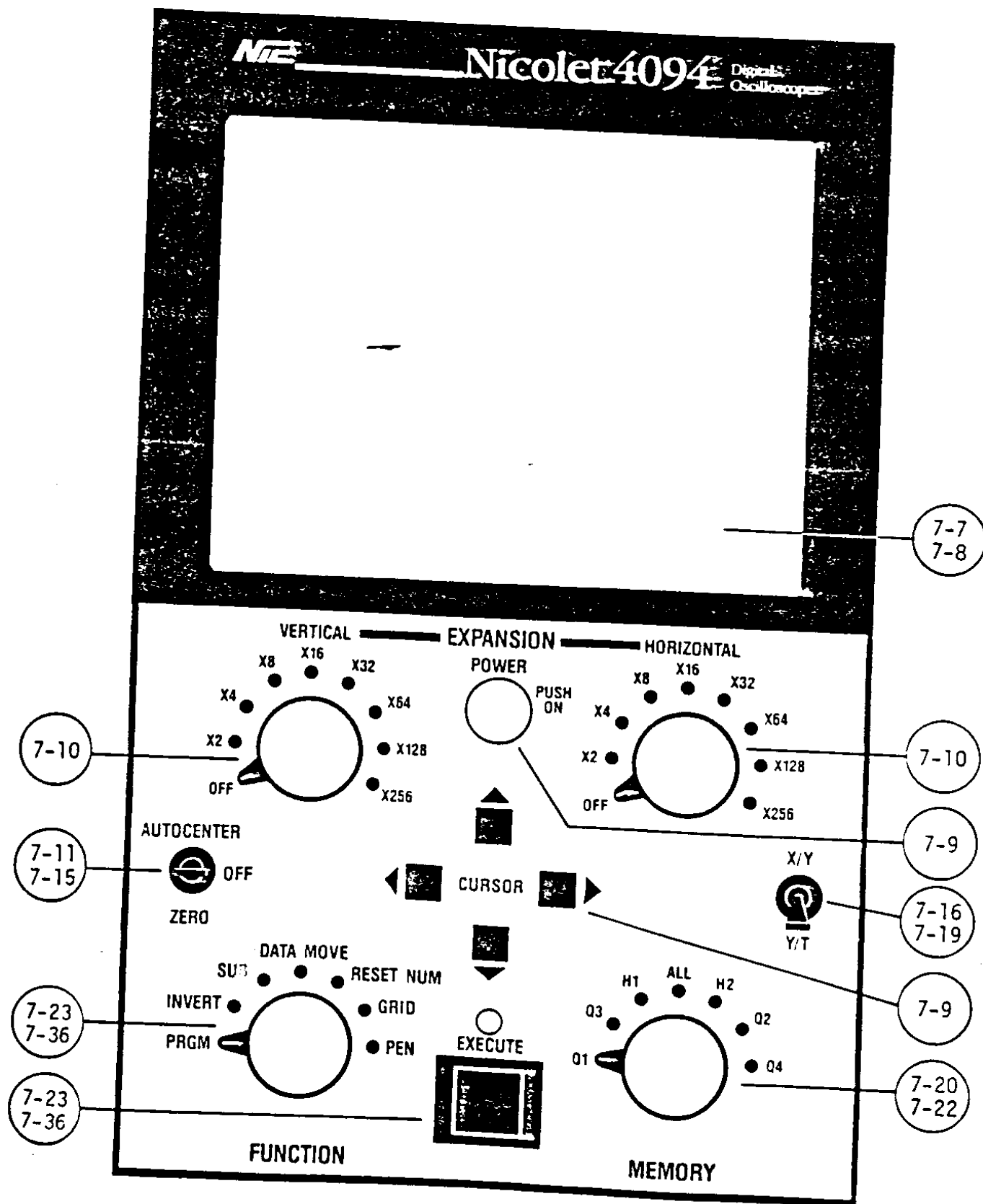
Figure 12 Nicolet Mainframe
