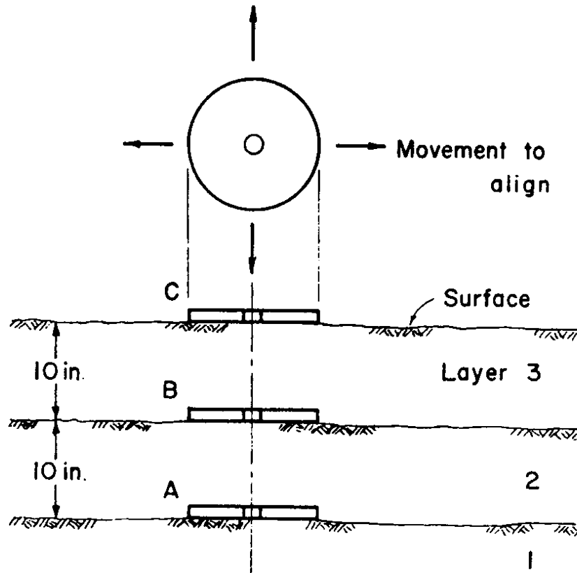
Figure 7-1. Electrical Centering of Sensors
