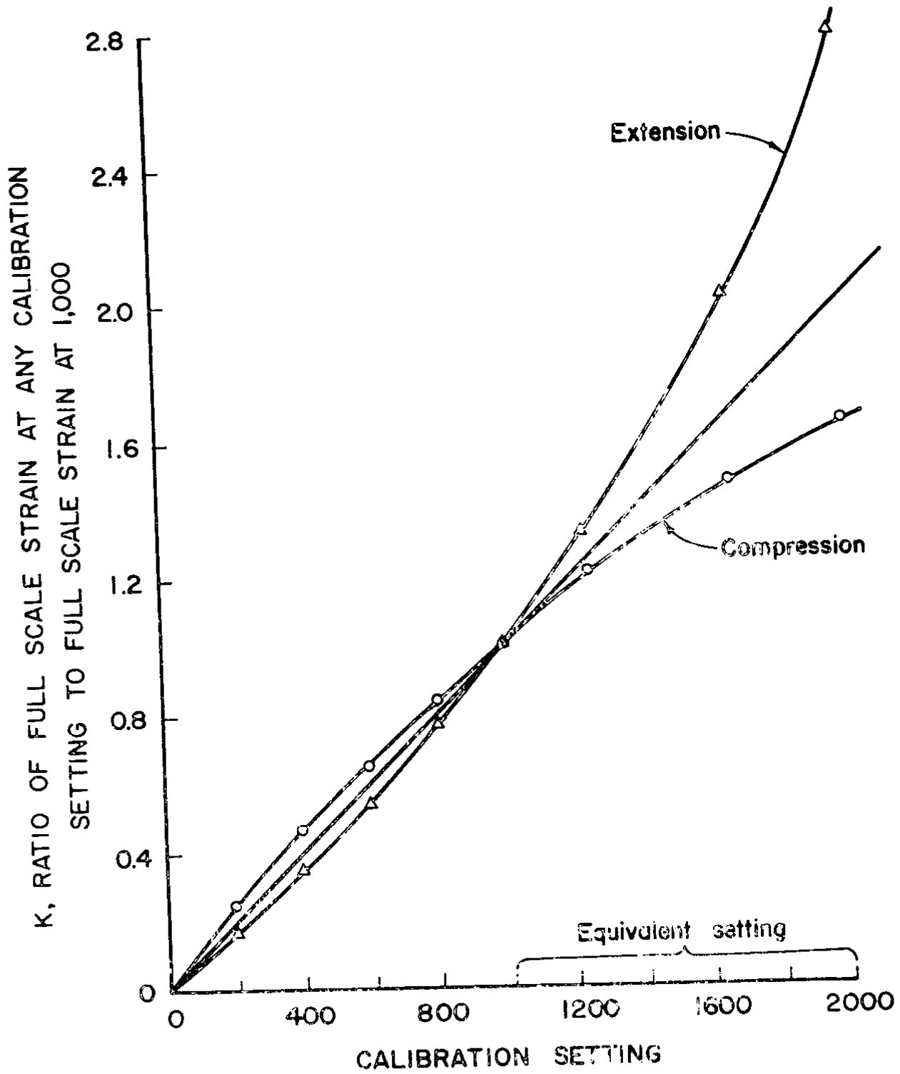
Figure 5-8. Variation of Calibration Strain with Calibration Setting (Range 3, Amp Dial = 500, Sensors = 2-in. diam)
