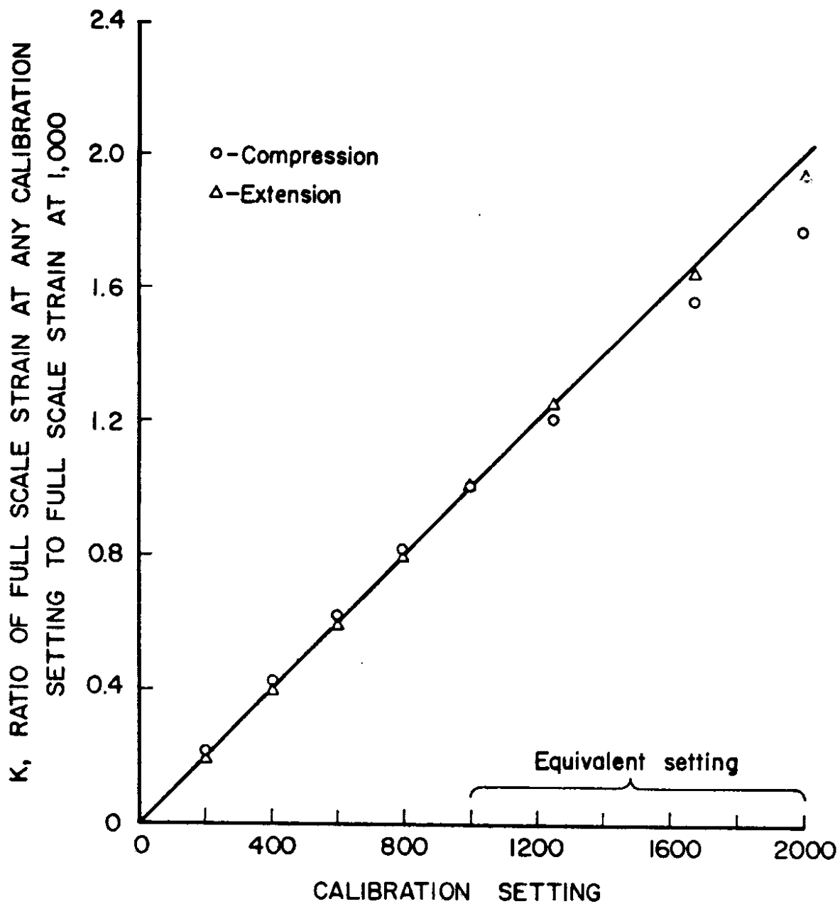
Figure 5-7. Variation of Calibration Strain with Calibration Setting (Range 2, Amp Dial = 500, Sensors = 2-in. diam)
