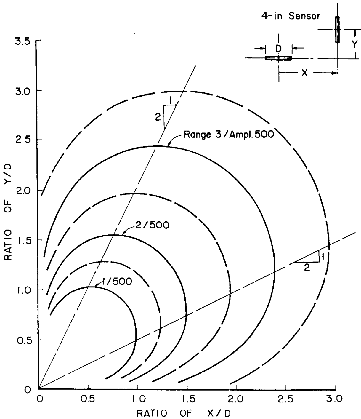
Figure 8-4. Lines of Equal Potential for Perpendicular Coil Configuration
