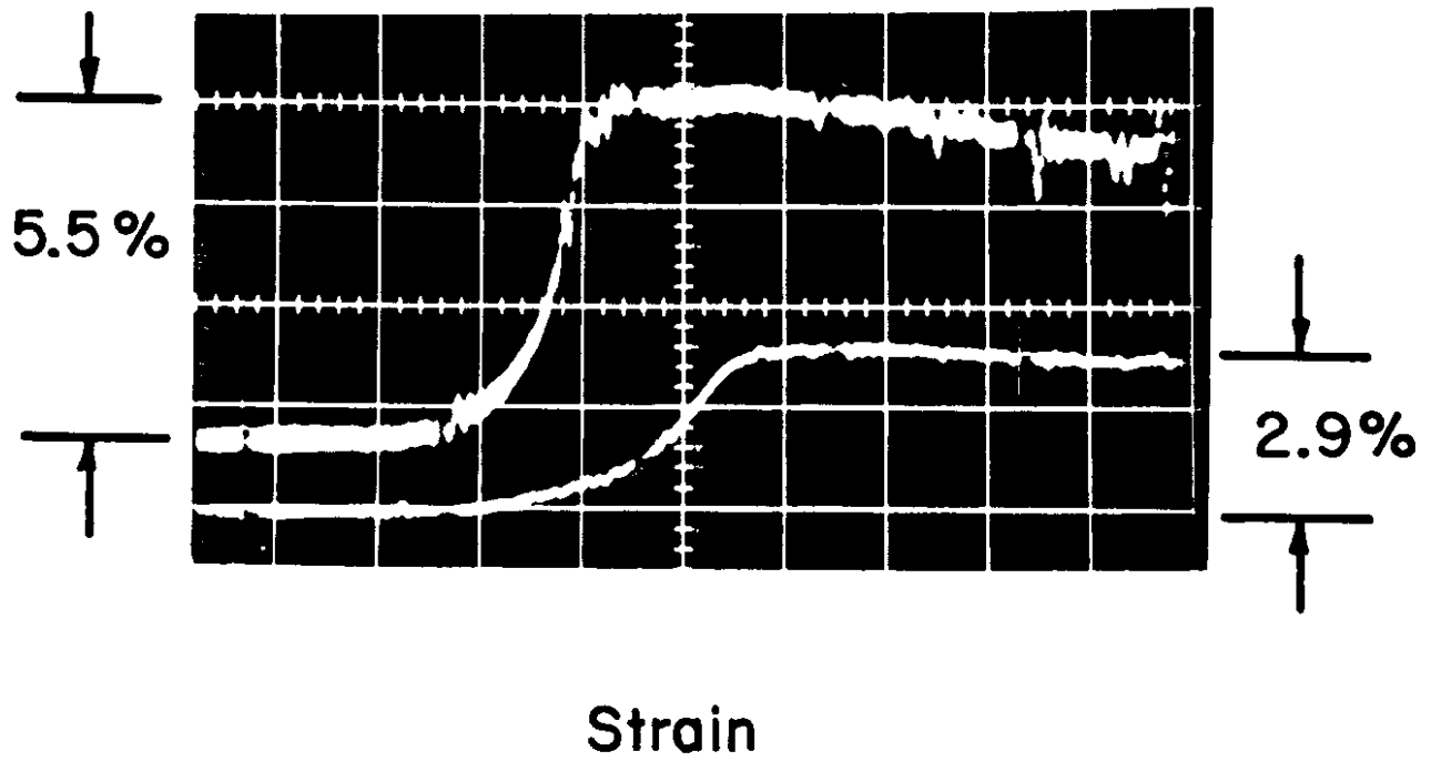
Figure 9-2. Stress and Strain Measurements During Shock Propagation
