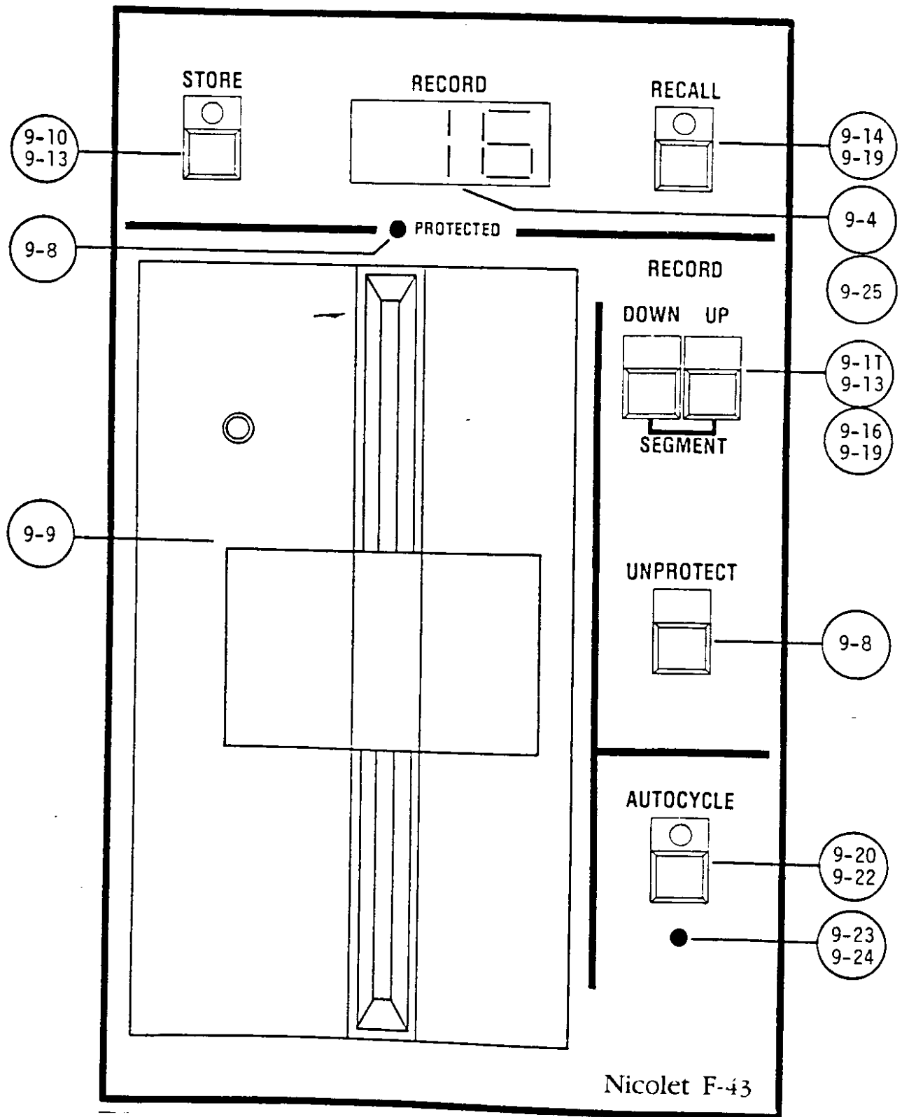
Figure 13 Nicolet Disk Recorder
