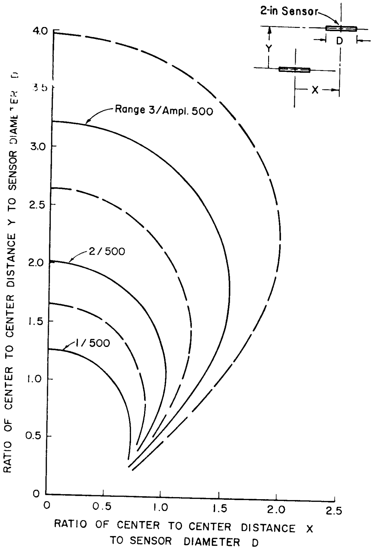
Figure 8-3. Lines of Equal Potential for Parallel Coil Configuration
