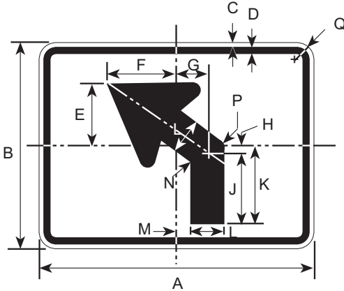
DIMENSIONS (MILLIMETERS)
