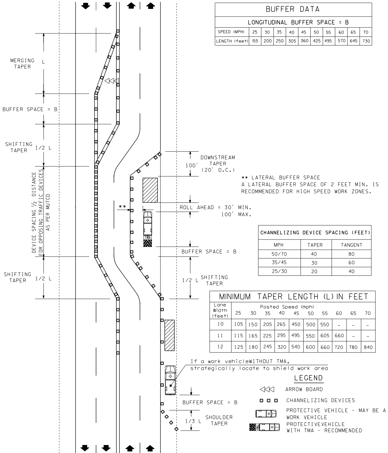
TAPER AND BUFFER SPACE DETAILS
