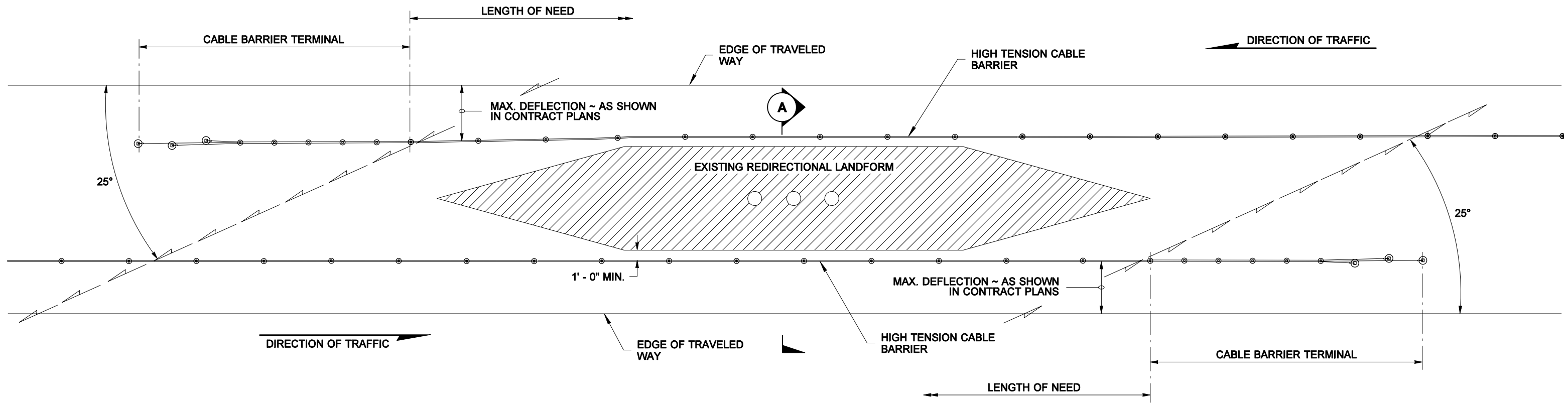
PLAN VIEW CASE 27
