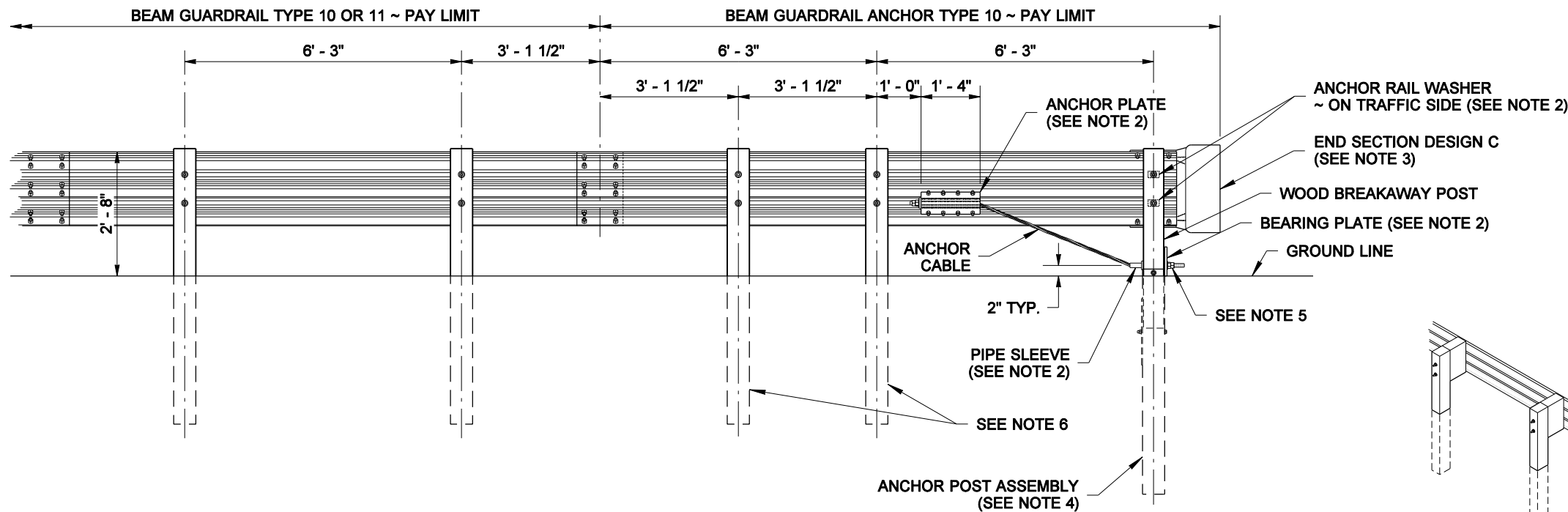
ELEVATION VIEW THRIE BEAM
