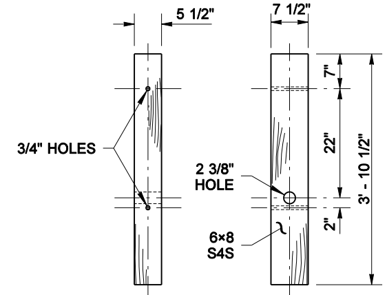
WOOD BREAKAWAY POST DETAIL
