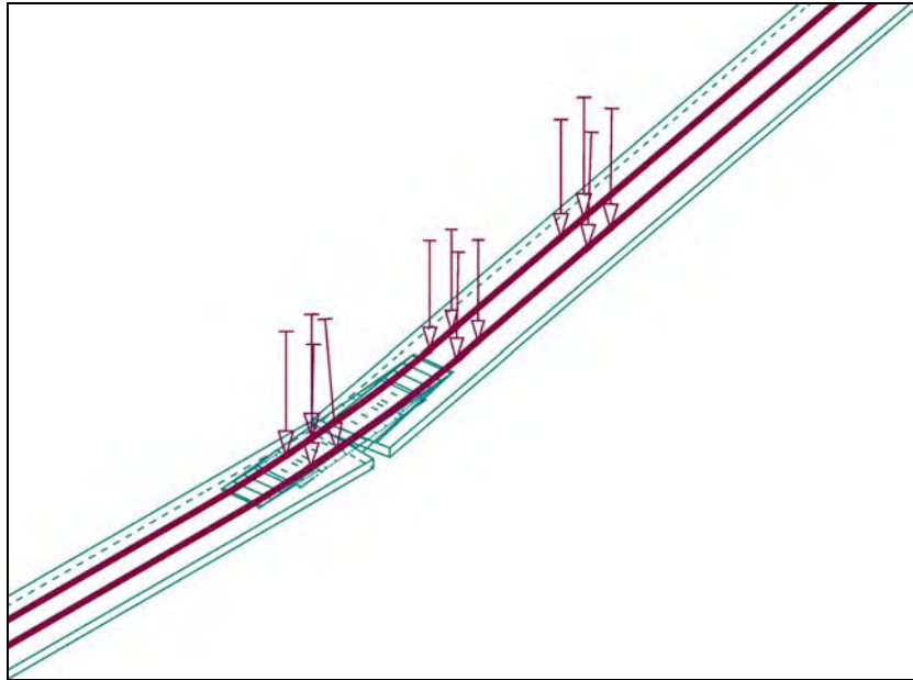
Figure 3-29: Maximum Lateral (ZZ) Rotation and Wheel Reactions (zoomed).
