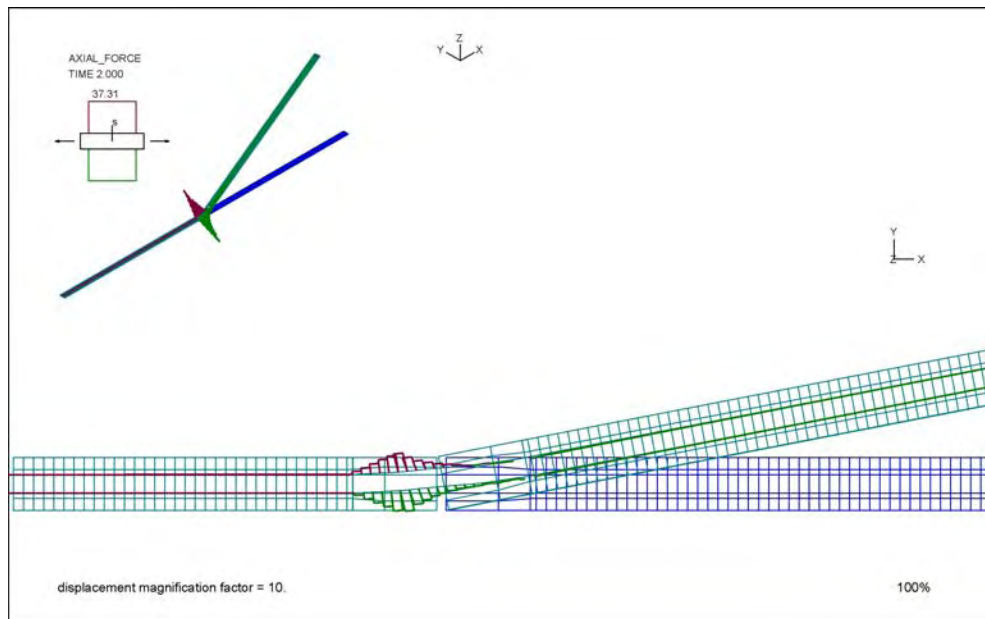
Figure 3-20: Combined Maximum Vertical (YY) and Lateral (ZZ) Rotation – Rail Axial Force on Deformed Mesh.
