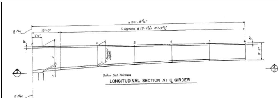
Figure 3-34: Variation in Depth for Cross-Sections along a Typical Span.
