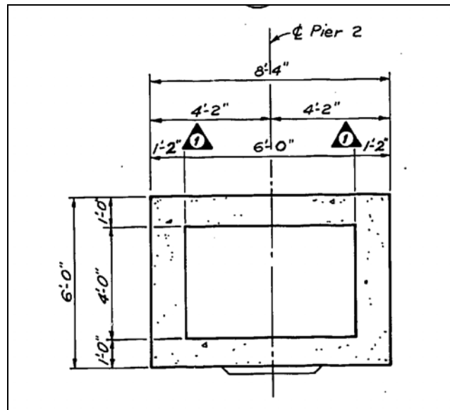
Figure 3-35: Transverse beam at Pier 2
