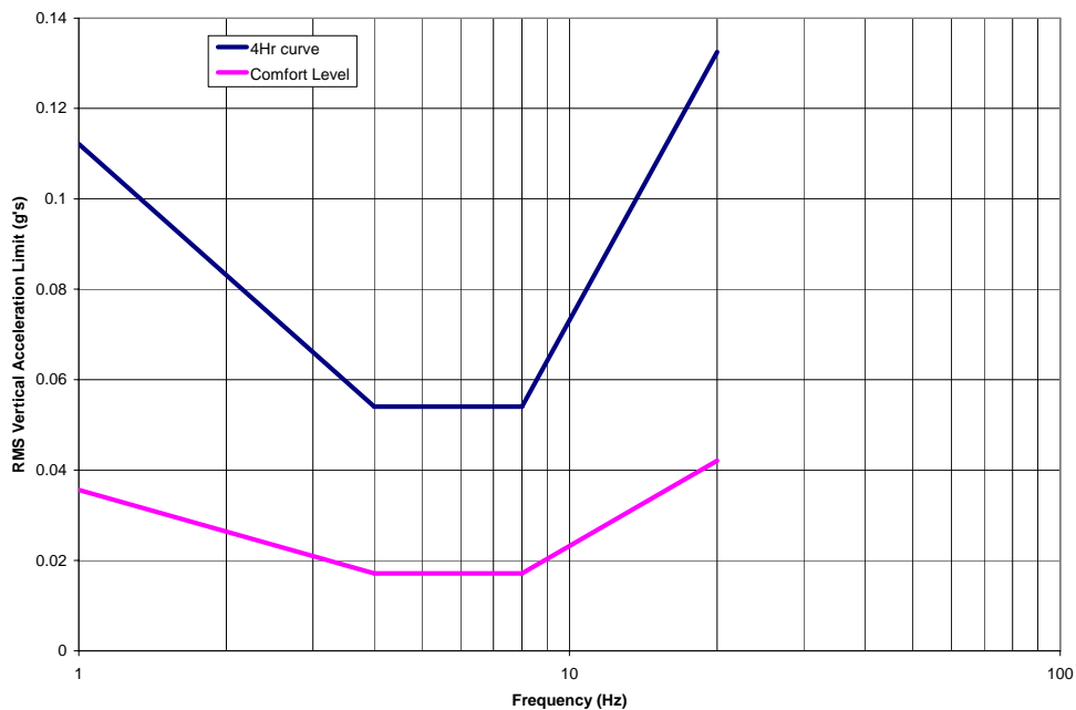
Figure 3-9: Reformatted Vertical Acceleration Limits
