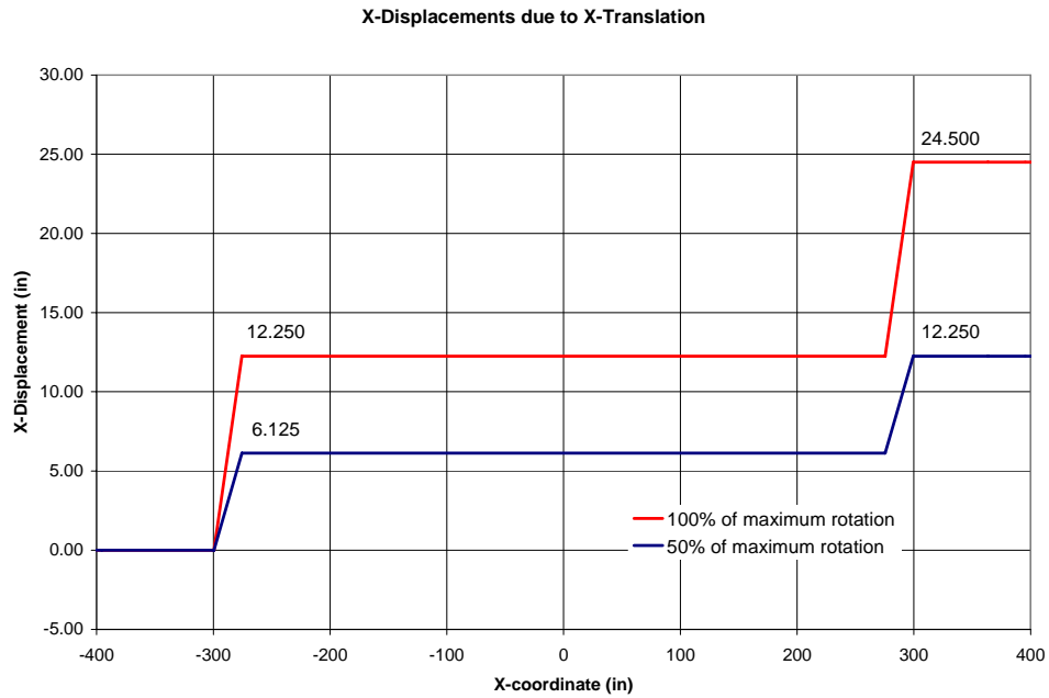
Figure 3-16: Rail Longitudinal (X) Displacements due to Joint Longitudinal (X) Translation.
