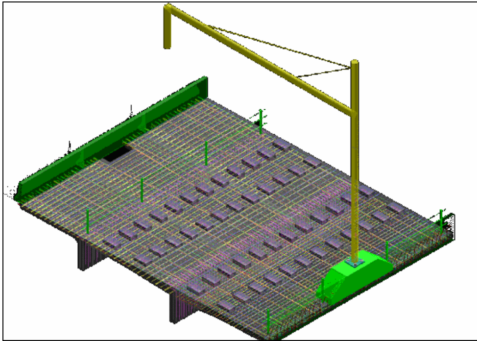
Figure 2-1: Two-Track OCS Cantilever Structure (Parsons and INCA [1])
