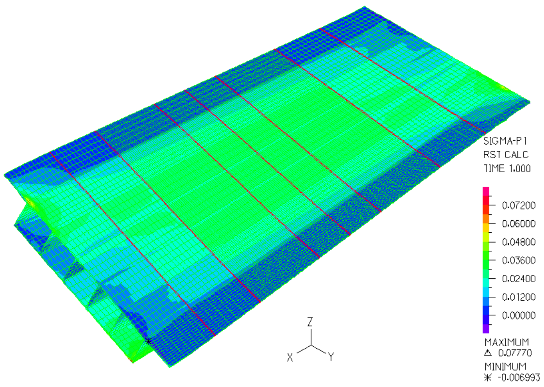
Figure 3-3: Principal Tensile Stress (Sp1) Contour Plot under a Torsion of 6202 kip-ft
