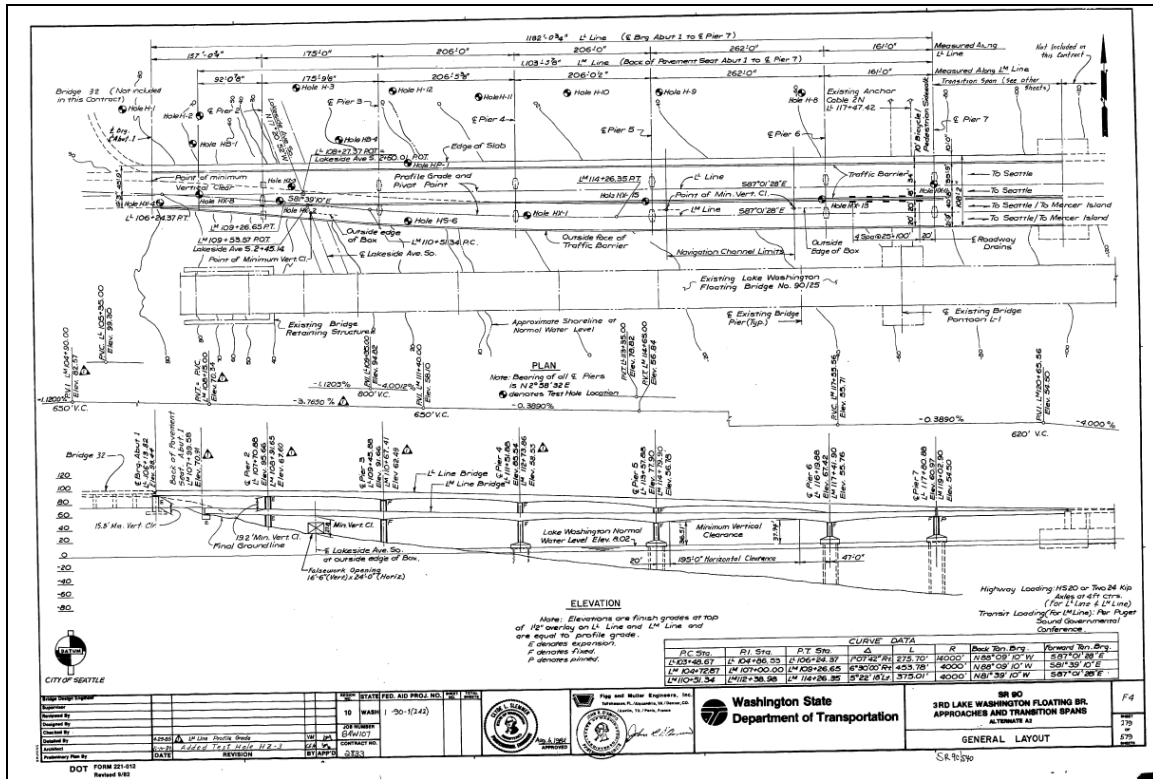
Figure 3-1: Approaches and Transition Spans
