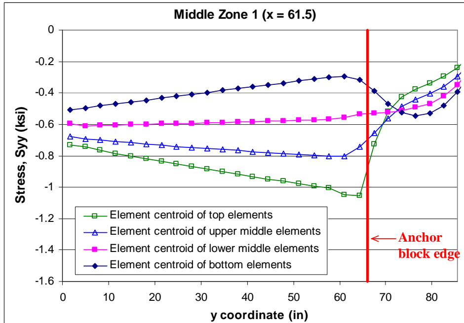
Figure 3-2: Transverse Stress (Syy) Variation in the y-direction
