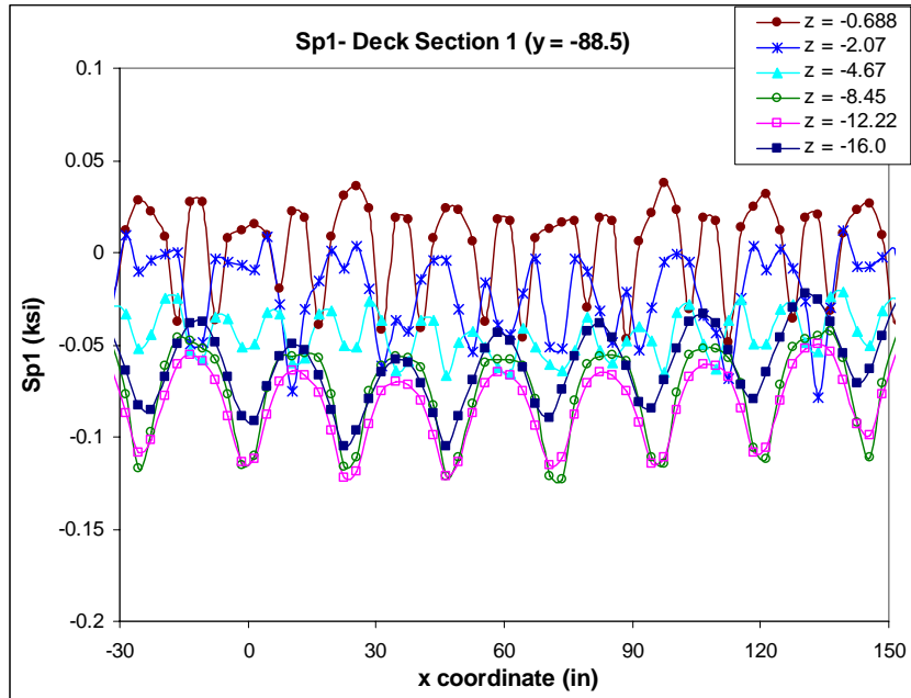
Figure 3-13: Principal Tensile Stress (Sp1) Variation in the x-direction at Deck Section 1 - Self Weight + Post Tension Forces + Light Rail Vehicle Loads (Case 2)
