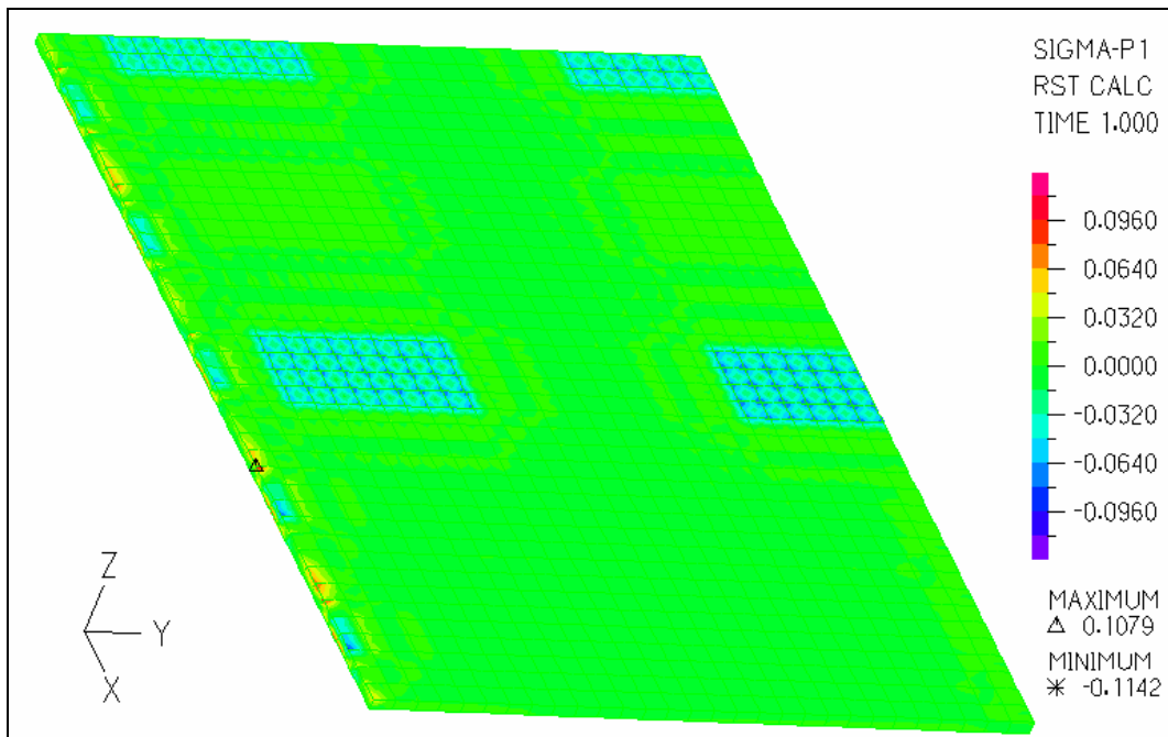
Figure 3-17: Principal Tensile Stress Contour Plot at the Top Surface of the Deck – Self Weight + Post Tension Forces + Light Rail Vehicle Loads +OCS Loads (Case 1)
