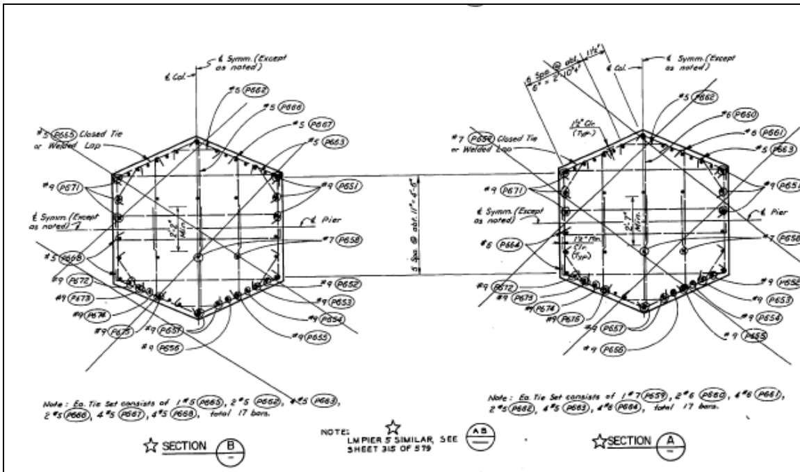
Figure 3-28: LM Pier 6 – drawing 318
