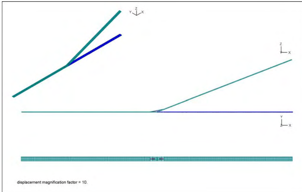
Figure 3-10: Maximum Vertical (YY) Rotation – Deformed Mesh.
