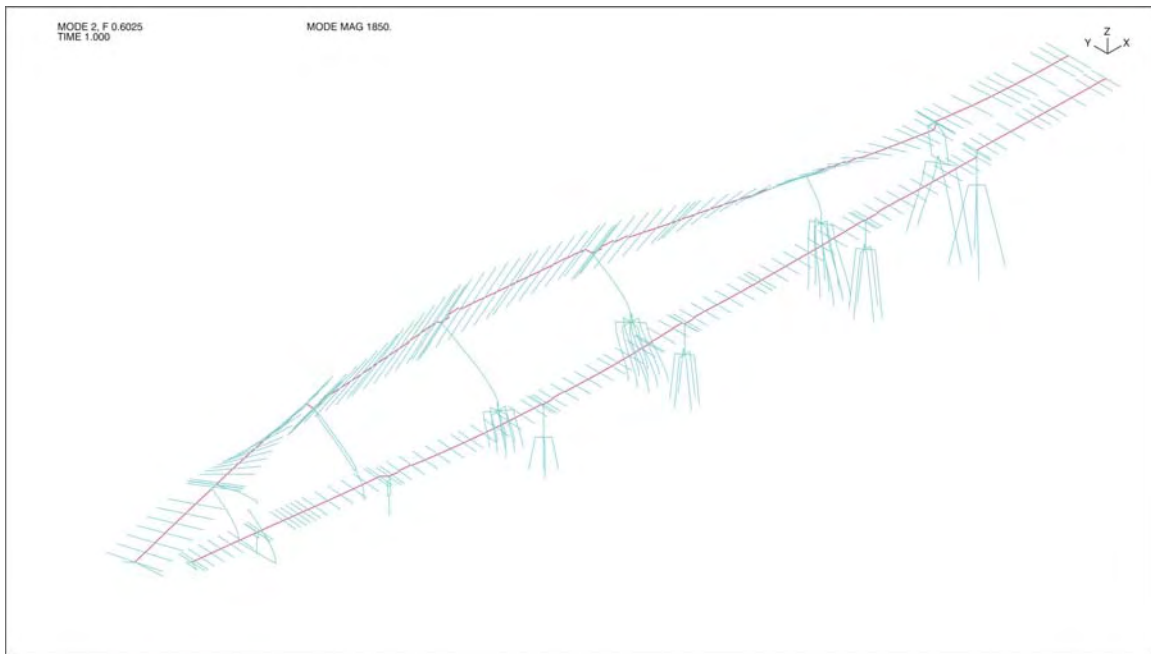
Figure 3-37: Mode Shape 2 (Transverse Line L – Period = 1.66 sec)
