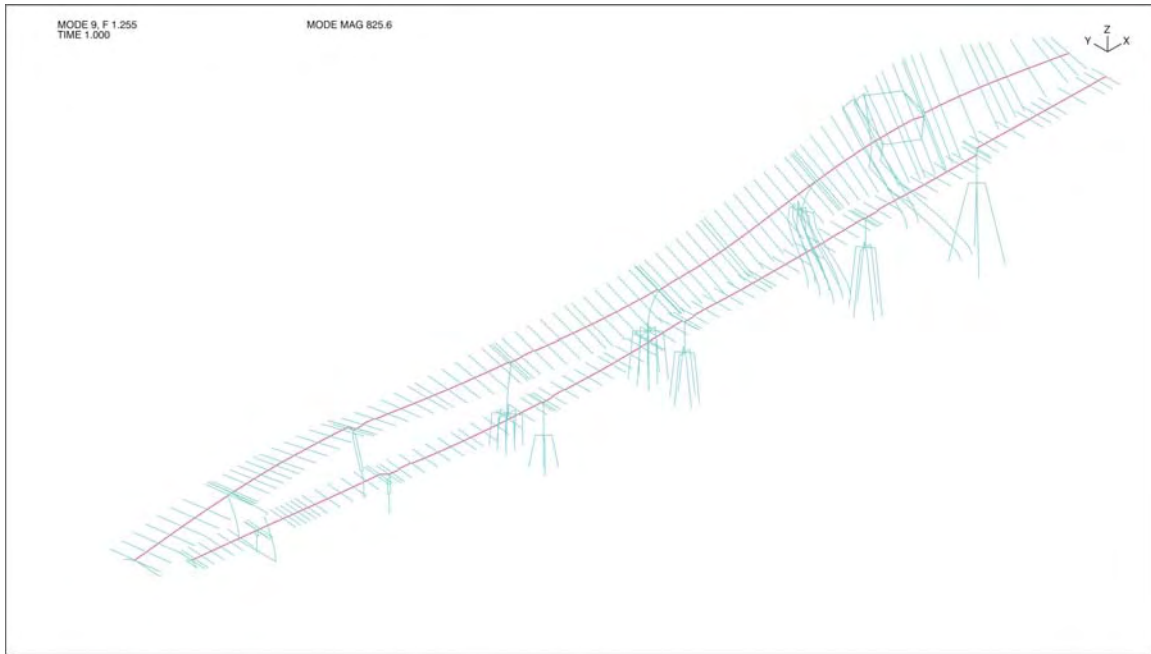
Figure 3-44: Mode Shape 9 (Transverse Line L – Period = 0.80 sec)
