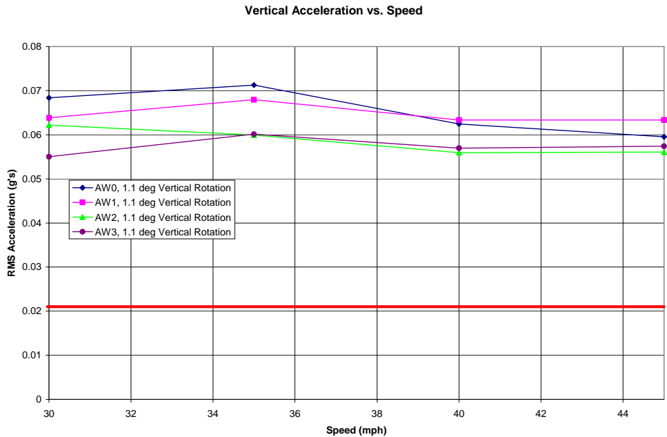
Figure 3-15: RMS Vertical acceleration with 1.1° vertical rotation at joint.
