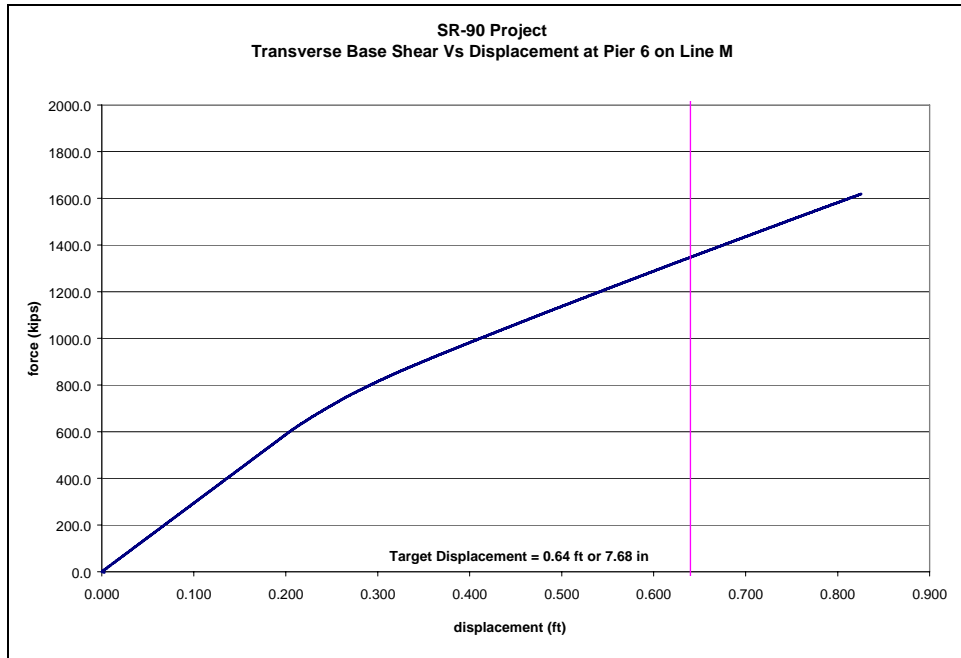
Figure 3-72: Column Force vs. Displacement at Pier 6 on Line M
