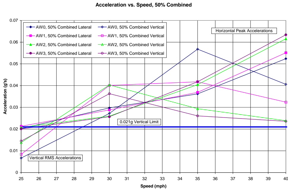
Figure 3-18: RMS Vertical and Peak Horizontal Acceleration with 1.1° Vertical and 0.55° Horizontal Rotation at Joint.
