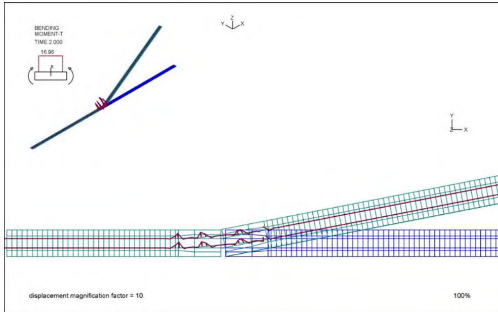
Figure 3-23: Combined Maximum Vertical (YY) and Lateral (ZZ) Rotation – Rail Bending Moment-T (about Vertical Axis) on Deformed Mesh.
