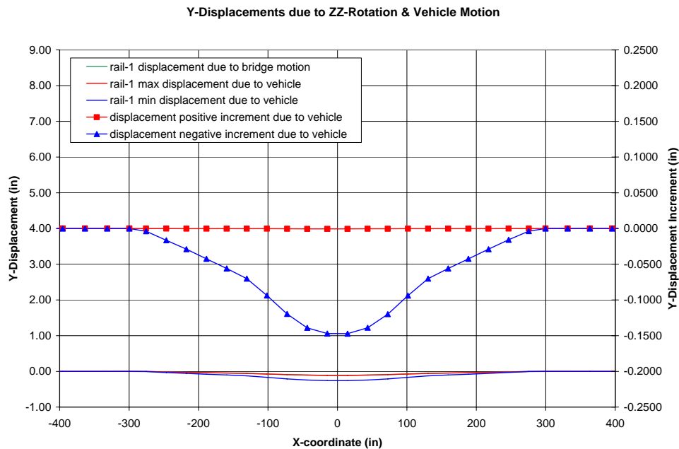
Figure 3-31: Rail Vertical (Z) Displacements due to Joint Lateral (ZZ) Rotation and Wheel Reactions.
