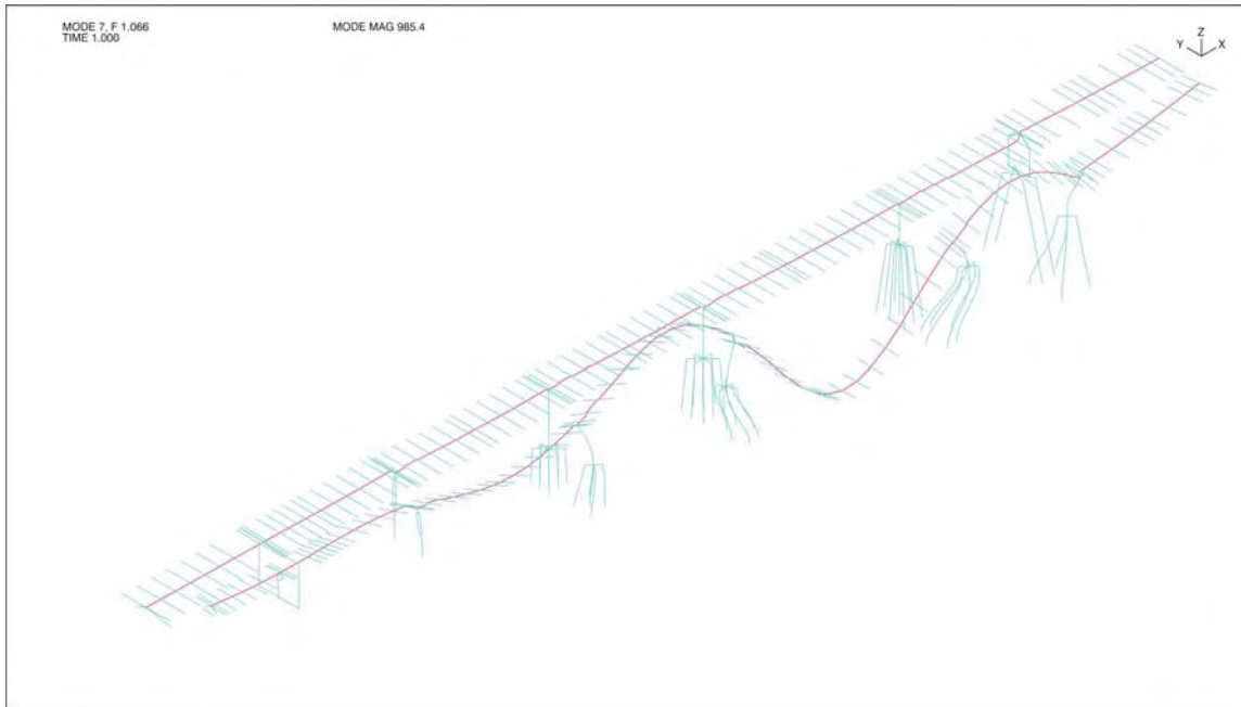
Figure 3-42: Mode Shape 7 (Vertical Line M – Period = 0.94 sec)
