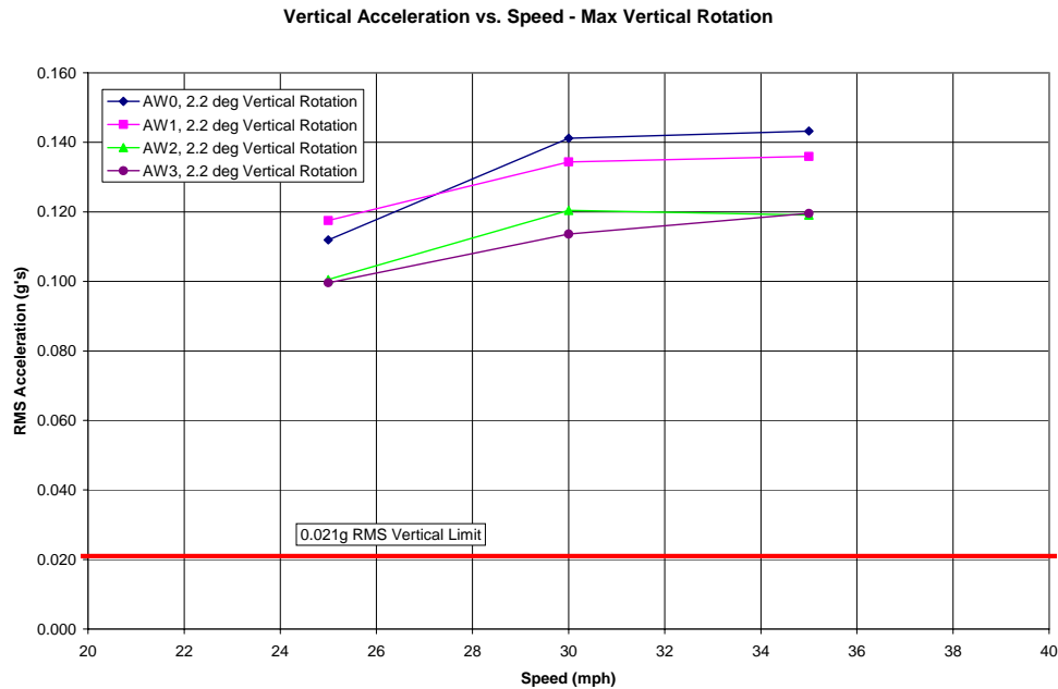
Figure 3-14: RMS Vertical acceleration with 2.2° Vertical rotation at joint
