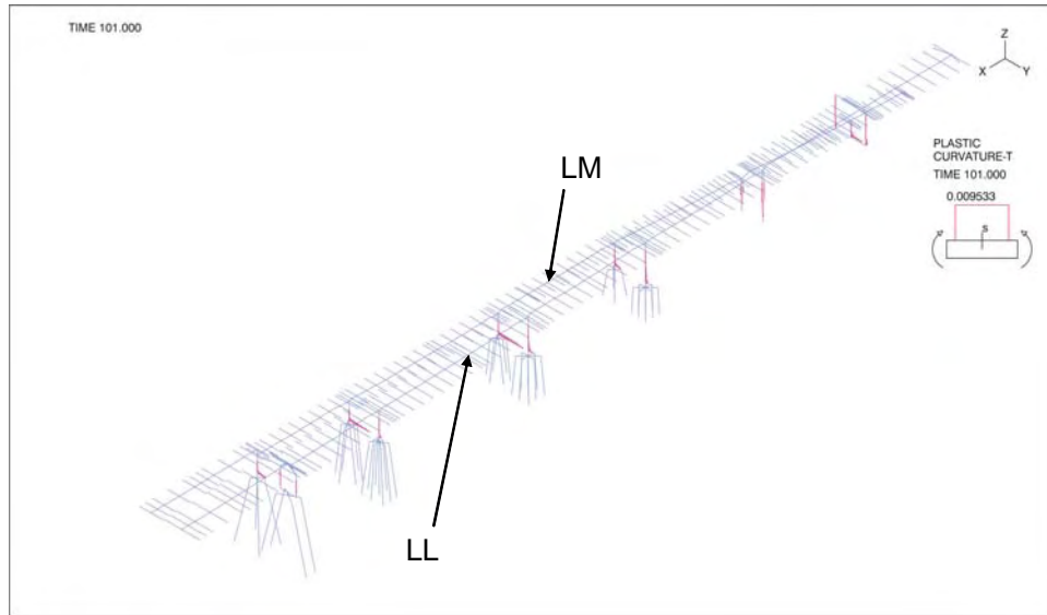
Figure 3-49: Plastic Curvature about Longitudinal axis (T-axis) at the Target Displacement
