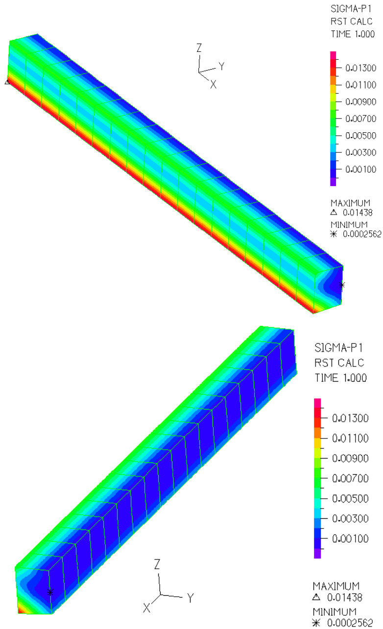
Figure 3-6: Principal Tensile Stress (Sp1) Contour Plots at the Deck Element Zone 1 under a Torsion of 6202 kip-ft
