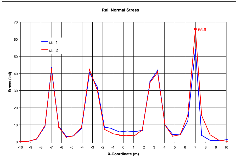
Figure 3-34: Combined Maximum Vertical (YY) and Lateral (ZZ) Rotation – Rail Normal Stress Envelope (ksi).
