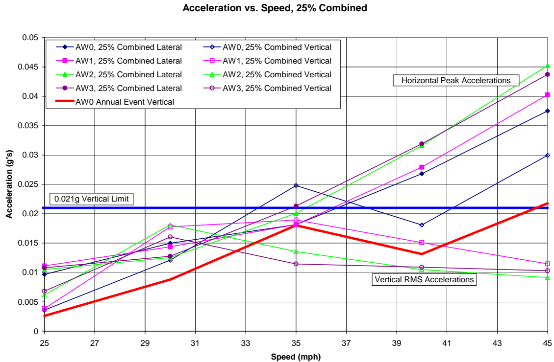
Figure 3-19: RMS Vertical and Peak Horizontal Acceleration with 0.55° Vertical and 0.275° Horizontal Rotation at Joint.
