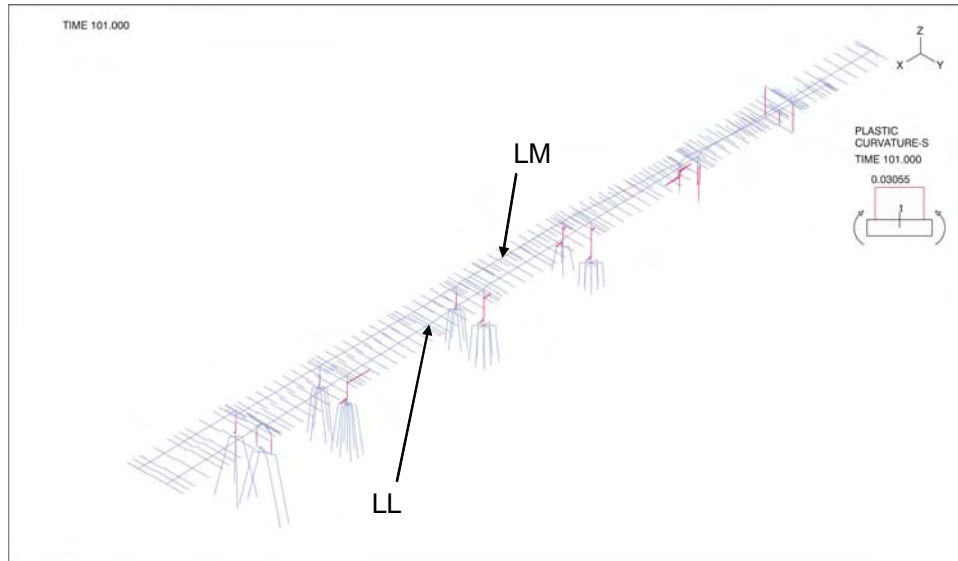
Figure 3-47: Plastic Curvature about Transverse axis (S-axis) at the Target Displacement
