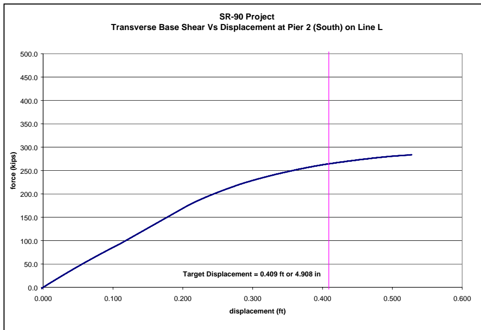
Figure 3-61: Column Force vs. Displacement at Pier 2 (South Column) on Line L
