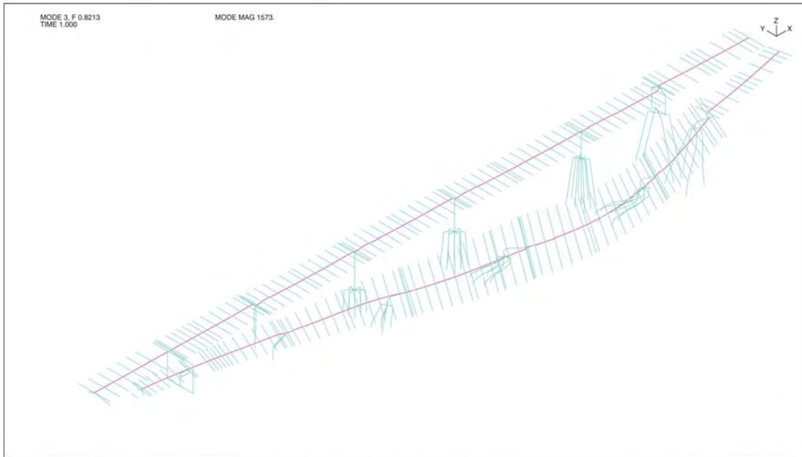
Figure 3-38: Mode Shape 3 (Transverse Line M – Period = 1.22 sec)
