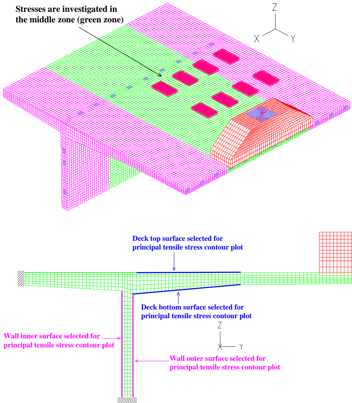
Figure 3-5: Coordinate Reference Points and Critical Sections selected for Stress Value Investigation – Cantilever Model
