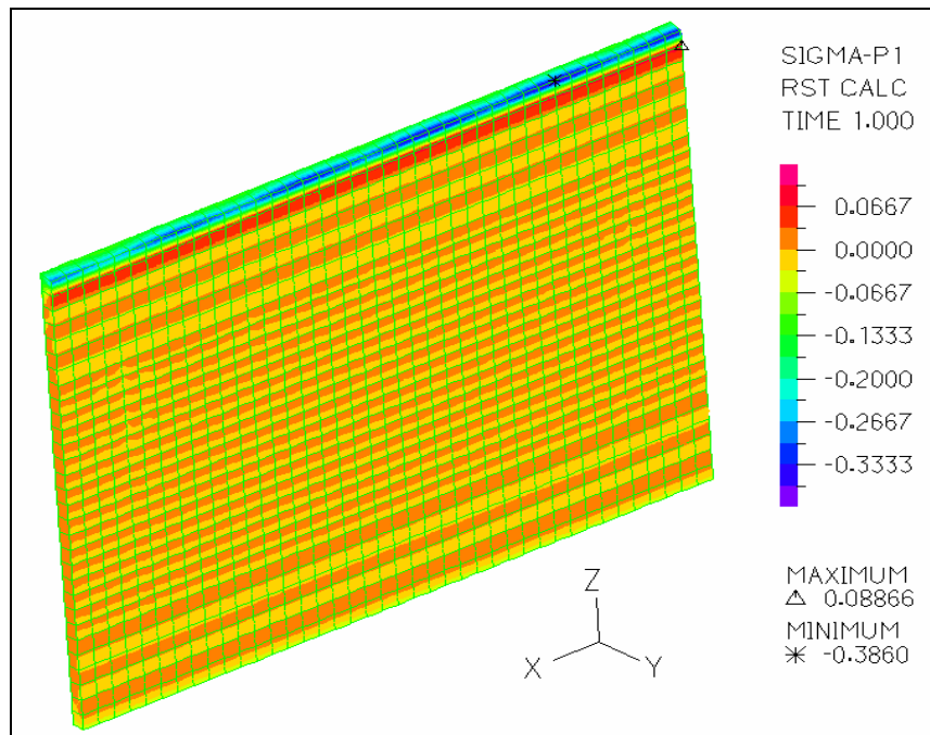
Figure 3-20: Principal Tensile Stress (Sp1) Contour Plot at the Outer Surface of the Wall – Self Weight + Post Tension Forces + Light Rail Vehicle Loads (Case 2)
