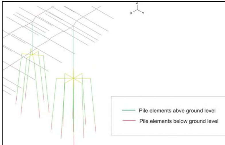
Figure 3-5: Typical Pile Group
