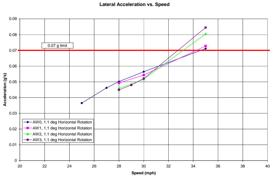
Figure 3-12: Peak Horizontal Acceleration vs. Speed, 100% Horizontal Rotation
