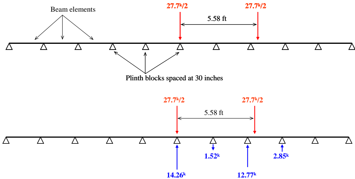
Figure 2-11: Forces acting on the Plinth Blocks under Light Rail Vehicle Loading
