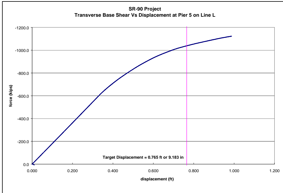
Figure 3-64: Column Force vs. Displacement at Pier 5 on Line L
