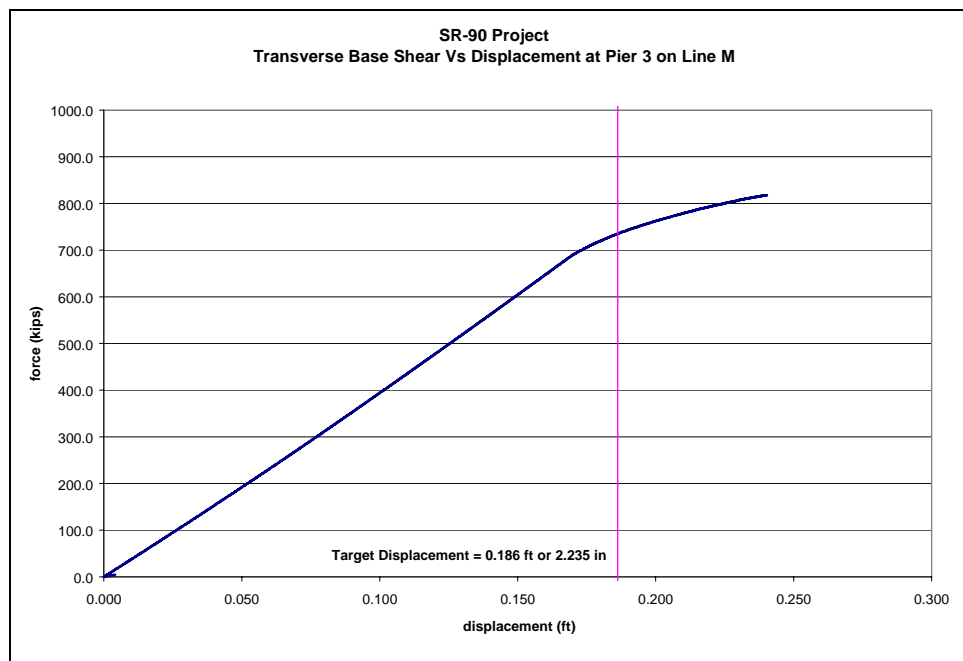
Figure 3-69: Column Force vs. Displacement at Pier 3 on Line M
