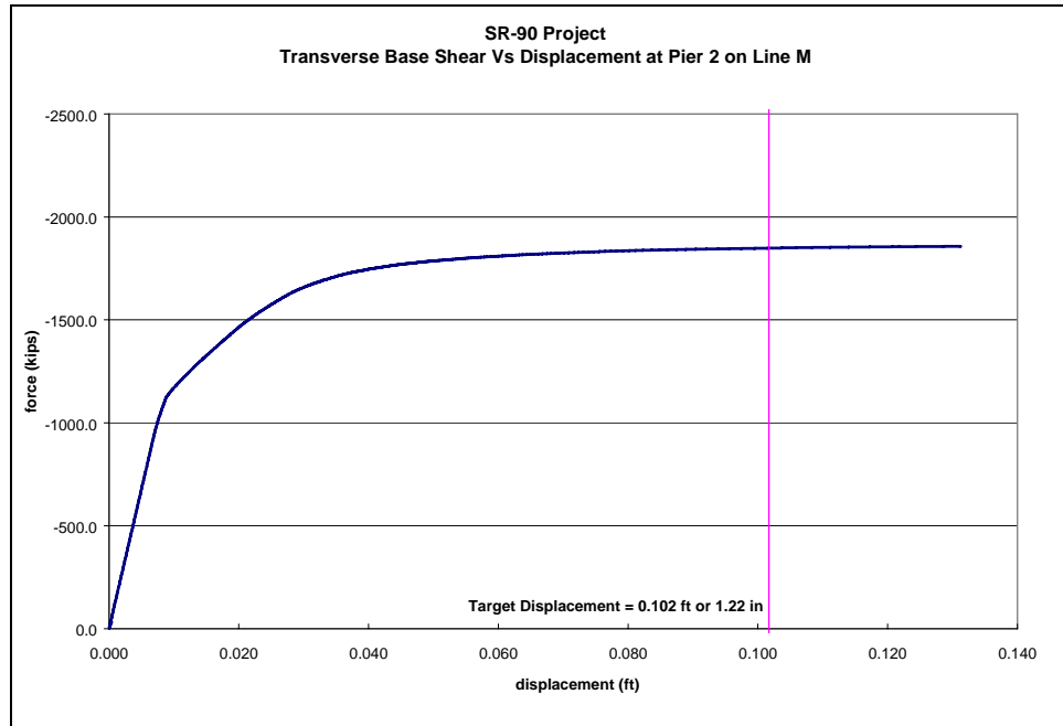
Figure 3-68: Column Force vs. Displacement at Pier 2 on Line M
