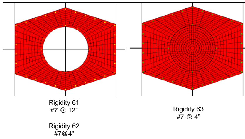
Figure 3-17: LL Pier 6 –SPEMC Model
