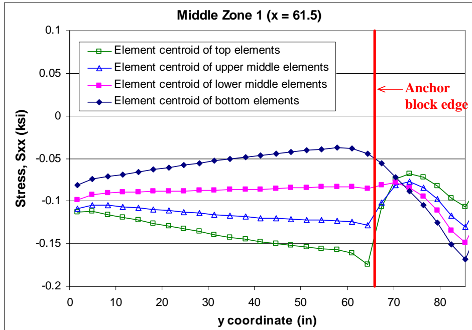
Figure 3-3: Longitudinal Stress (Sxx) Variation in the y-direction
