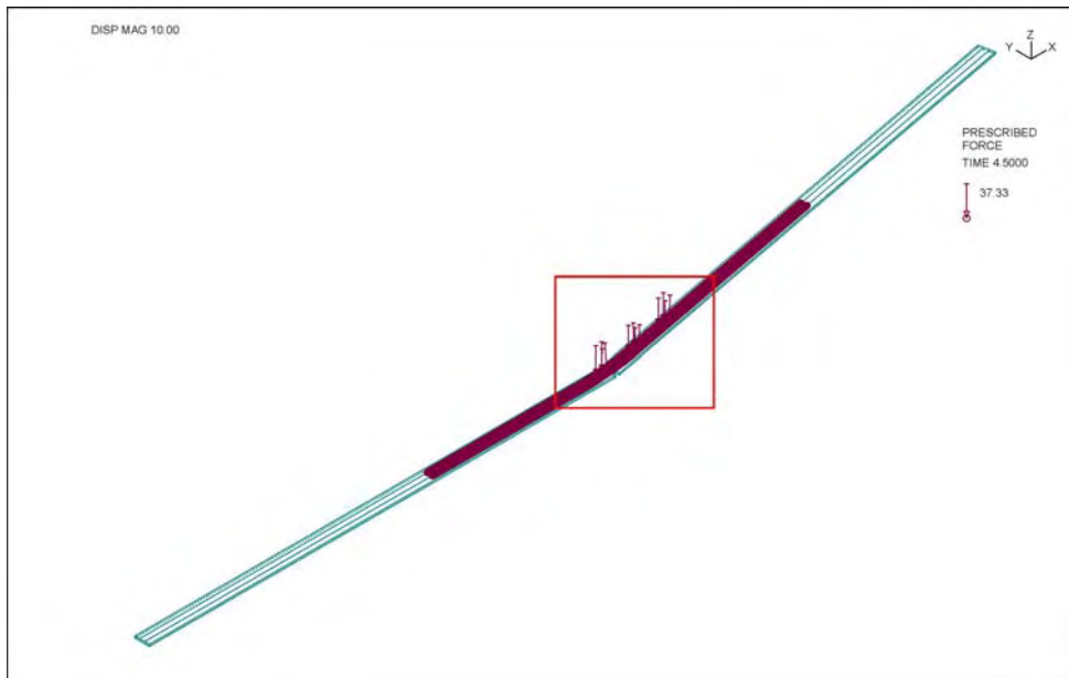
Figure 3-28: Maximum Lateral (ZZ) Rotation and Wheel Reactions.
