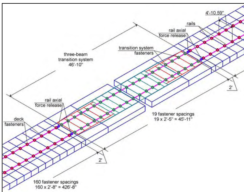
Figure 3-6: Expansion Joint Model – Rails and Fasteners – Dimensions in Feet and Inches.
