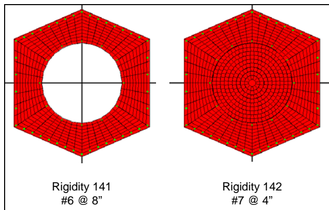
Figure 3-25: LM Pier 4 – SPERC Model
