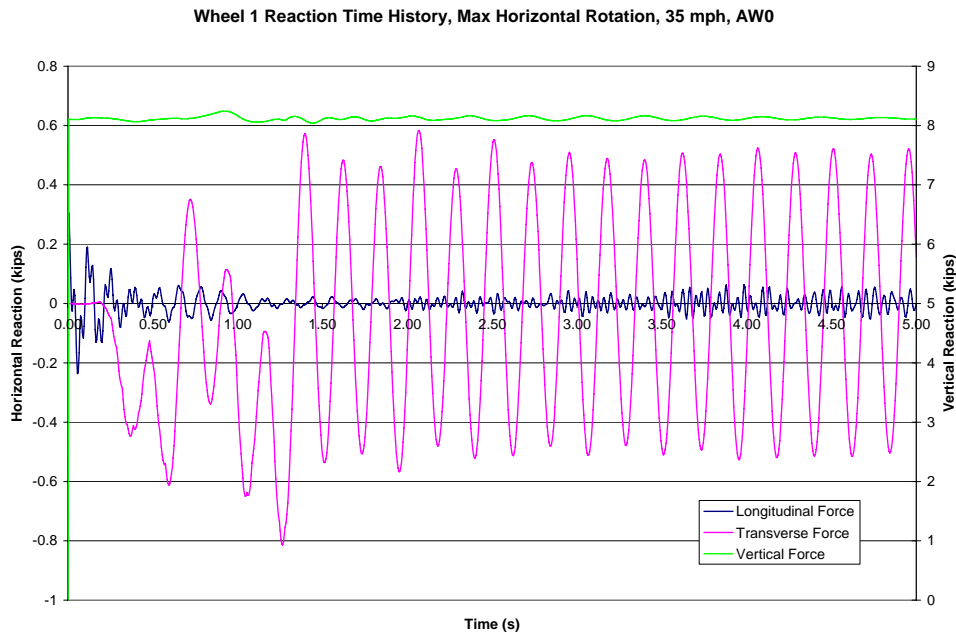
Figure 3-7: Wheel 1 Reaction, Max Horizontal Rotation, 35 MPH, Condition AW0
