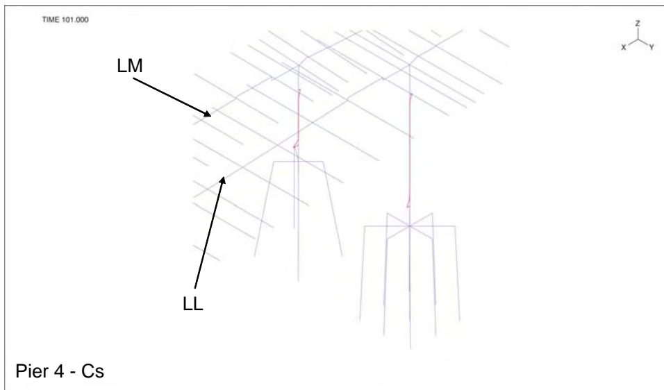
Figure 3-52: Plastic Curvature about Transverse Axis (S-axis) – Pier 4
