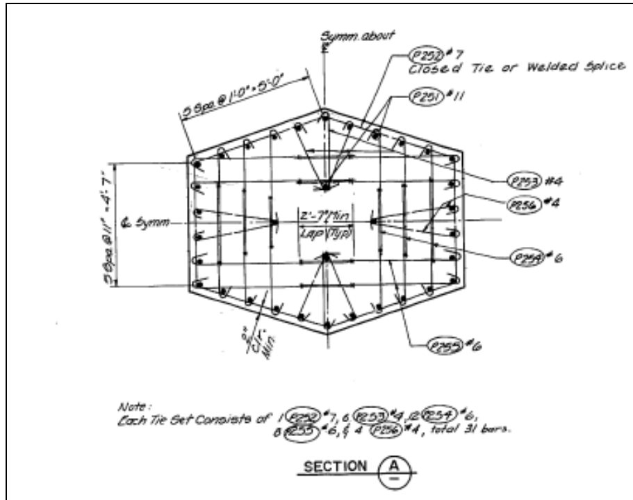
Figure 3-20: LM Pier 2 – drawing 304
