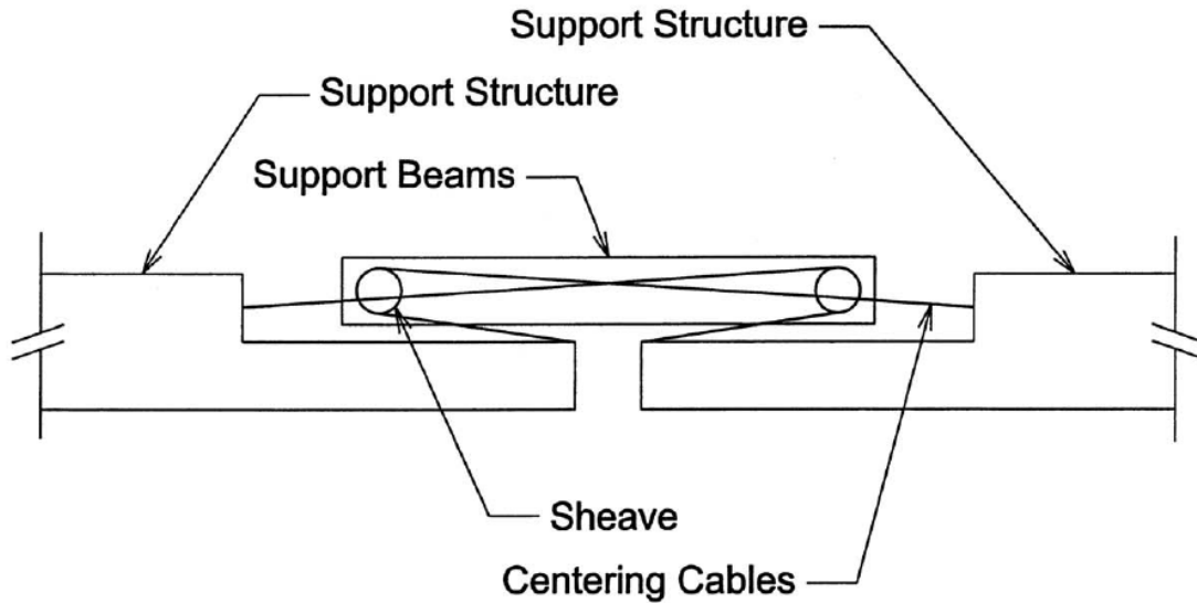
Figure 3-4: Cable System for Centering the Track Bridge (from [1])
