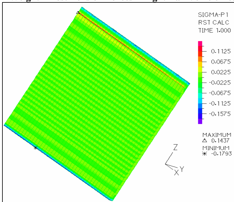
Figure 3-14: Principal Tensile Stress (Sp1) Variation in the x-direction at Deck Section 2 - Self Weight + Post Tension Forces + Light Rail Vehicle Loads (Case 2)
