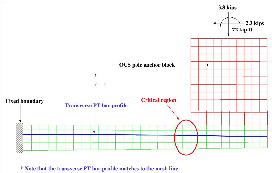
Figure 2-7: Transverse PT Bar Profile and Critical Zone Location
