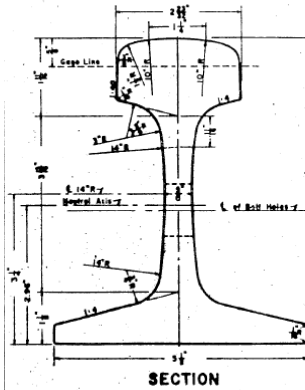
Figure 3-8: 115 LB RE Rail, Cross Section, Dimensions in Inches.
