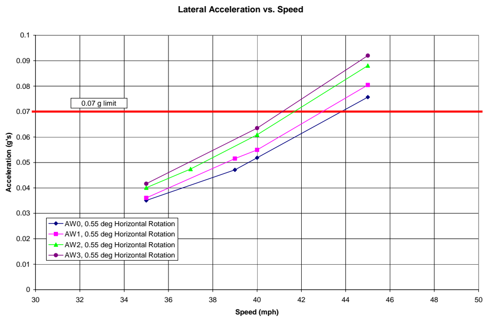
Figure 3-13: Peak Horizontal Acceleration vs. Speed, 50% Horizontal Rotation.
