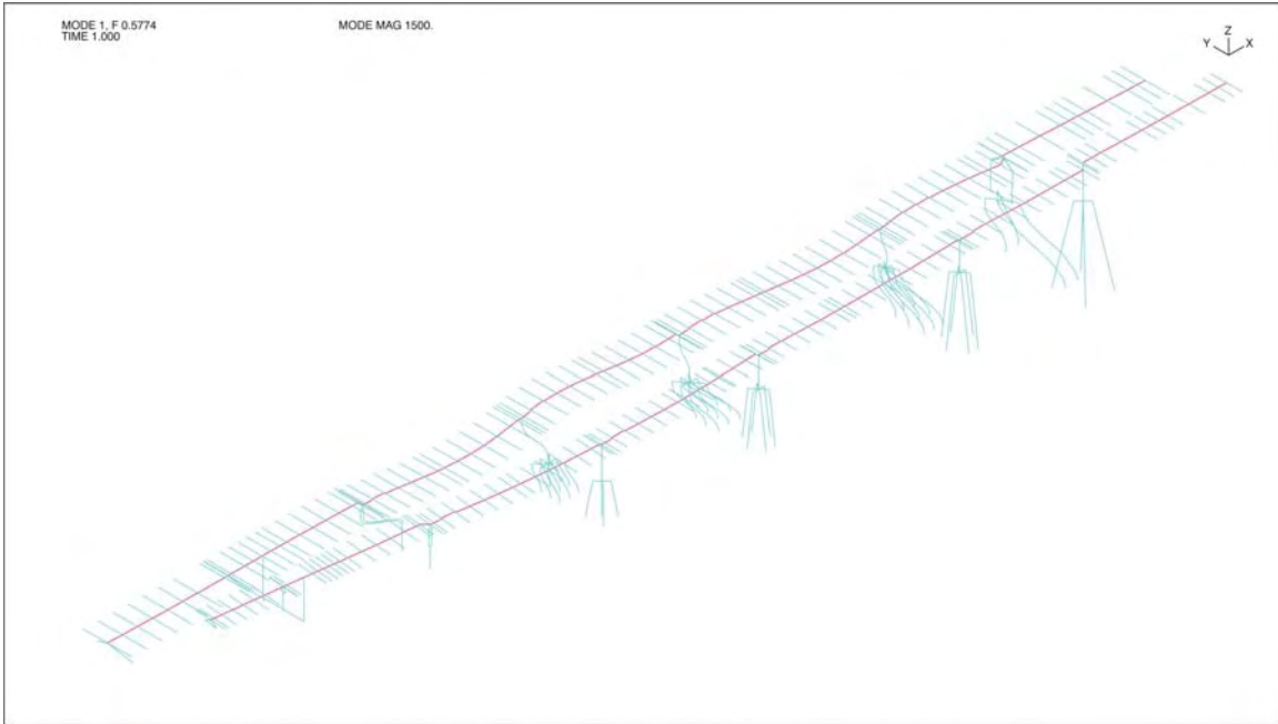
Figure 3-36: Mode Shape 1 (Longitudinal Line L – Period = 1.73)
