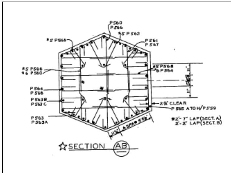
Figure 3-26: LM Pier 5 – drawing 315
