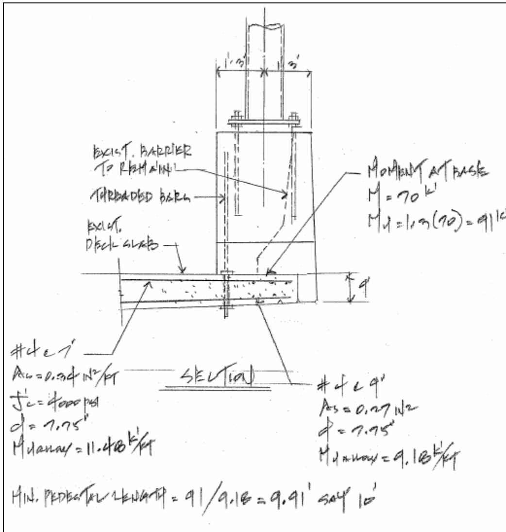
Figure 2-2: An OCS Anchor Block Design by INCA [5] Analyzed in This Study – Sectional View
