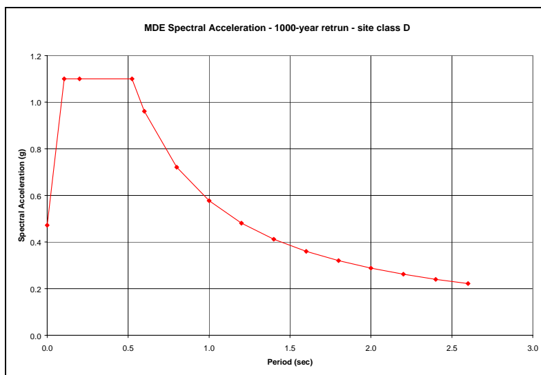
Figure 3-46: MDE Spectral Acceleration - 1000-year return - site class D
