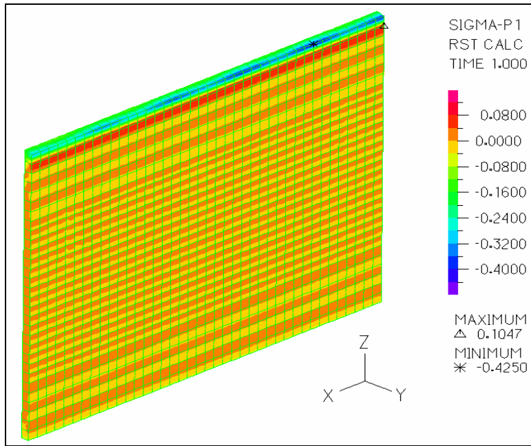
Figure 3-16: Principal Tensile Stress Contour Plot at the Outer Surface of the Wall – Self Weight +Post Tension Forces +Light Rail Vehicle Loads+OCS Loads (Case 1)
