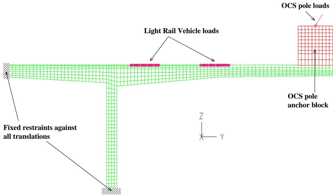
Figure 2-9: Loading and Boundary Conditions of a Cantilever Model
