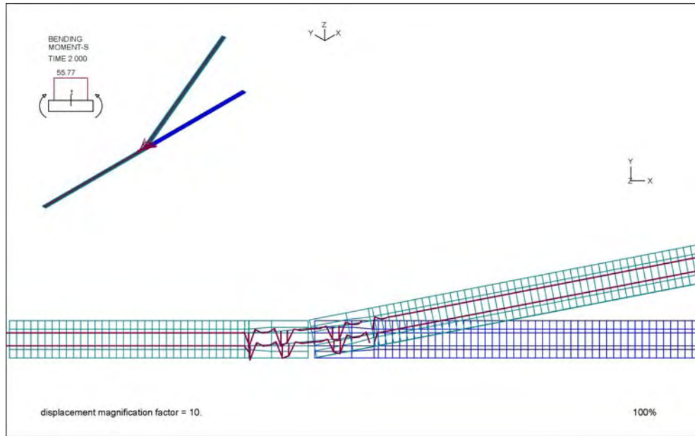
Figure 3-21: Combined Maximum Vertical (YY) and Lateral (ZZ) Rotation – Rail Bending Moment-S (about Horizontal Axis) on Deformed Mesh.
