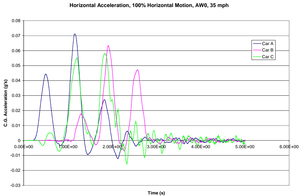
Figure 3-11: Lateral acceleration with 1.1° horizontal rotation at joint
