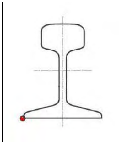
Figure 3-27: Rail Cross-Section – Point of Maximum Normal Stress
