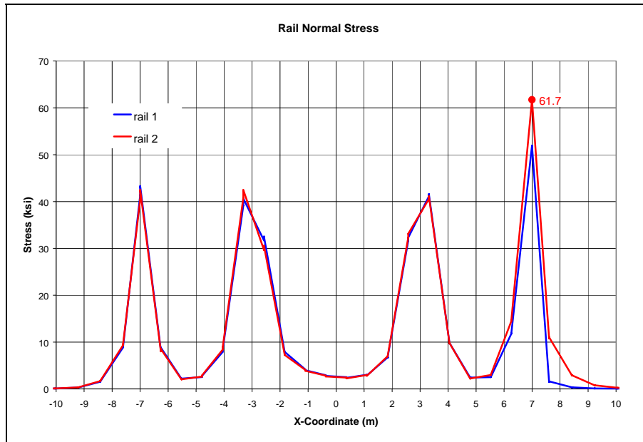
Figure 3-25: Combined Maximum Vertical (YY) and Lateral (ZZ) Rotation – Rail Normal Stress (ksi).
