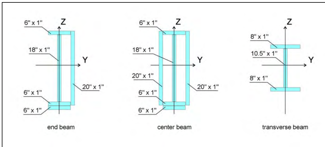
Figure 3-7: Expansion Joint Model – Three-Beam Transition System Element Cross-Sections – Dimensions in Inches.
