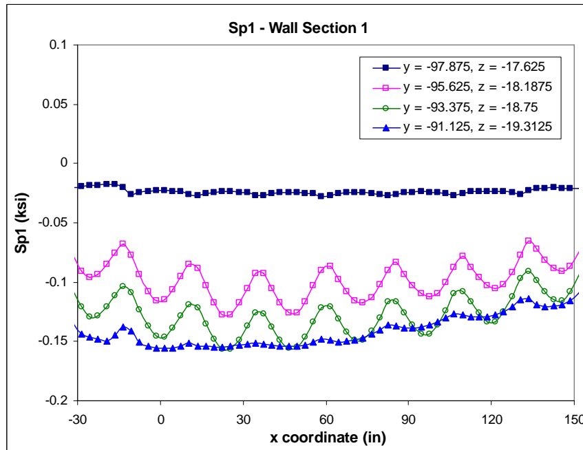
Figure 3-11: Principal Tensile Stress (Sp1) Variation in the x-direction at Wall Section 1 - Self Weight + Post Tension Forces + Light Rail Vehicle Loads (Case 2)
