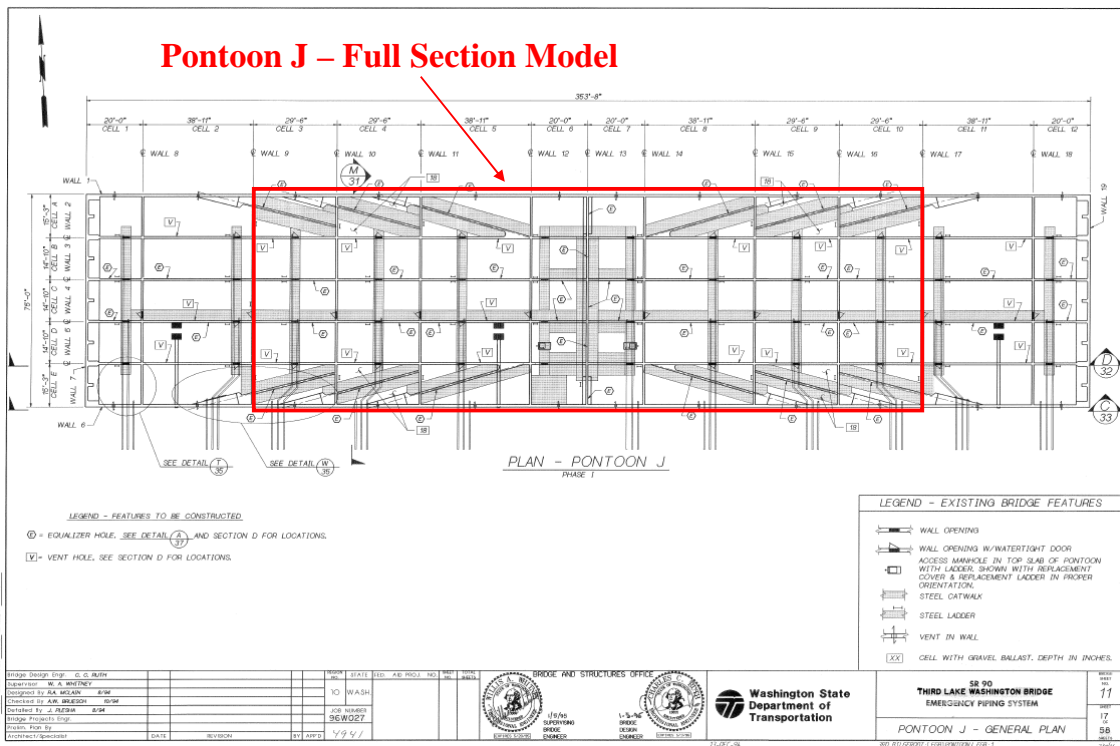
Figure 2-1: Substructure Model Boundary of a Full Section Model
