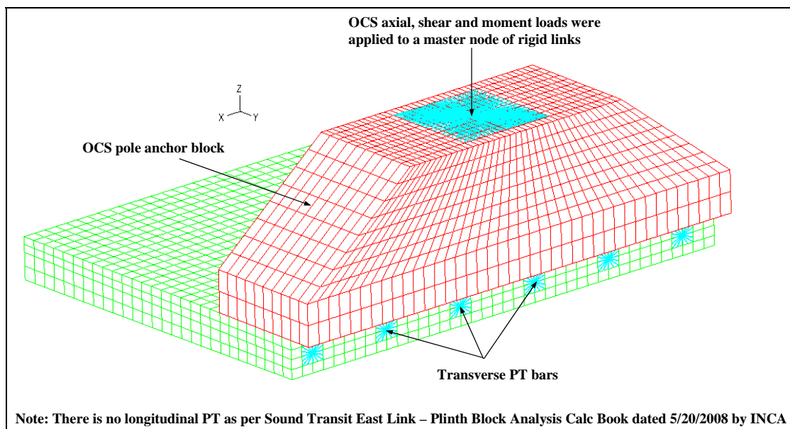
Figure 2-5: Finite Element Model for OCS Pole Analysis (7'-6" wide by 30-ft long)
