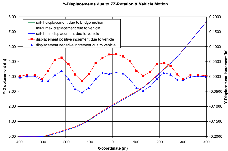
Figure 3-30: Rail Lateral (Y) Displacements due to Joint Lateral (ZZ) Rotation and Wheel Reactions.
