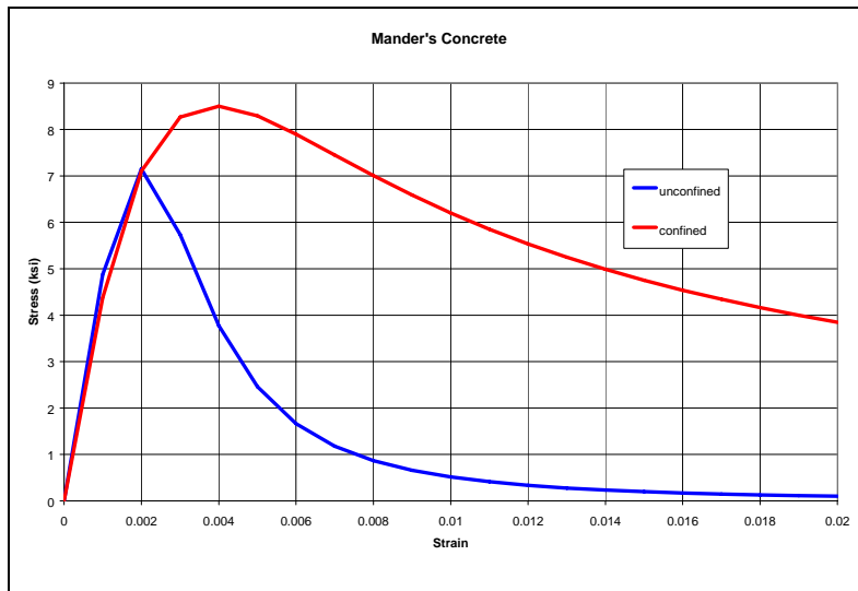
Figure 3-7: Typical Concrete Stress-Strain Relation
