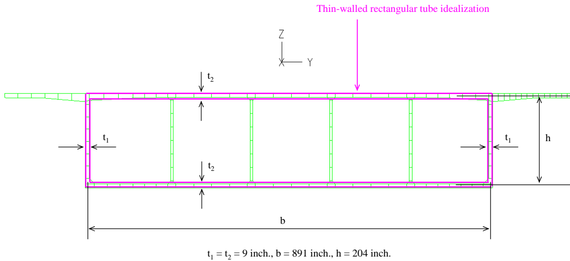
Figure 3-2: Thin-Walled Rectangular Tube Assumption of a Pontoon Full Section for a Twist Angle Prediction
