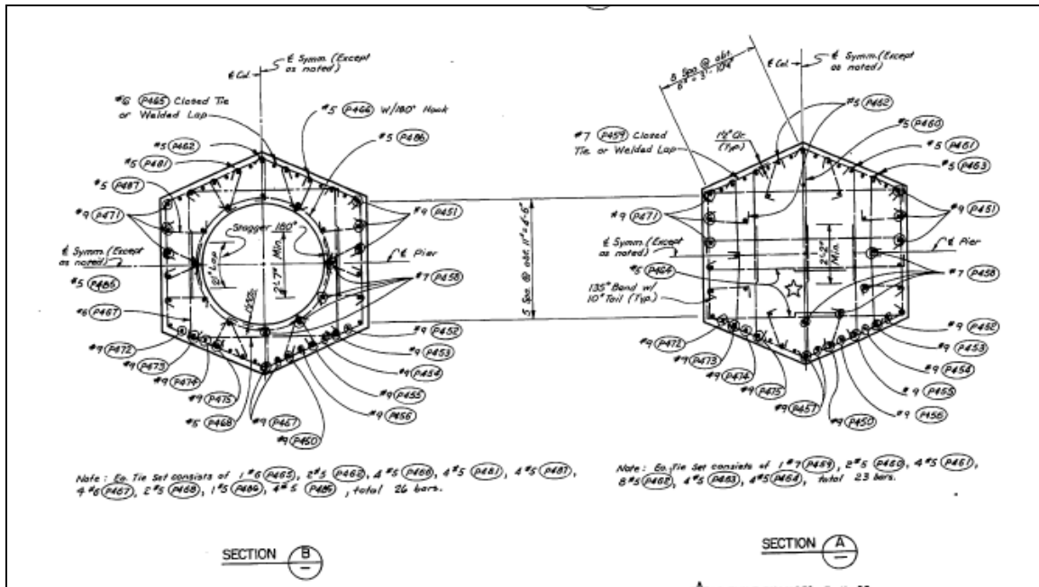
Figure 3-24: LM Pier 4 – drawing 312
