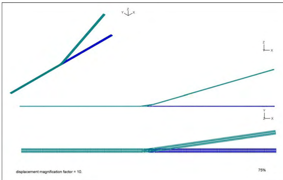
Figure 3-13: Combined 3/4 Maximum Vertical (YY) and Lateral (ZZ) Rotation – Deformed Mesh.
