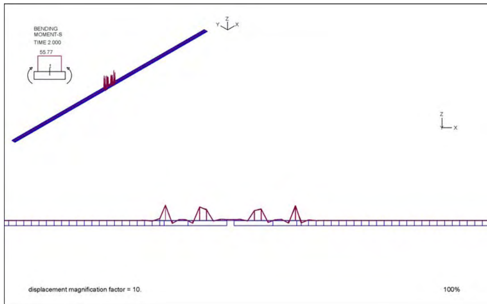
Figure 3-22: Combined Maximum Vertical (YY) and Lateral (ZZ) Rotation – Rail Bending Moment-S (about Horizontal Axis) on Original Mesh.
