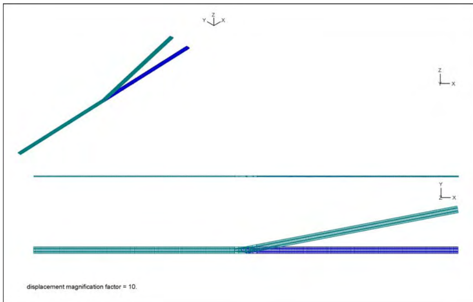
Figure 3-11: Maximum Lateral (ZZ) Rotation – Deformed Mesh.
