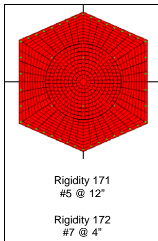
Figure 3-31: LM Pier 7 – SPEMC Model
