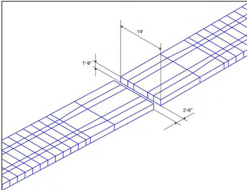
Figure 3-2: Expansion Joint Model – Span Connection Area – Dimensions in Feet and Inches.
