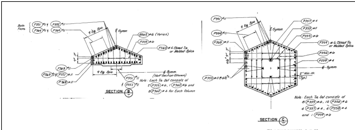
Figure 3-22: LM Pier 3 – drawing 309
