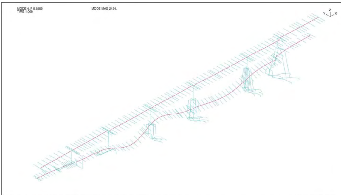
Figure 3-39: Mode Shape 4 (Longitudinal Line M -- Period = 1.17 sec)
