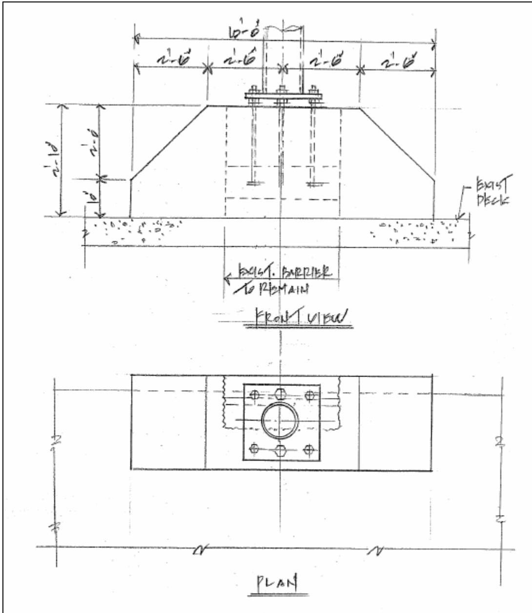
Figure 2-3: An OCS Anchor Block Design by INCA [5] Analyzed in This Study – Front View and Plan View
