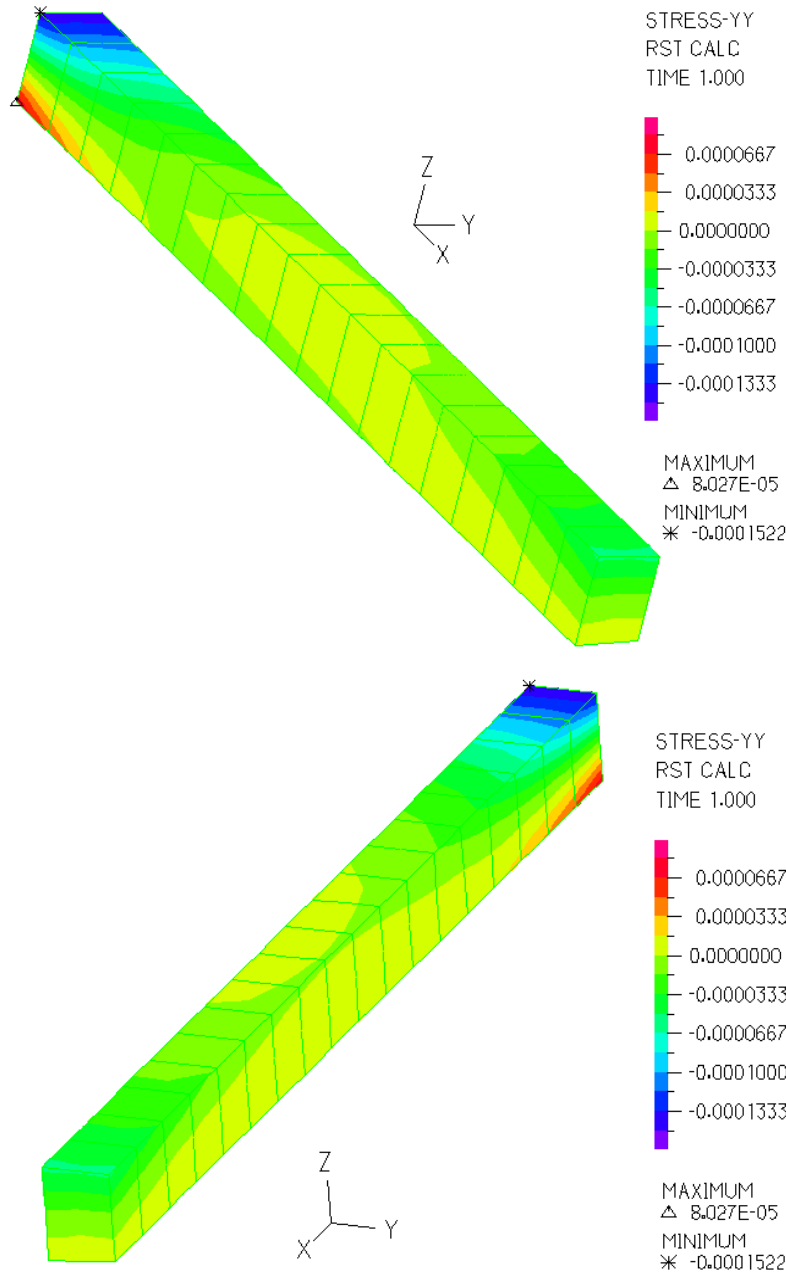
Figure 3-7: Transverse Normal Stress (Syy) Contour Plots at the Deck Element Zone 1 under a Torsion of 6202 kip-ft
