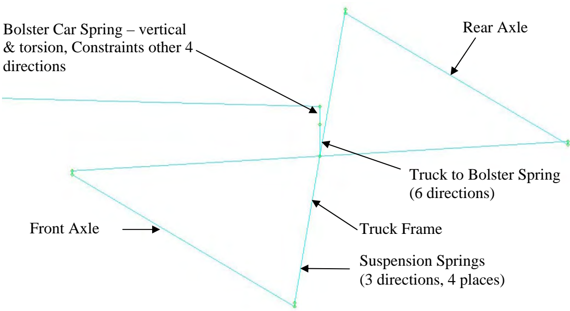
Figure 3-3: Vehicle Dynamics Model
