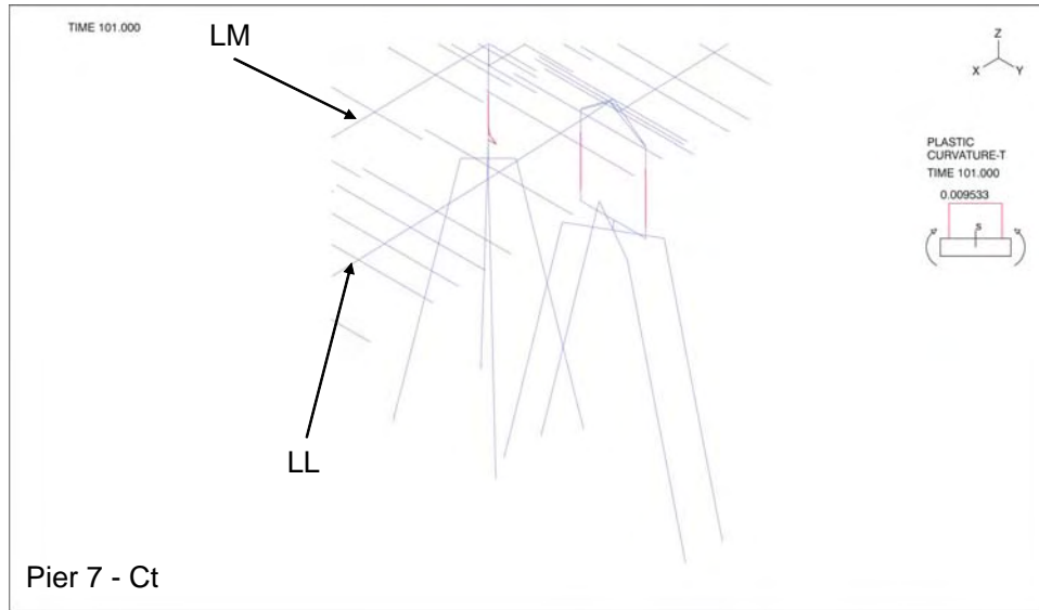
Figure 3-59: Plastic Curvature about Longitudinal Axis (T-axis) – Pier 7
