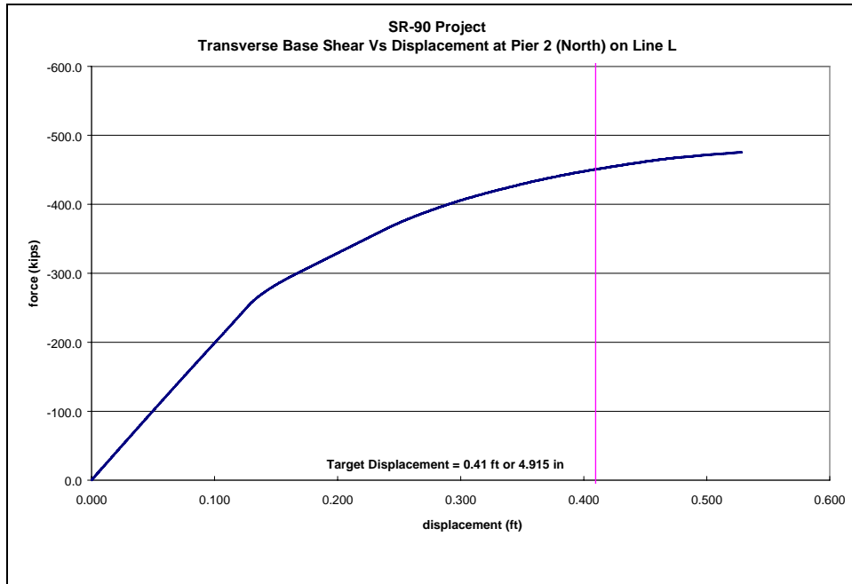
Figure 3-60: Column Force vs. Displacement at Pier 2 (North Column) on Line L
