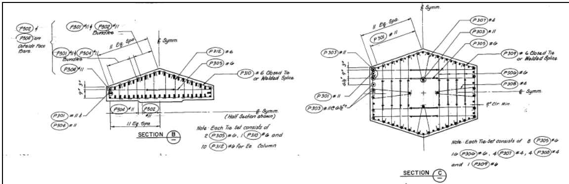
Figure 3-10: LL Pier 3 Transverse View – drawing 289
