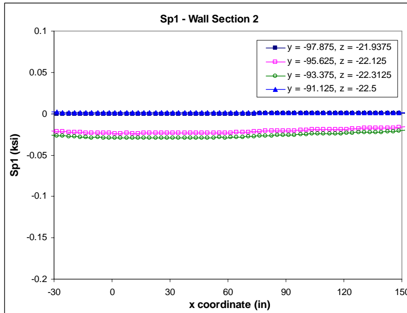
Figure 3-8: Principal Tensile Stress Variation in the x-direction at Wall Section 2- Self Weight +Post Tension Forces +Light Rail Vehicle Loads +OCS Loads (Case 1)
