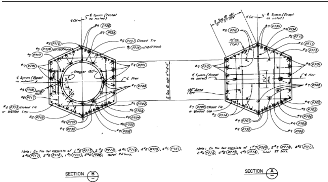
Figure 3-18: LL Pier 7 – drawing 301
