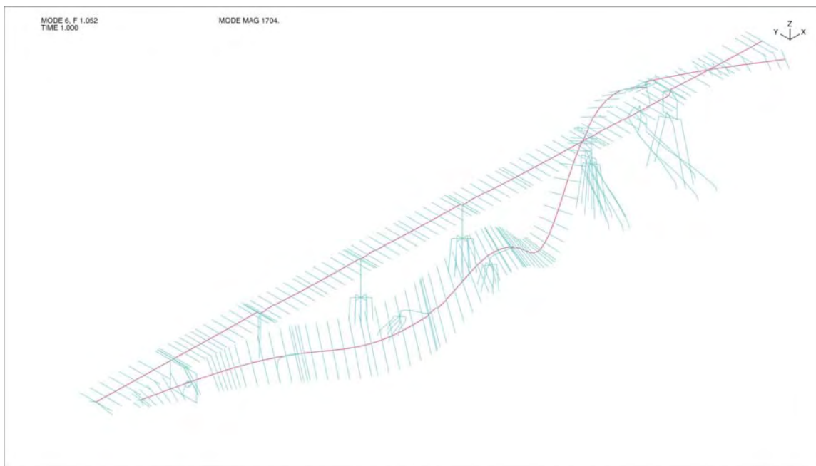
Figure 3-41: Mode Shape 6 (Vertical Line L – Period = 0.95 sec)
