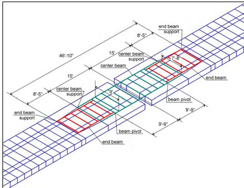
Figure 3-5: Expansion Joint Model – Three-Beam Transition System – Dimensions in Feet and Inches.
