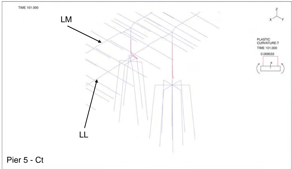
Figure 3-55: Plastic Curvature about Longitudinal Axis (T-axis) – Pier 5
