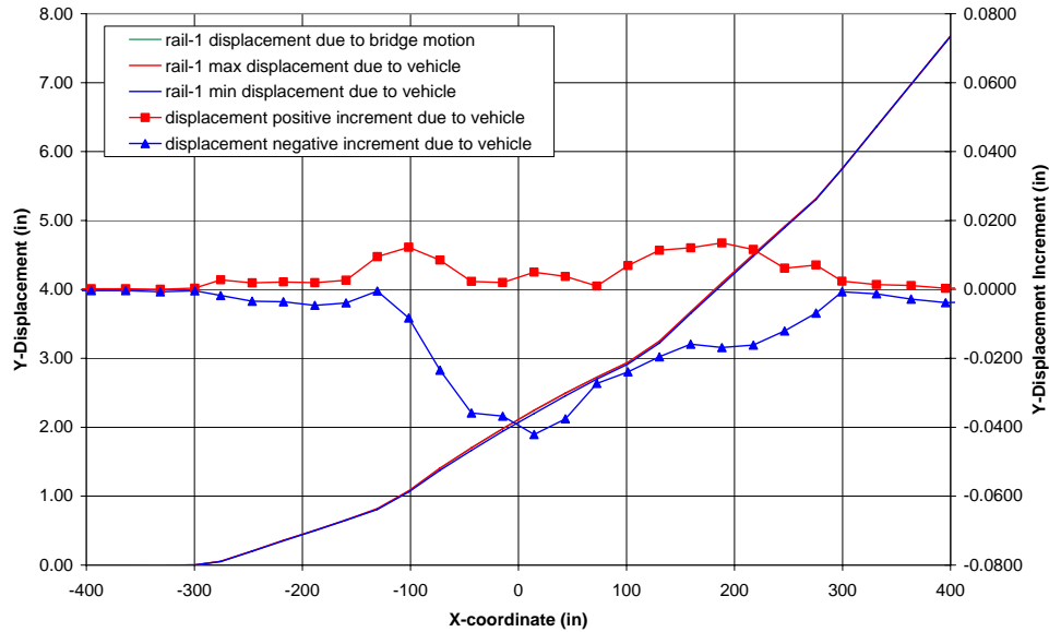
Figure 3-32: Rail Lateral (Y) Displacements due to Joint Combined Lateral (ZZ) and Vertical (YY) Rotation and Wheel Reactions.
