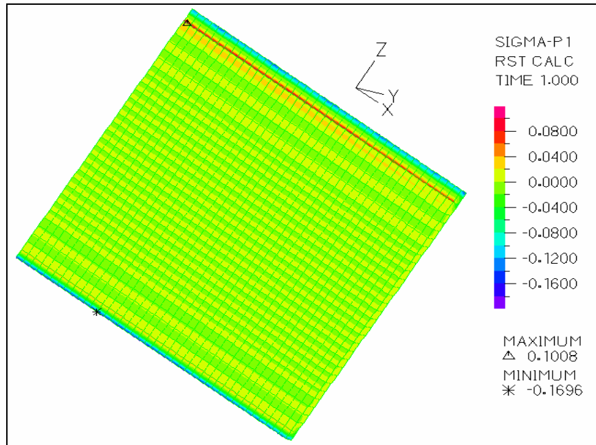
Figure 3-19: Principal Tensile Stress (Sp1) Contour Plot at the Inner Surface of the Wall – Self Weight + Post Tension Forces + Light Rail Vehicle Loads (Case 2)
