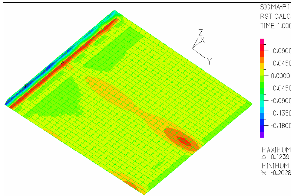
Figure 3-22: Principal Tensile Stress (Sp1) Contour Plot at the Bottom Surface of the Deck – Self Weight + Post Tension Forces + Light Rail Vehicle Loads (Case 2)
