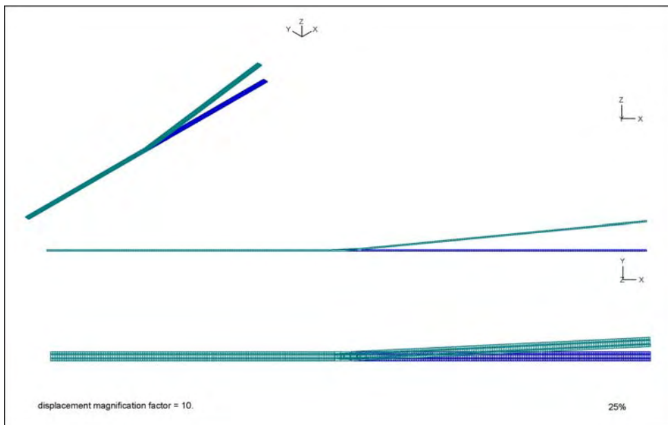
Figure 3-15: Combined 1/4 Maximum Vertical (YY) and Lateral (ZZ) Rotation – Deformed Mesh.
