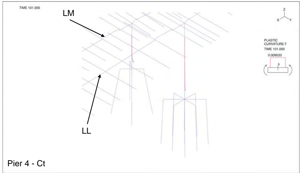
Figure 3-53: Plastic Curvature about Longitudinal Axis (T-axis) – Pier 4
