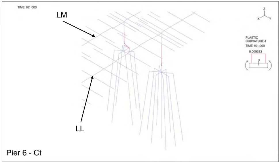
Figure 3-57: Plastic Curvature about Longitudinal Axis (T-axis) – Pier 6
