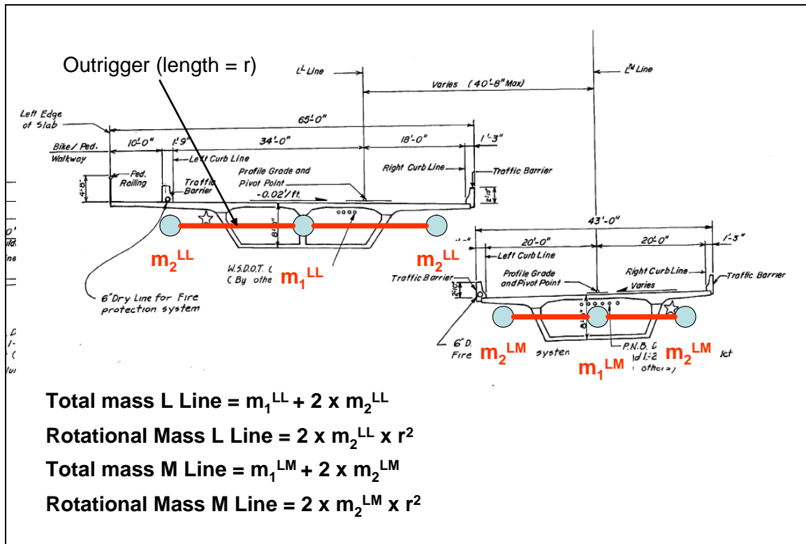
Figure 3-4: Modeling of the Superstructures of Lines L and M
