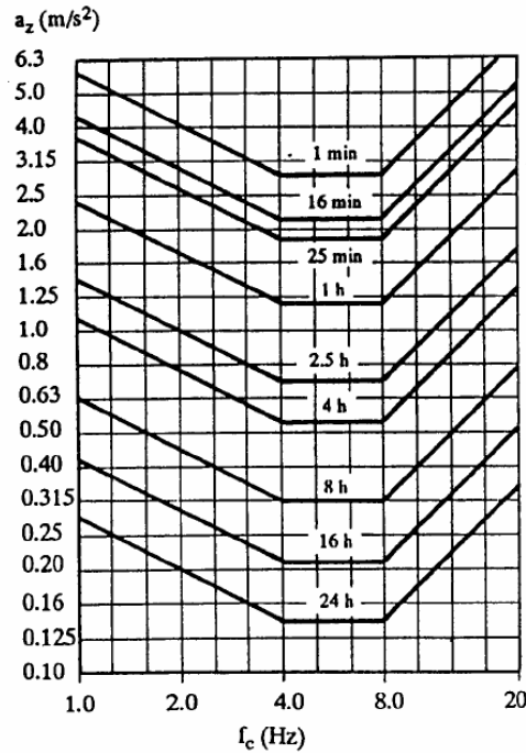
Figure 3-8: Vertical Acceleration Limits
