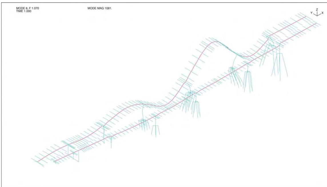
Figure 3-43: Mode Shape 8 (Torsion-Transverse Line M – Period = 0.93 sec)
