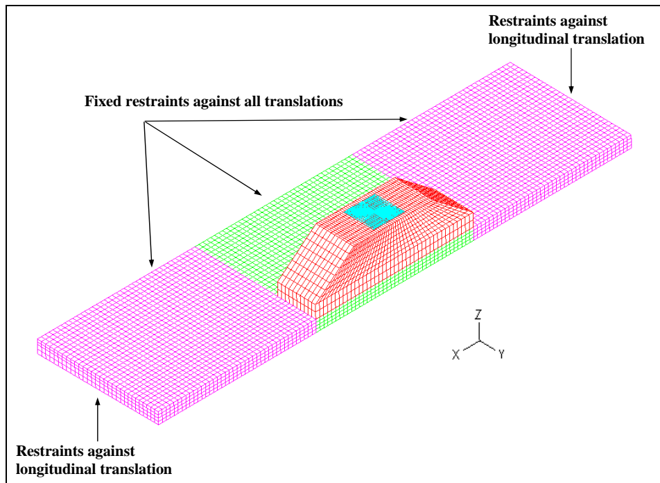
Figure 2-5: Finite Element Model for OCS Pole Analysis (7'-6" wide by 30-ft long)
