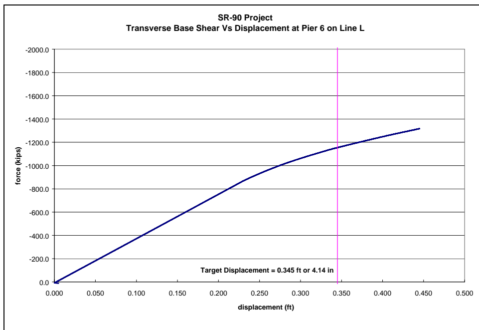
Figure 3-65: Column Force vs. Displacement at Pier 6 on Line L
