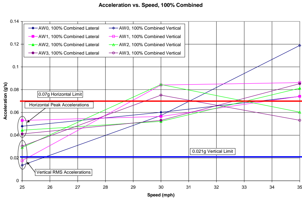
Figure 3-16: RMS Vertical and Peak Horizontal Acceleration with 2.2° Vertical and 1.1° Horizontal Rotation at Joint.
