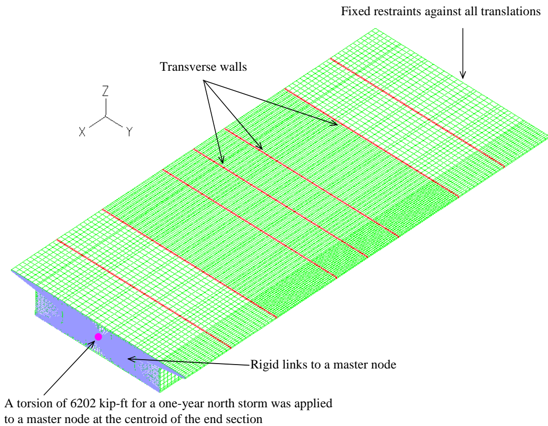
Figure 2-2: Loading and Boundary Conditions of a Full Section Model
