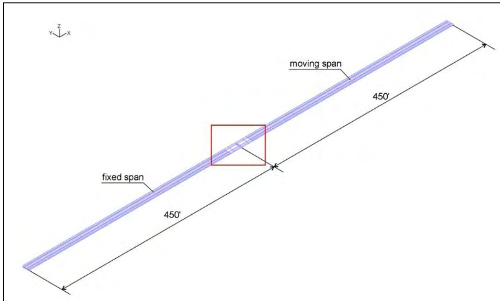
Figure 3-1: Expansion Joint Model – Total View – Dimensions in Feet.
