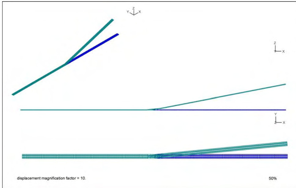
Figure 3-14: Combined 1/2 Maximum Vertical (YY) and Lateral (ZZ) Rotation – Deformed Mesh.
