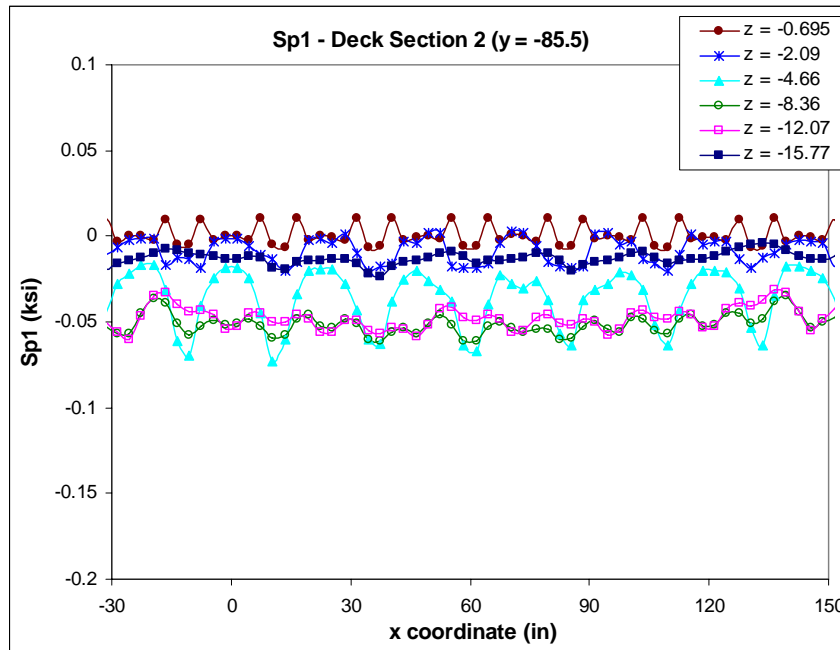
Figure 3-14: Principal Tensile Stress (Sp1) Variation in the x-direction at Deck Section 2 - Self Weight + Post Tension Forces + Light Rail Vehicle Loads (Case 2)
