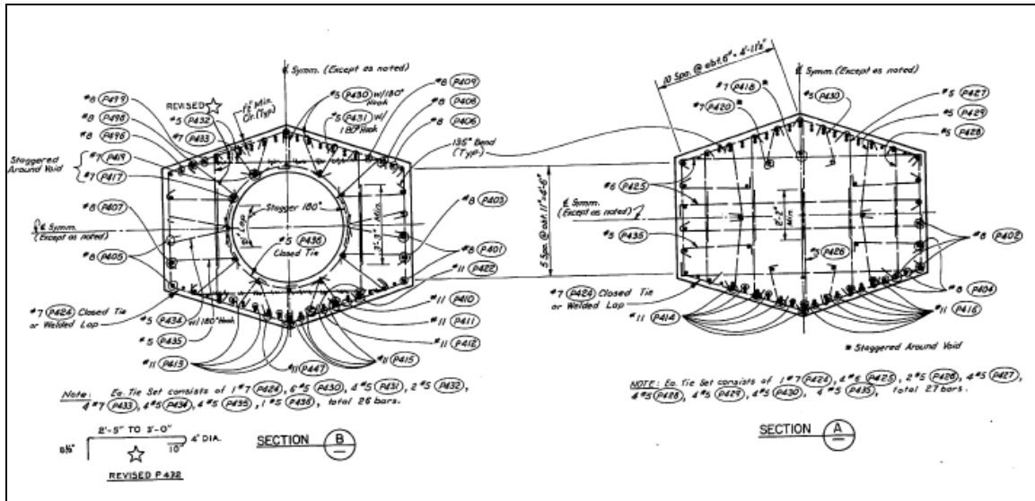
Figure 3-12: LL Pier 4 Column Reinforcement - drawing 292
