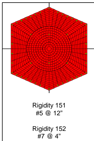
Figure 3-29: LM Pier 6 – SPEMC Model (identical to Pier 5 LM)
