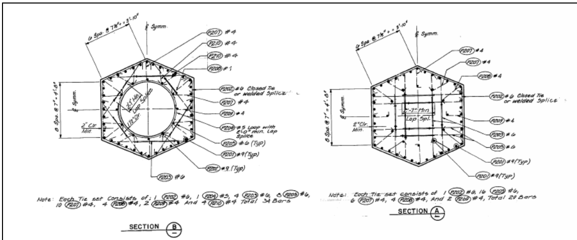
Figure 3-8: LL Pier 2 - drawing 286
