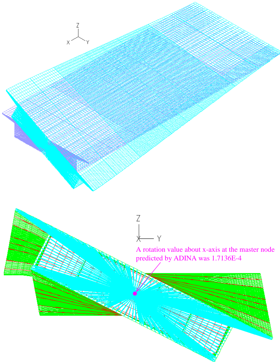
Figure 3-1: Deformed Shape of a Full Section Model under a Torsion of 6202 kip-ft
