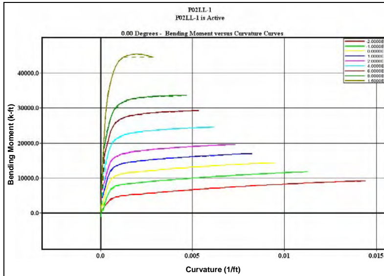
Figure 3-32 Typical Moment-Curvature Relation of Piers
