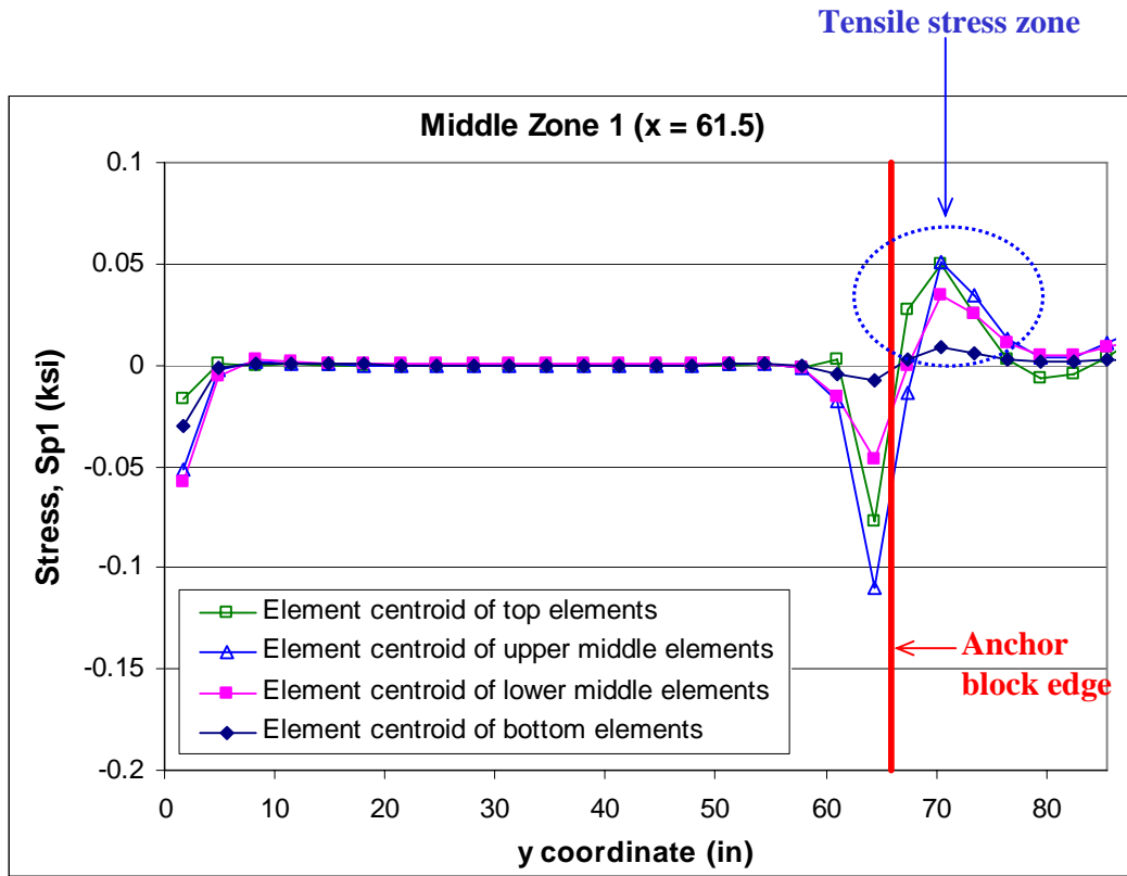
Figure 3-4: Principal Tensile Stress (Sp1) Variation in the y-direction
