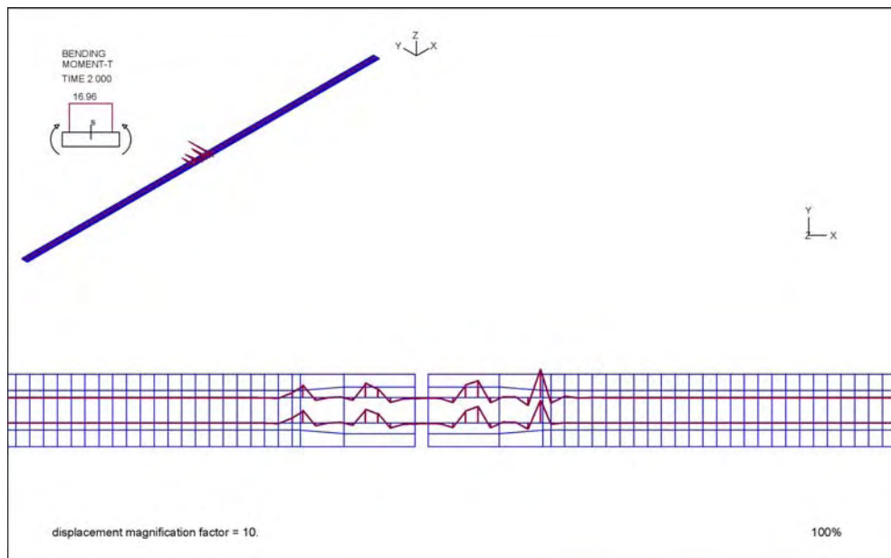
Figure 3-24: Combined Maximum Vertical (YY) and Lateral (ZZ) Rotation – Rail Bending Moment-T (about Vertical Axis) on Original Mesh.
