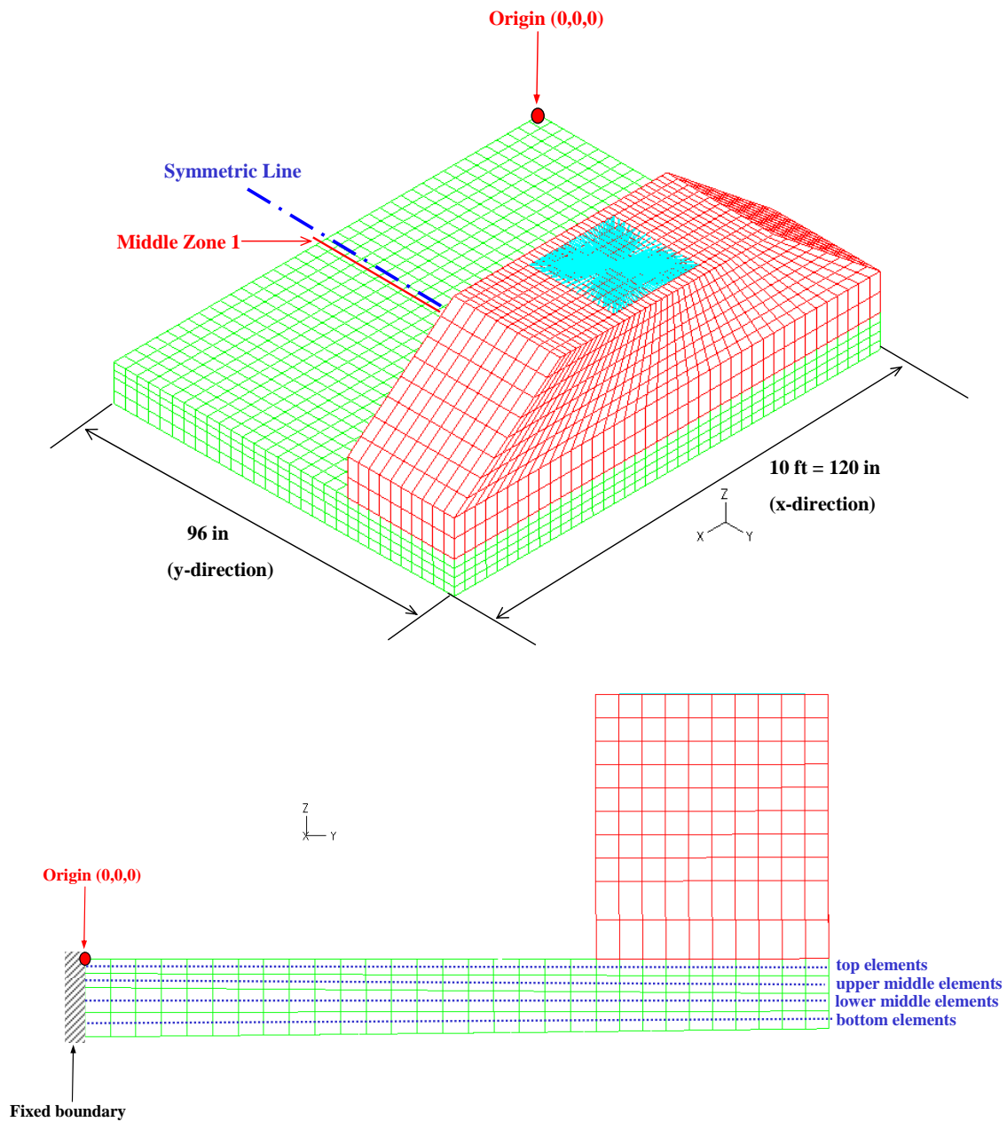
Figure 3-1: Middle Zone Location selected for the Investigation of Stress Variation in the y-direction (x = 61.5)
