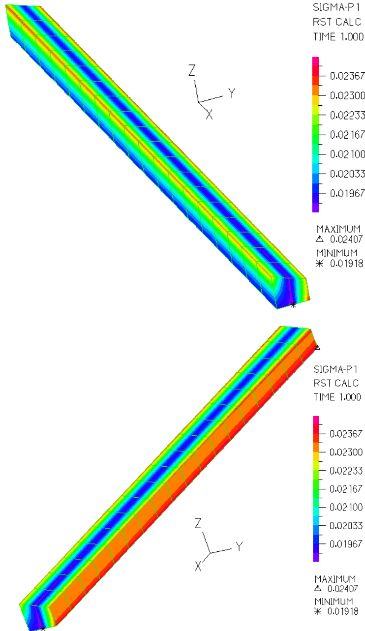
Figure 3-8: Principal Tensile Stress (Sp1) Contour Plots at the Wall Element Zone 1 under a Torsion of 6202 kip-ft
