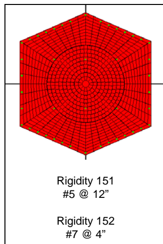
Figure 3-27: LM Pier 5 – SPEMC Model
