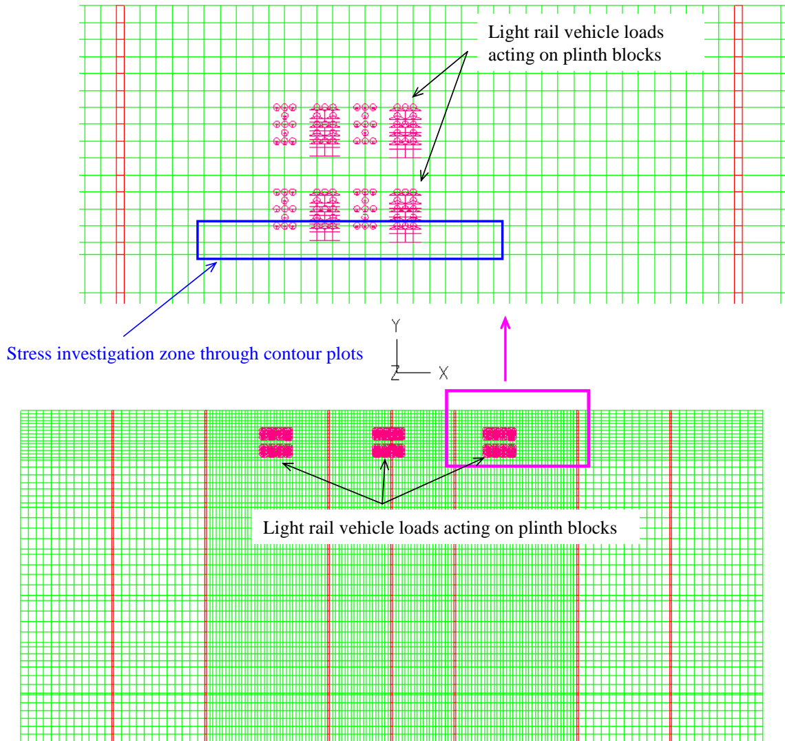
Figure 3-4: Critical Zones selected for Stress Investigation – Plan View
