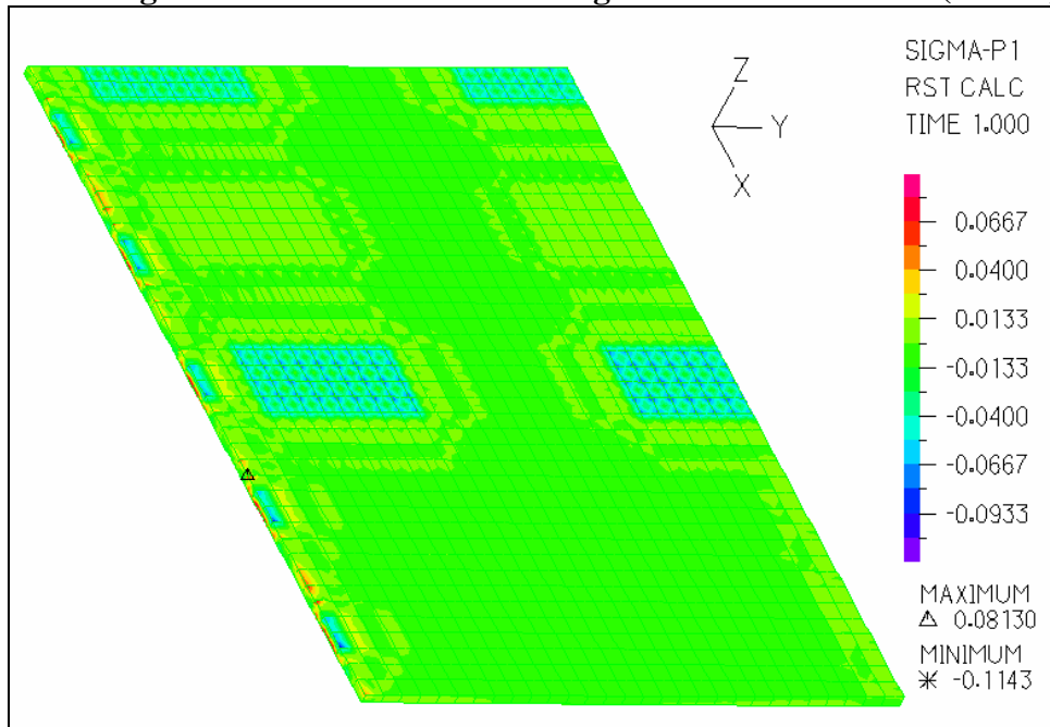
Figure 3-20: Principal Tensile Stress (Sp1) Contour Plot at the Outer Surface of the Wall – Self Weight + Post Tension Forces + Light Rail Vehicle Loads (Case 2)
