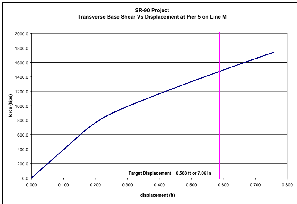
Figure 3-71: Column Force vs. Displacement at Pier 5 on Line M
