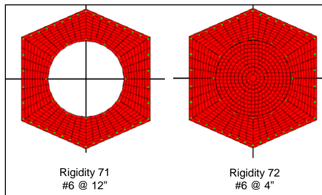
Figure 3-19: LL Pier 7 – SPEMC Model
