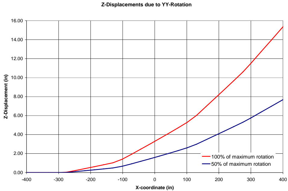
Figure 3-17: Rail Vertical (Z) Displacements due to Joint Vertical (YY) Rotation.
