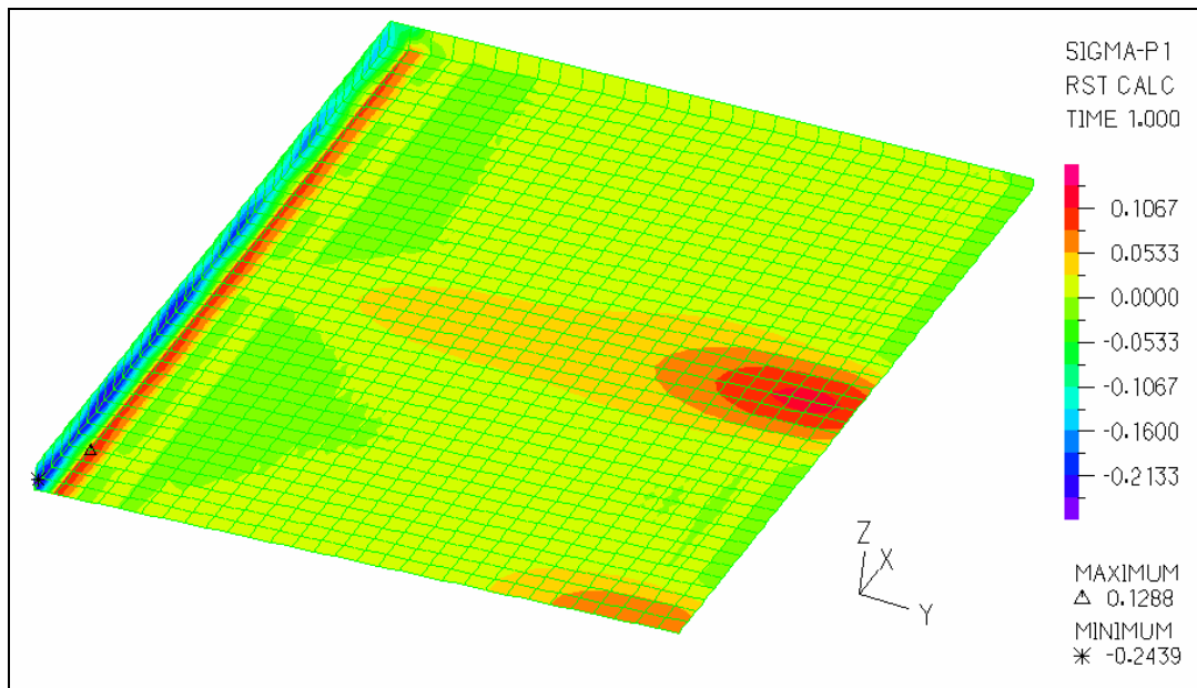
Figure 3-17: Principal Tensile Stress Contour Plot at the Top Surface of the Deck – Self Weight + Post Tension Forces + Light Rail Vehicle Loads +OCS Loads (Case 1)
