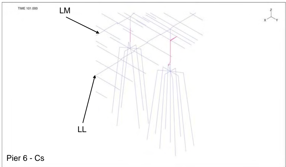
Figure 3-56: Plastic Curvature about Transverse Axis (S-axis) – Pier 6
