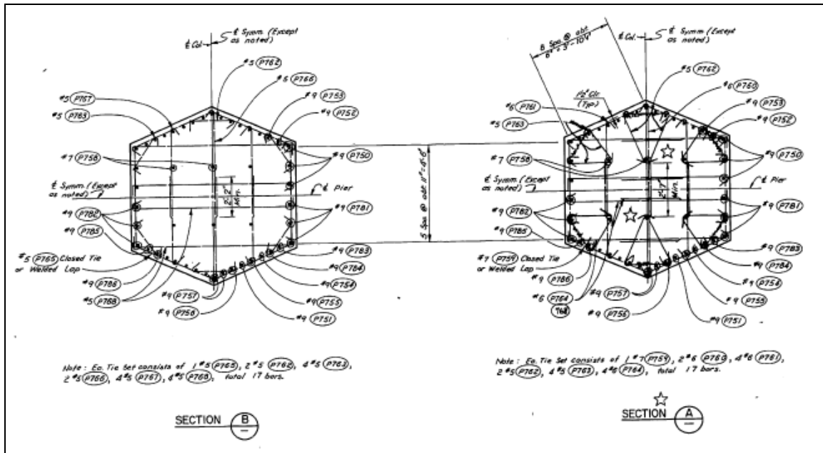
Figure 3-30: LM Pier 7 – drawing 321
