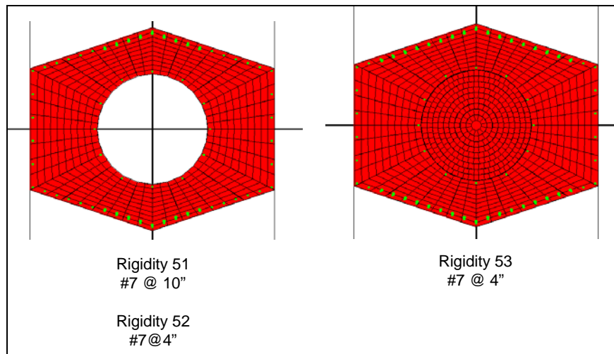
Figure 3-15: LL Pier 5 – SPEMC Model
