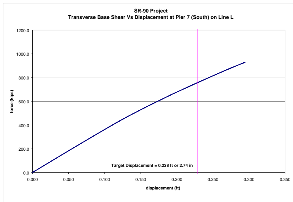
Figure 3-67: Column Force vs. Displacement at Pier 7 (South Column) on Line L
