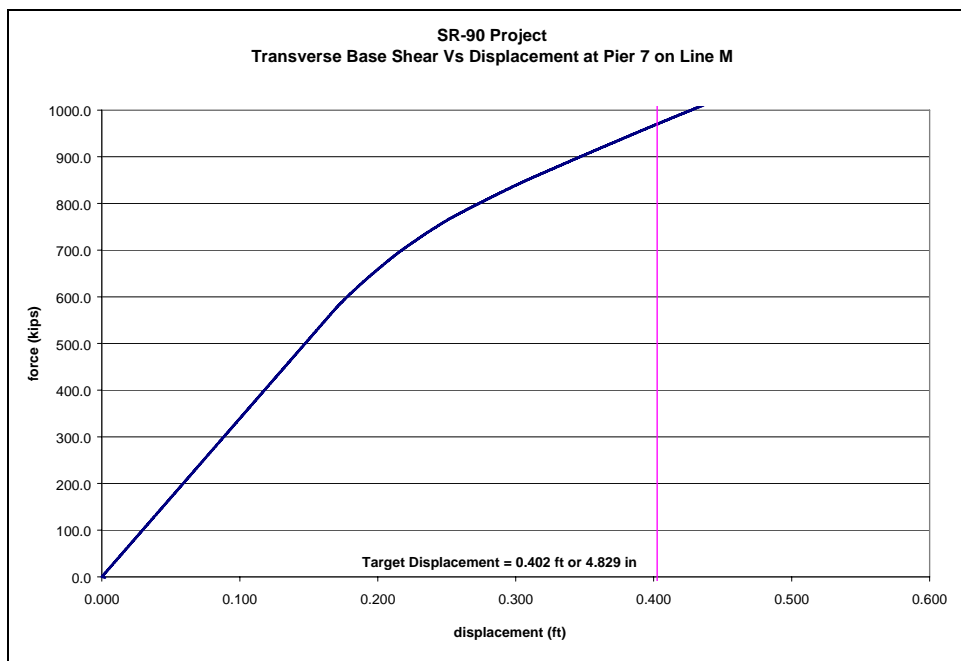
Figure 3-73: Column Force vs. Displacement at Pier 7 on Line M
