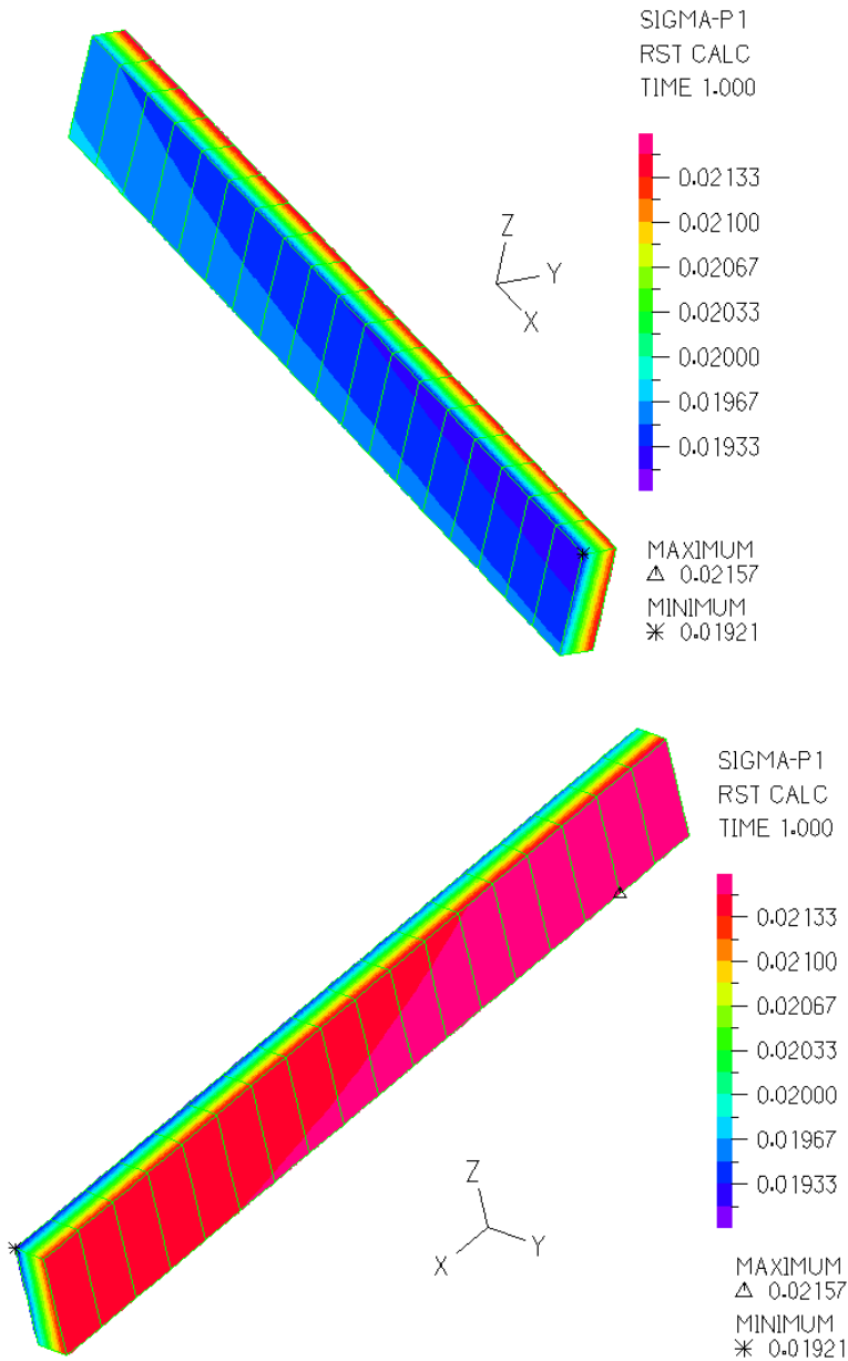
Figure 3-10: Principal Tensile Stress (Sp1) Contour Plots at the Wall Element Zone 2 under a Torsion of 6202 kip-ft
