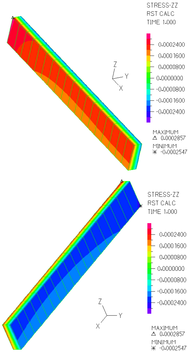
Figure 3-11: Vertical Normal Stress ( S_{zz} ) Contour Plots at the Wall Element Zone 2 under a Torsion of 6202 kip-ft
