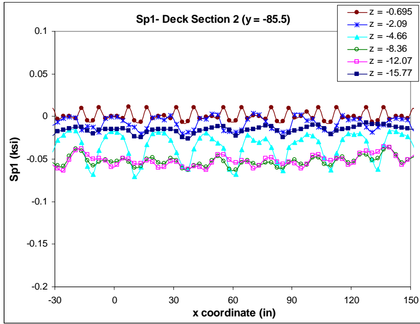
Figure 3-10: Principal Tensile Stress Variation in the x-direction at Deck Section 2 - Self Weight +Post Tension Forces +Light Rail Vehicle Loads +OCS Loads (Case 1)
