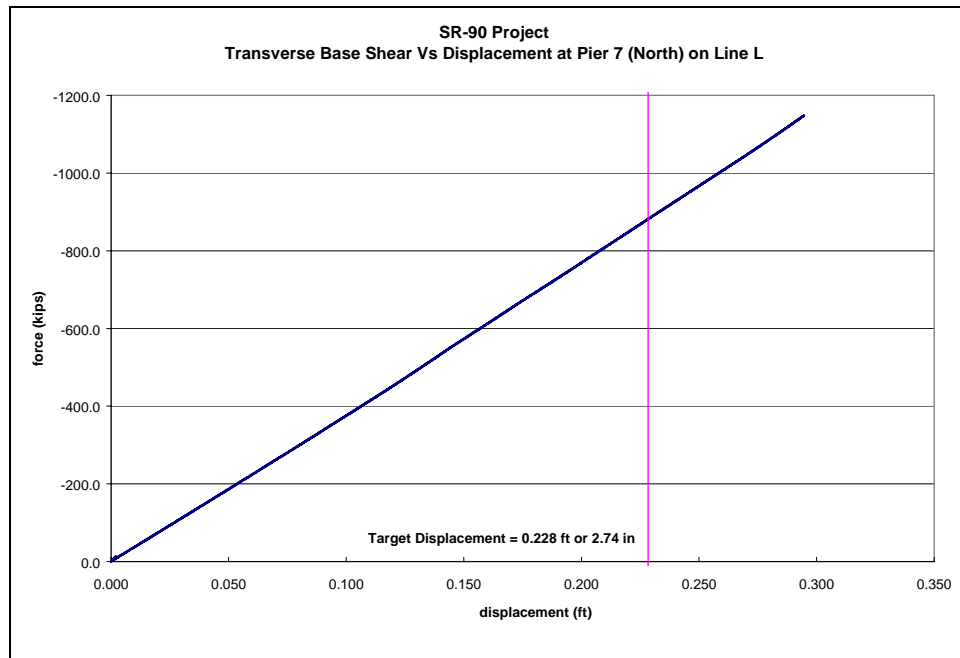
Figure 3-66: Column Force vs. Displacement at Pier 7 (North Column) on Line L
