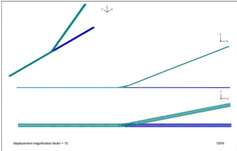
Figure 3-12: Combined Maximum Vertical (YY) and Lateral (ZZ) Rotation – Deformed Mesh.
