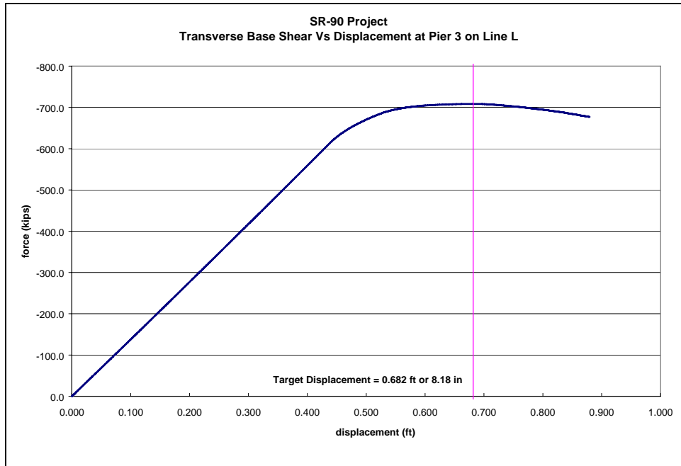
Figure 3-62: Column Force vs. Displacement at Pier 3 on Line L
