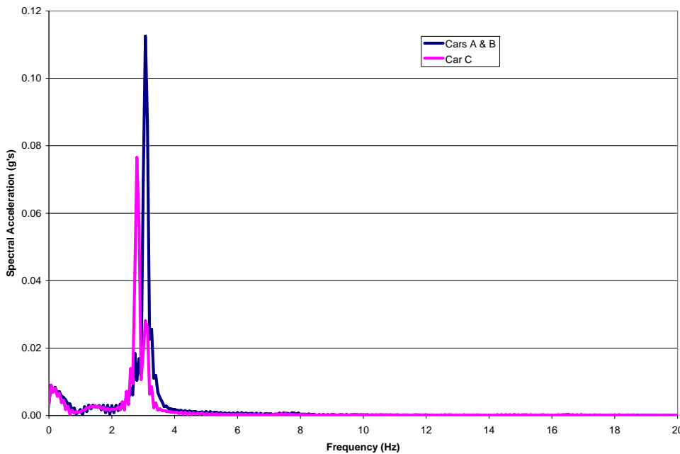
Figure 3-10: Vertical Spectral Acceleration, 35 mph, AW0
