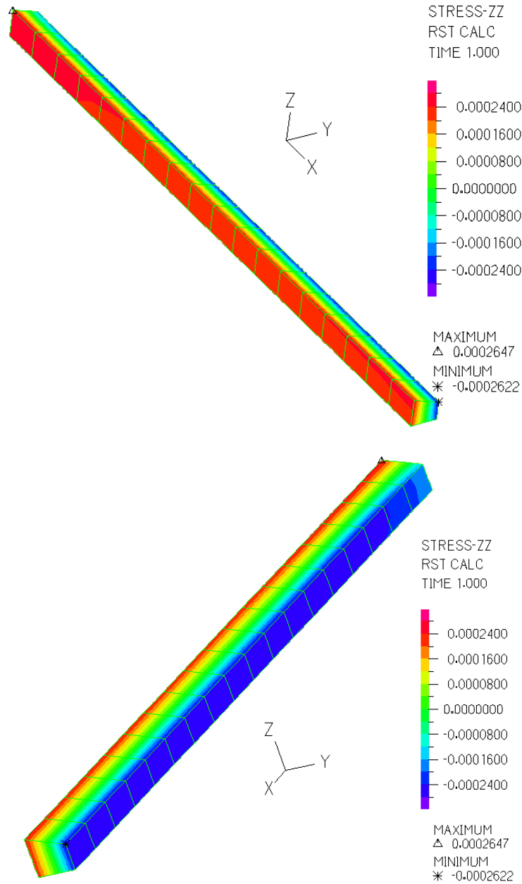
Figure 3-9: Vertical Normal Stress (Szz) Contour Plots at the Wall Element Zone 1 under a Torsion of 6202 kip-ft
