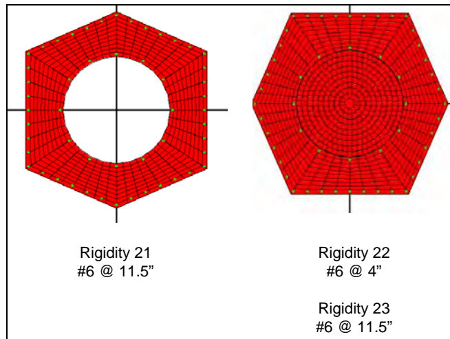
Figure 3-9: LL Pier 2 SPEMC Model
