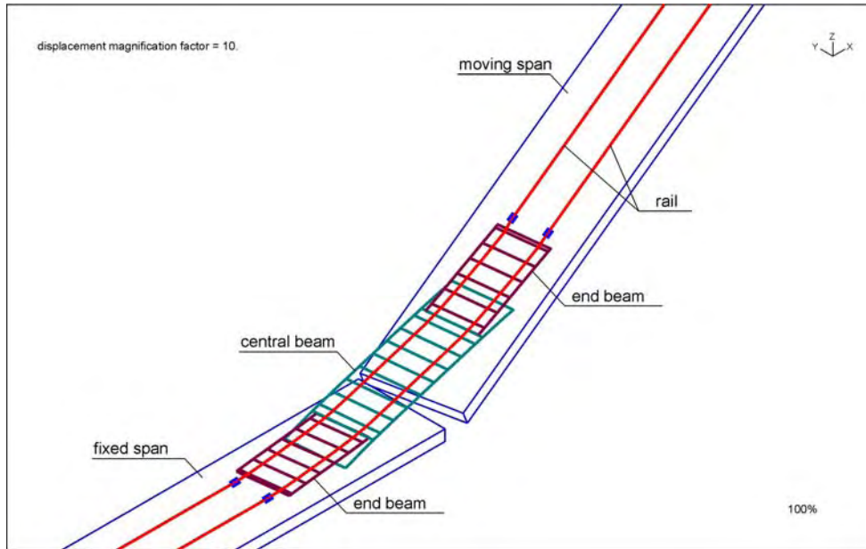
Figure 3-19: Deformed Expansion Joint Model Details.
