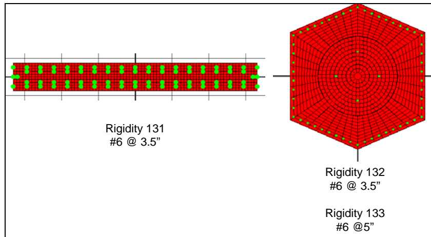
Figure 3-23: LM Pier 3 – SPEMC Model
