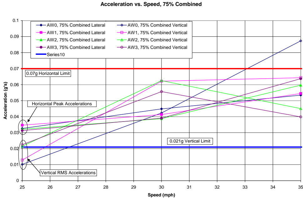
Figure 3-17: RMS Vertical and Peak Horizontal Acceleration with 1.65° Vertical and 0.825° Horizontal Rotation at Joint.
