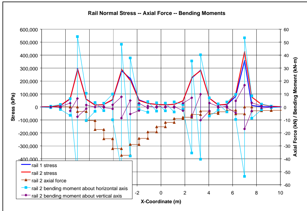
Figure 3-26: Combined Maximum Vertical (YY) and Lateral (ZZ) Rotation – Rail Normal Stress (kPa) – Axial Force (kN) – Bending Moments (kN-m).
