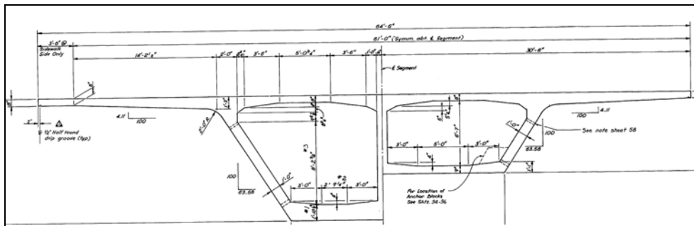
Figure 3-33: Typical Superstructure Cross-Section
