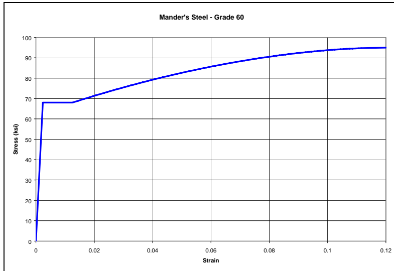
Figure 3-6: Typical Steel Stress-Strain Relation
