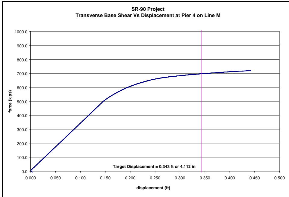
Figure 3-70: Column Force vs. Displacement at Pier 4 on Line M
