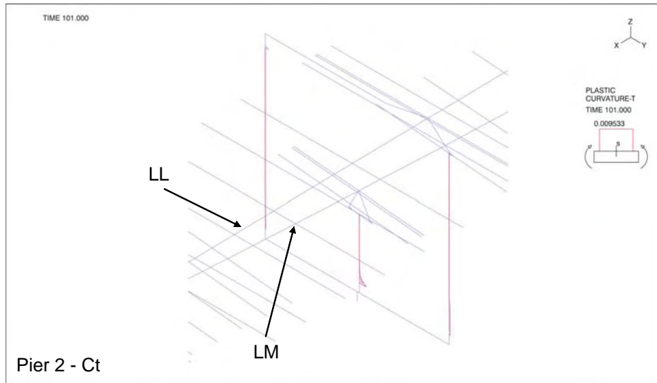
Figure 3-50: Plastic Curvature about Longitudinal Axis (T-axis) – Pier 2
