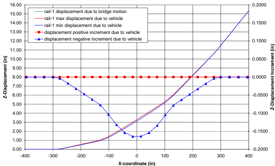
Figure 3-33: Rail Vertical (Z) Displacements due to Joint Combined Lateral (ZZ) and Vertical (YY) Rotation and Wheel Reactions.
