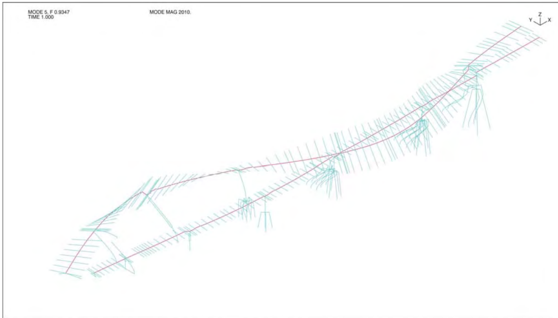
Figure 3-40: Mode Shape 5 (Transverse Line L – Period = 1.07 sec)
