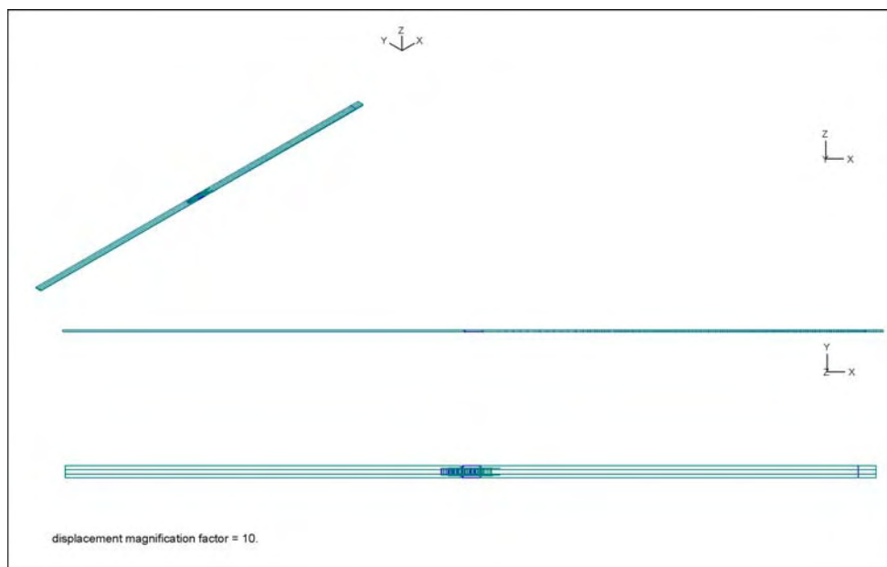
Figure 3-9: Maximum Longitudinal (X) Translation – Deformed Mesh.
