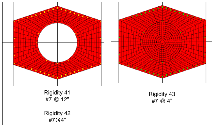
Figure 3-13: LL Pier 4 – SPEMC Model
