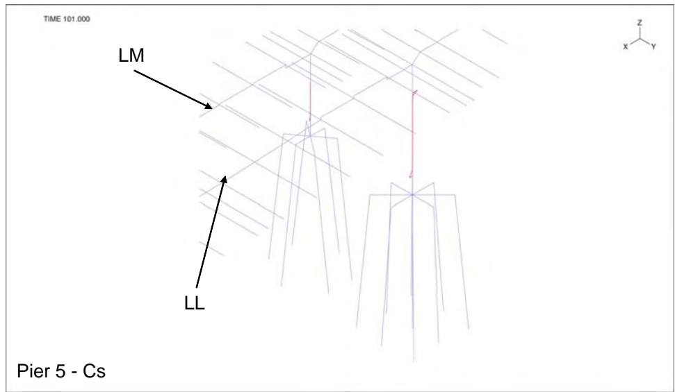
Figure 3-54: Plastic Curvature about Transverse Axis (S-axis) – Pier 5
