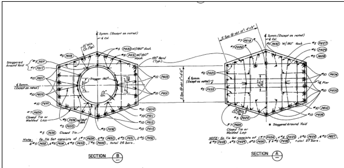
Figure 3-16: LL Pier 6 – drawing 296
