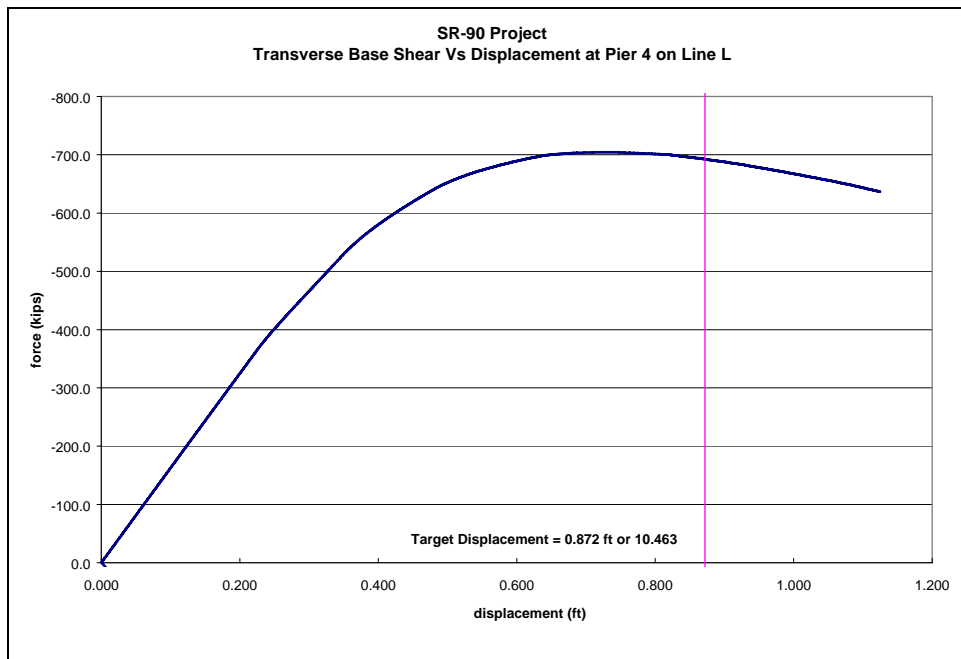
Figure 3-63: Column Force vs. Displacement at Pier 4 on Line L
