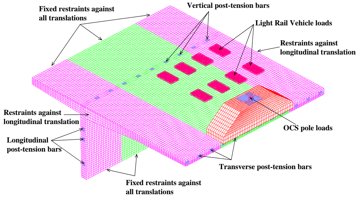
Figure 2-8: Substructure Model Boundary of a Cantilever Model
