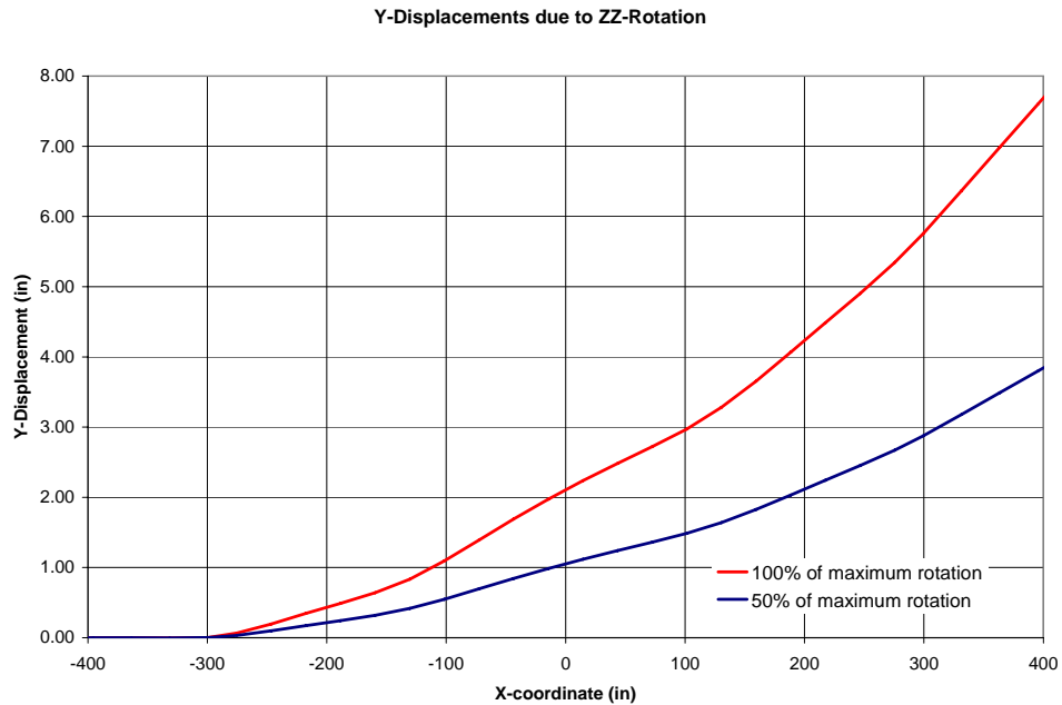
Figure 3-18: Rail Lateral (Y) Displacements due to Joint Lateral (ZZ) Rotation.
