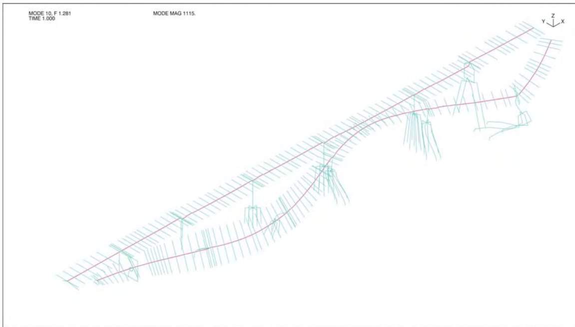
Figure 3-45: Mode Shape 10 (Transverse Line M – Period = 0.78 sec)
