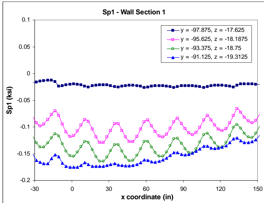
Figure 3-7: Principal Tensile Stress Variation in the x-direction at Wall Section 1 – Self Weight +Post Tension Forces +Light Rail Vehicle Loads +OCS Loads (Case 1)
