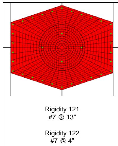
Figure 3-21: LM Pier 2 – SPEMC Model
