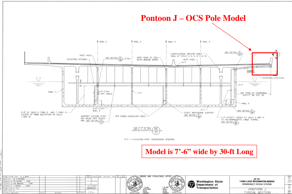
Figure 2-4: Substructure Model Boundary selected for OCS Pole Analysis
