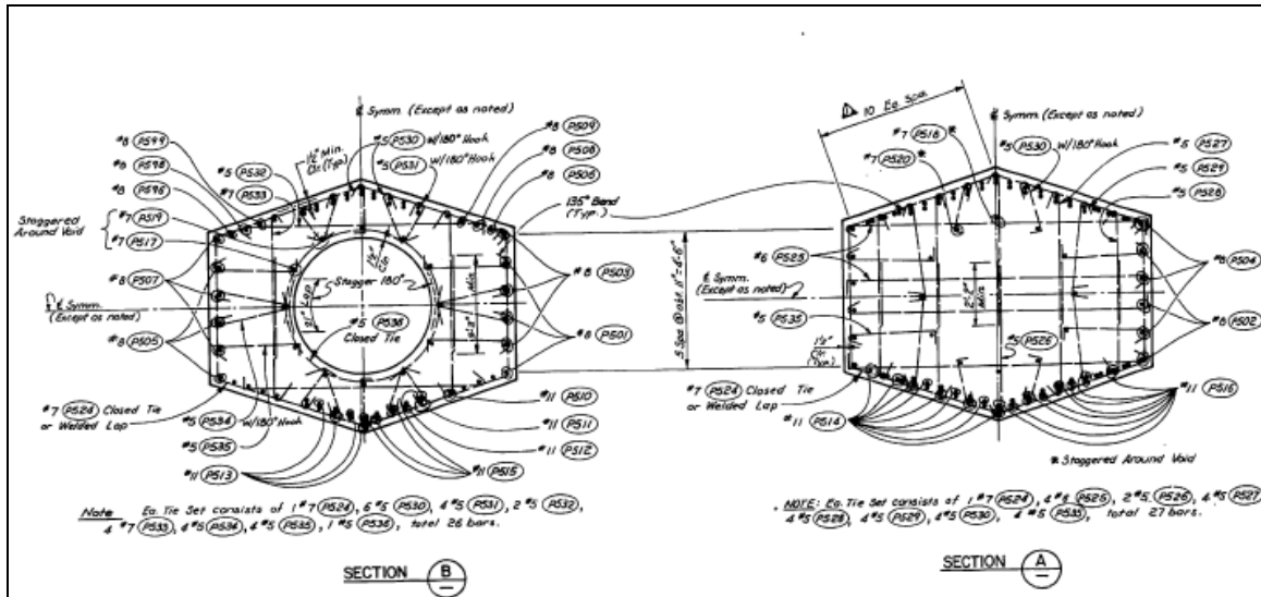
Figure 3-14: LL Pier 5 – drawing 295
