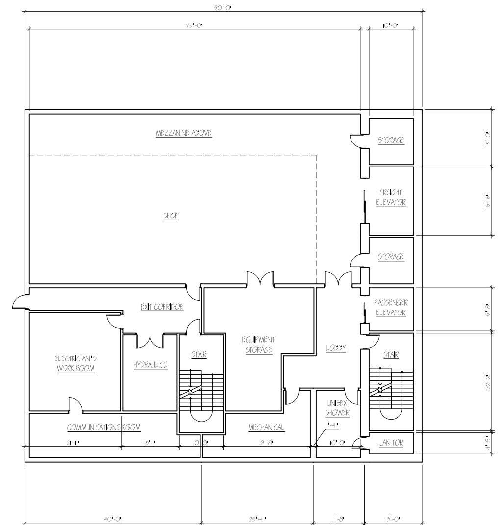
SHOP LEVEL FLOOR PLAN
