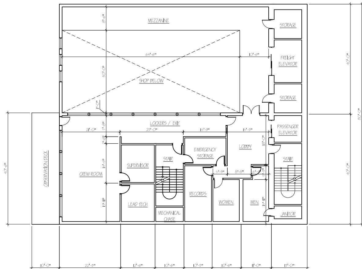
CREW LEVEL FLOOR PLAN
