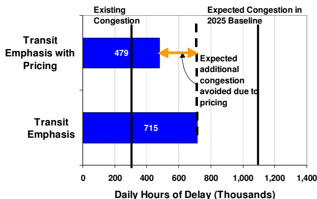
Figure 15 Effectiveness of Freeway Value Pricing in Central Puget Sound Region
