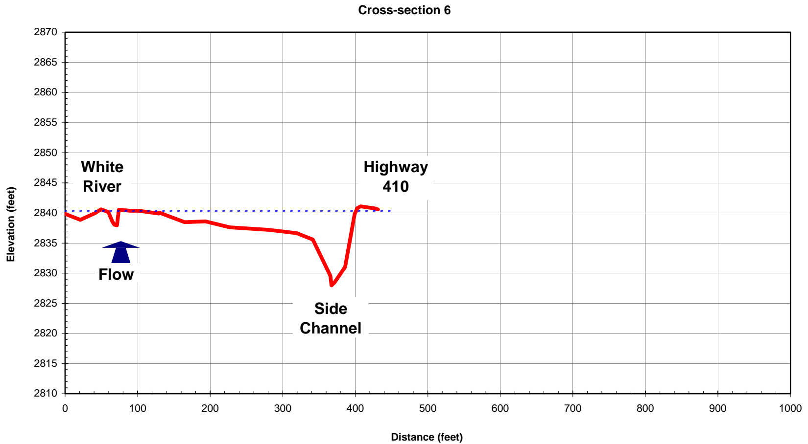
Figure D-8. Cross-section 6 (upstream end of site 4).
