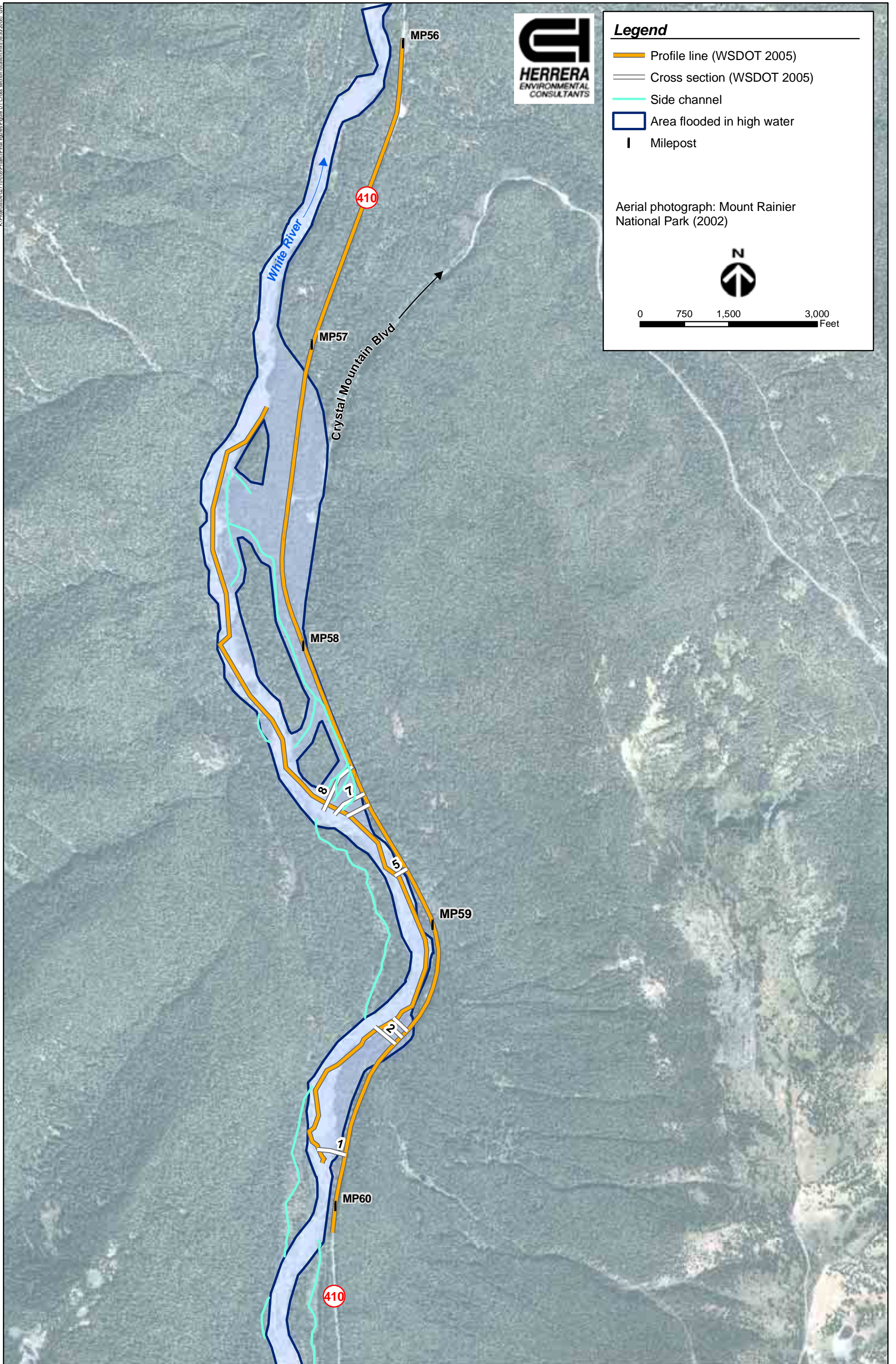
Figure D-1. Profile and cross-section locations on the White River, Pierce County, Washington.
