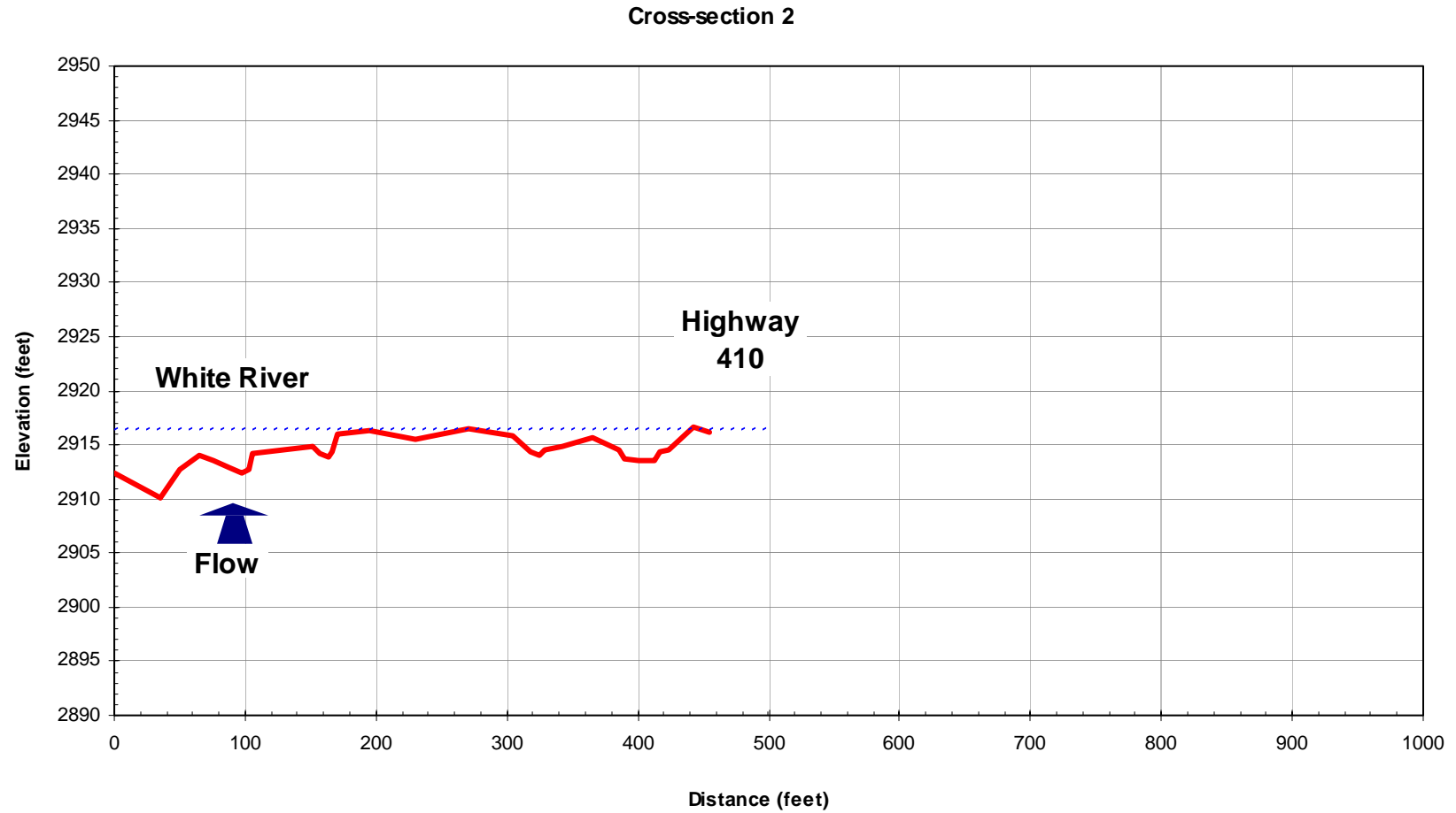
Figure D-4. Cross-section 2 (Site 8).
