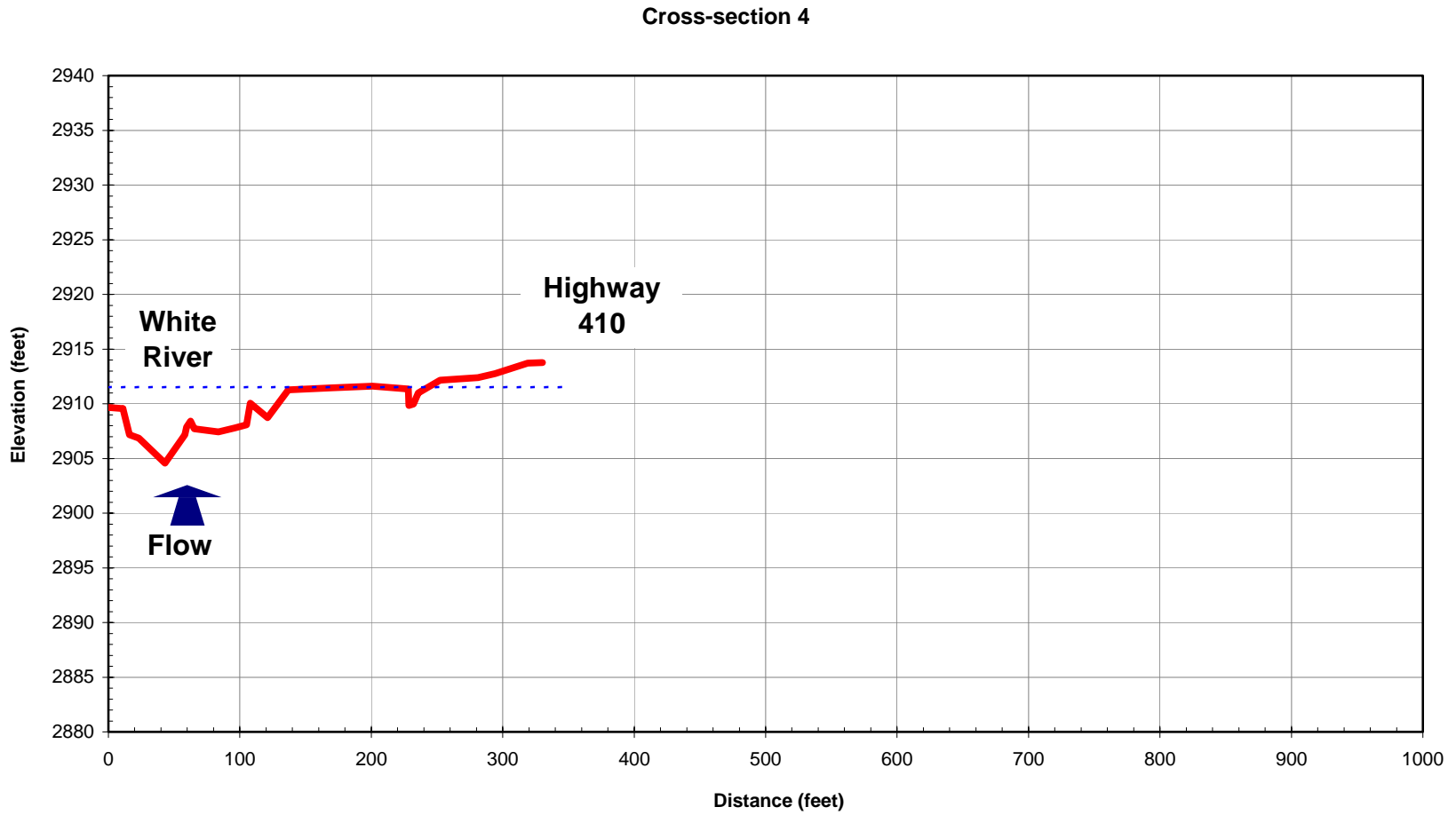
Figure D-6. Cross-section 4 (Site 8).
