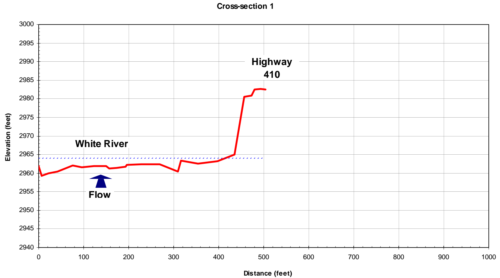
Figure D-3. Cross-section 1 (upstream of Site 8).
