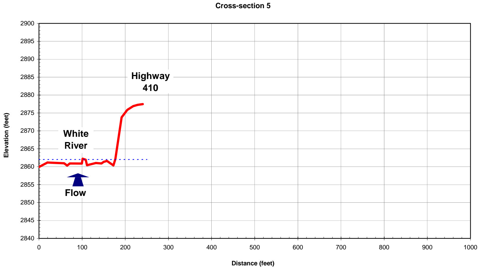
Figure D-7. Cross-section 5 (Site 6).
