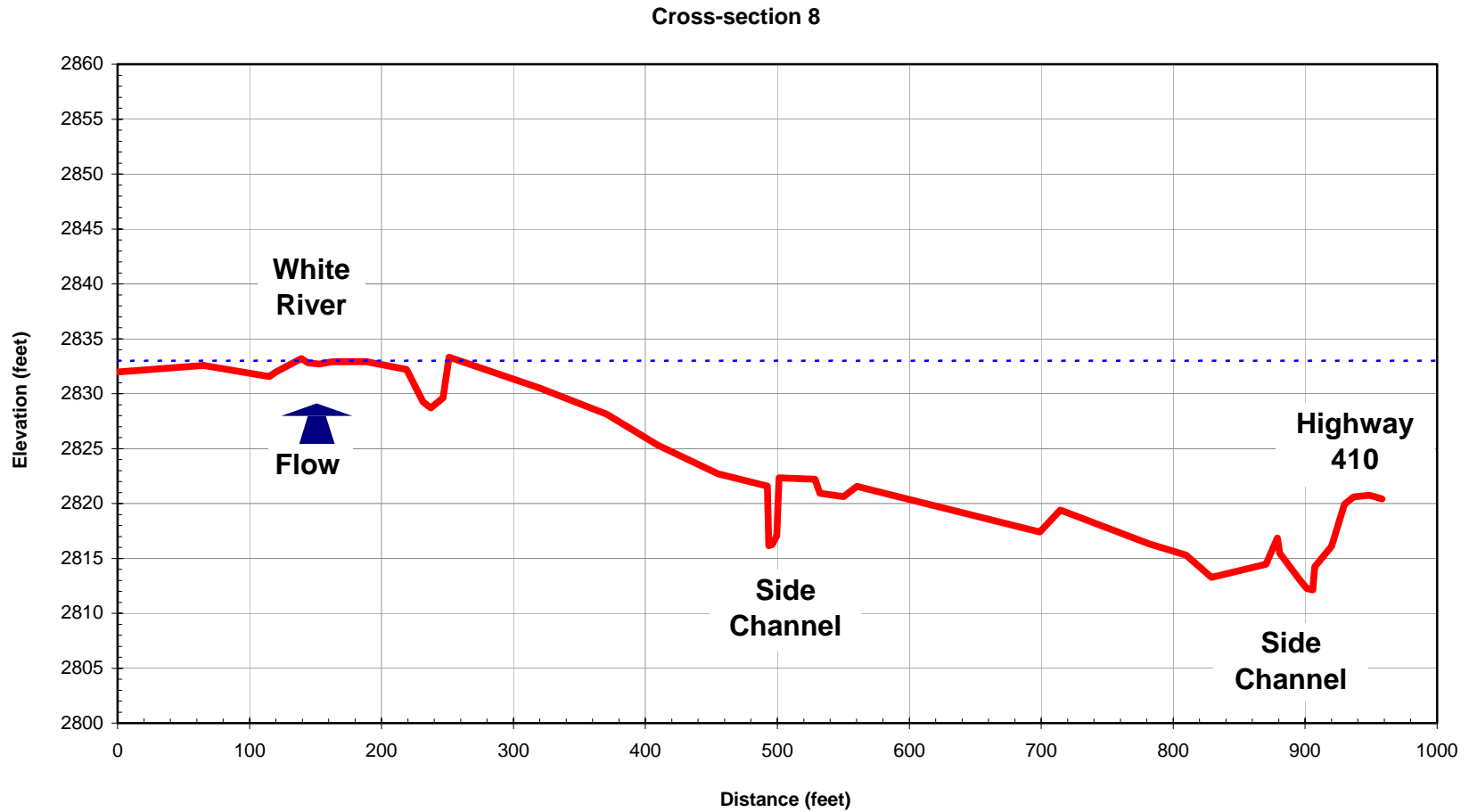
Figure D-10. Cross-section 8 (Site 4).
