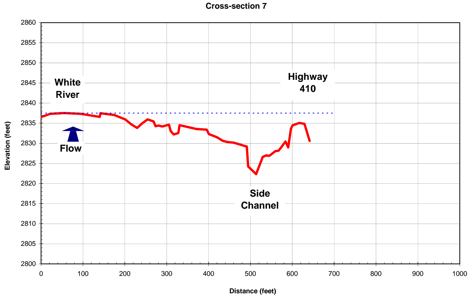
Figure D-9. Cross-section 7 (Site 4).
