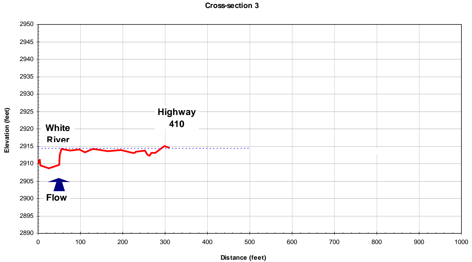
Figure D-5. Cross-section 3 (Site 8).
