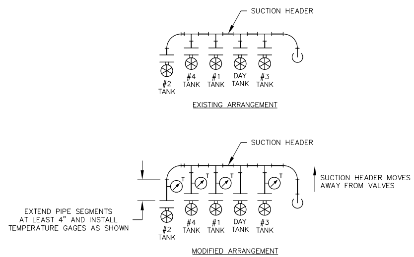
DETAIL 22-A FO TANK SUCTION MANIFOLD (OVERHEAD VIEW)
