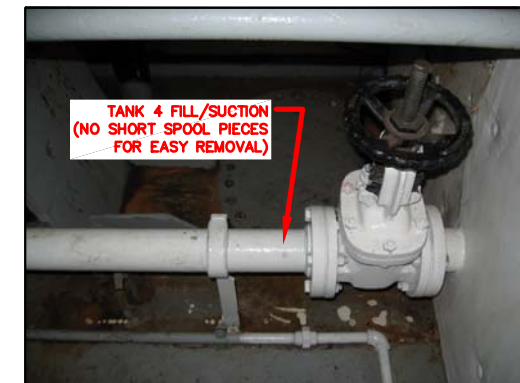
PHOTO 10-A FO STORAGE TANK 4 FILL/SUCTION
