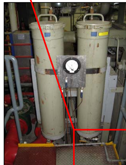
PHOTO 15-A EXISTING FUEL FILTER NO. 1 SAMPLE LINES (NO MODIFICATION REQUIRED)
