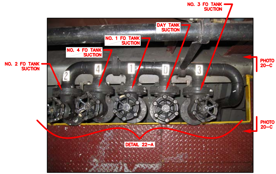
PHOTO 22-C FO TANK SUCTION MANIFOLD (OVERHEAD VIEW)
