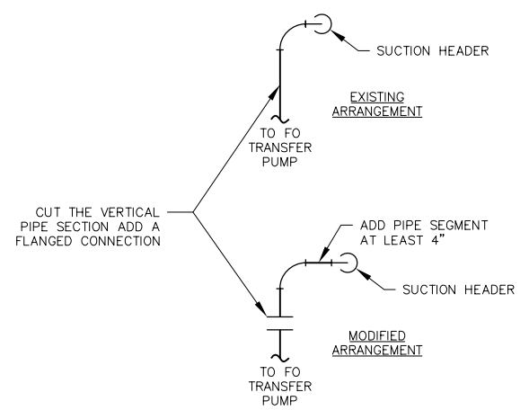
DETAIL 20-A FO TANK SUCTION MANIFOLD (SIDE PROFILE VIEW)
