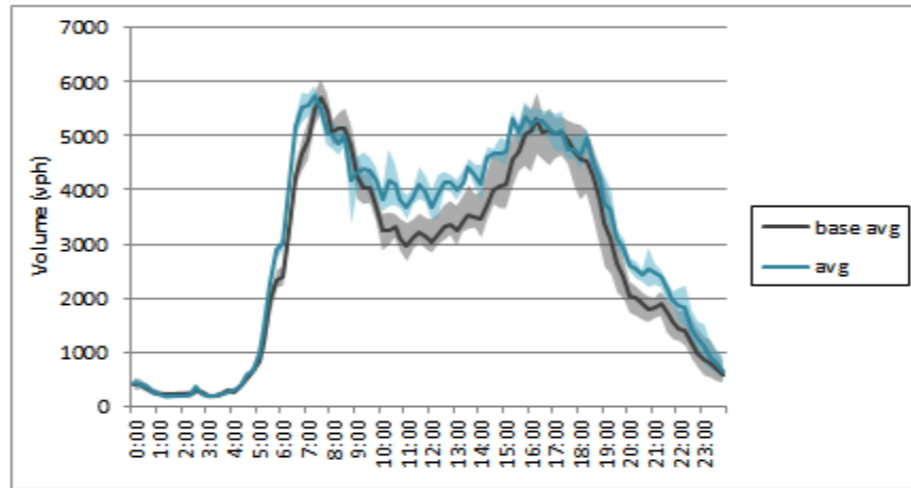
I-90 EB Volume - Week 6
