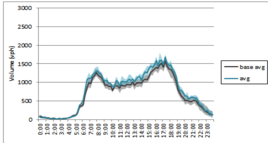
SR 522 EB Volume - Week 6
