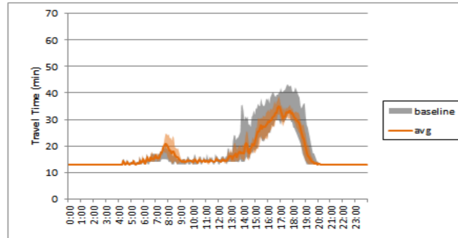
I-405 SB Travel Time - Bellevue to Tukwila - Week 6
