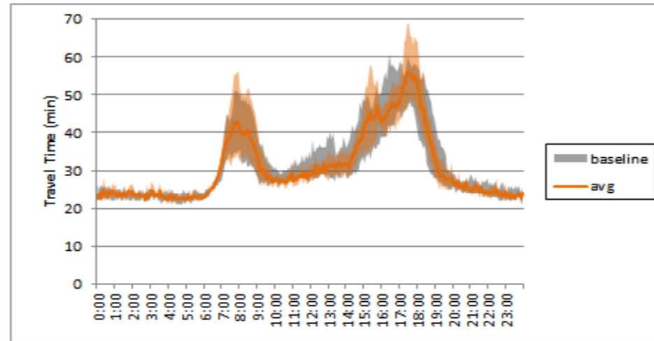
SR 522 EB Travel Time - Seattle to Woodinville - Week 6
