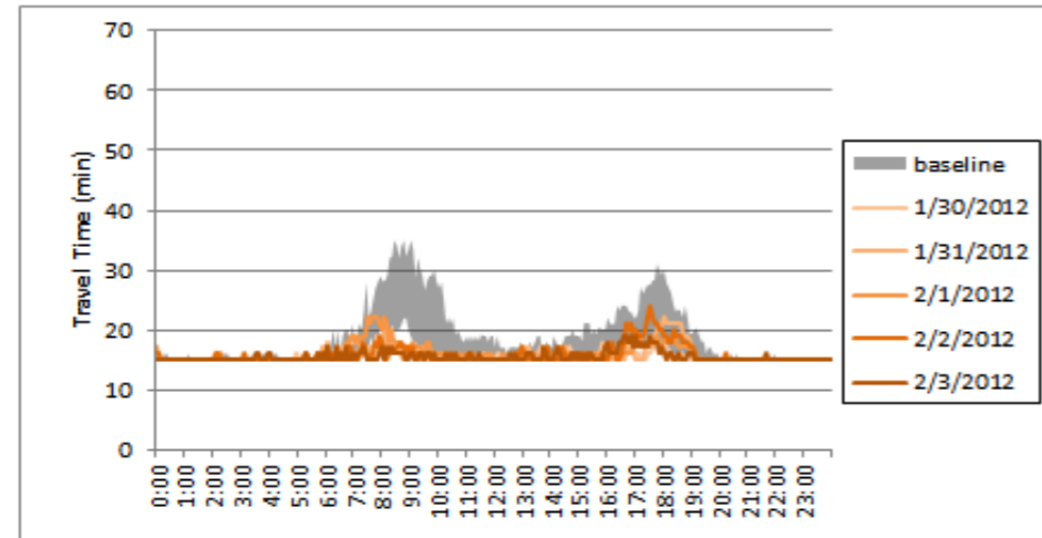
SR 520 EB Travel Time - Seattle to Redmond - Week 5
