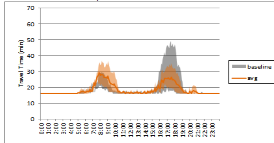
I-90 EB Travel Time - Seattle to Issaquah - Week 6
