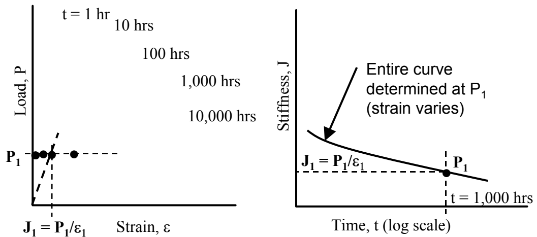
(b) Creep stiffness determined at constant load level.
