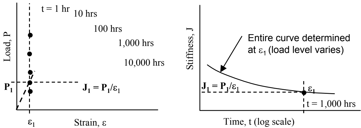
(a) Creep stiffness determined at constant strain level.
