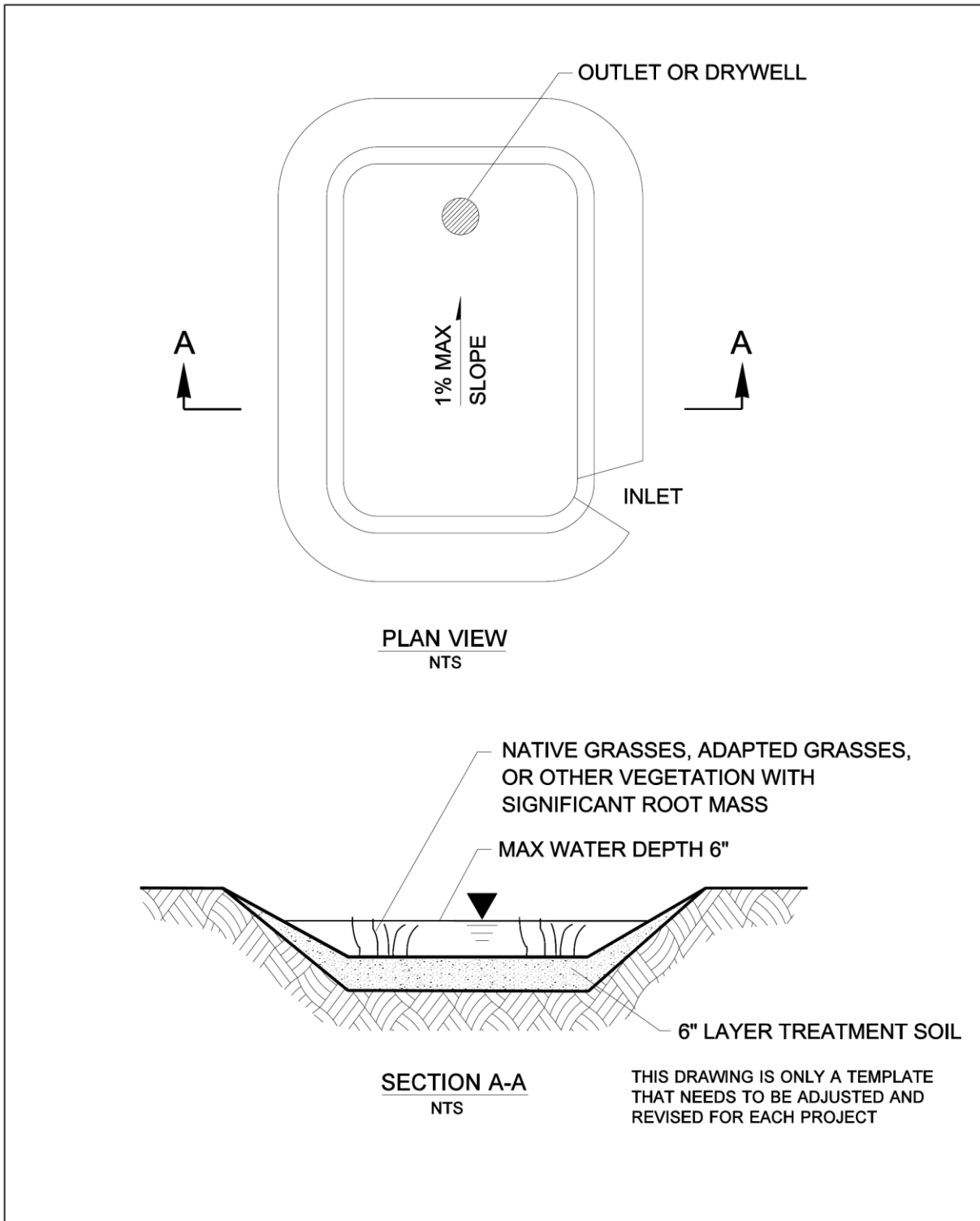
Figure 5-40 Bioinfiltration pond.
