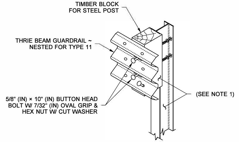
STEEL POST ASSEMBLY
