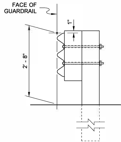
RAIL ASSEMBLY
