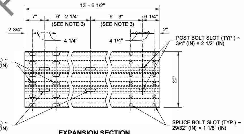
EXPANSION SECTION
