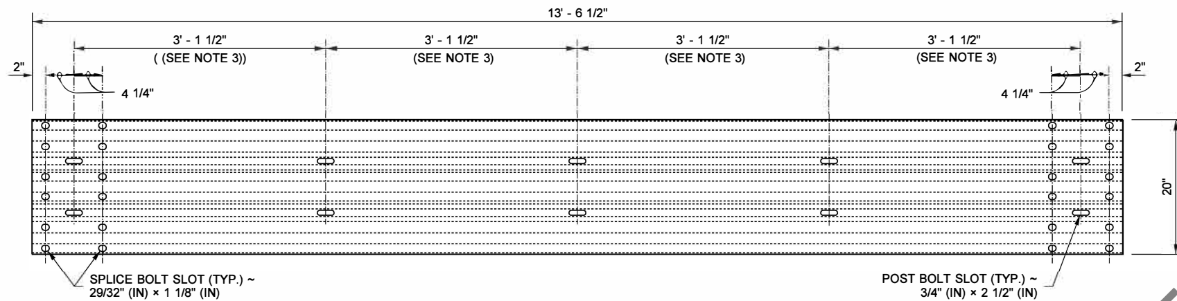
TYPICAL RAIL ELEMENT
