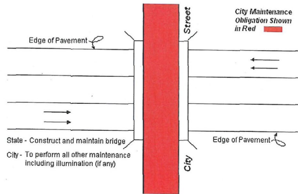
EXISTING CITY STREET CROSSED BY NEW STATE HIGHWAY UNDERPASS Figure 2
