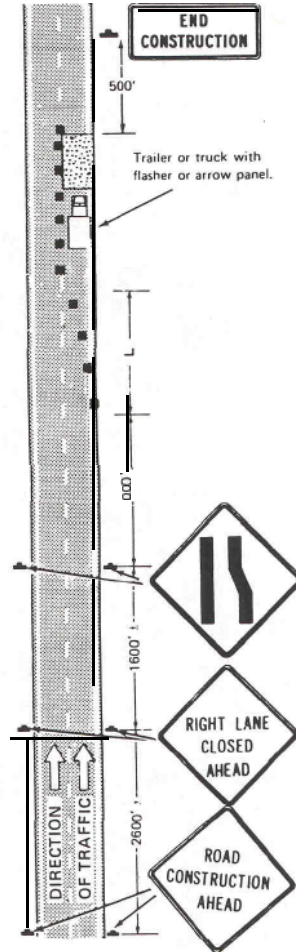
Typical application—daytime maintenance operations of short duration on a 4-lane divided roadway where half of roadway is closed.
