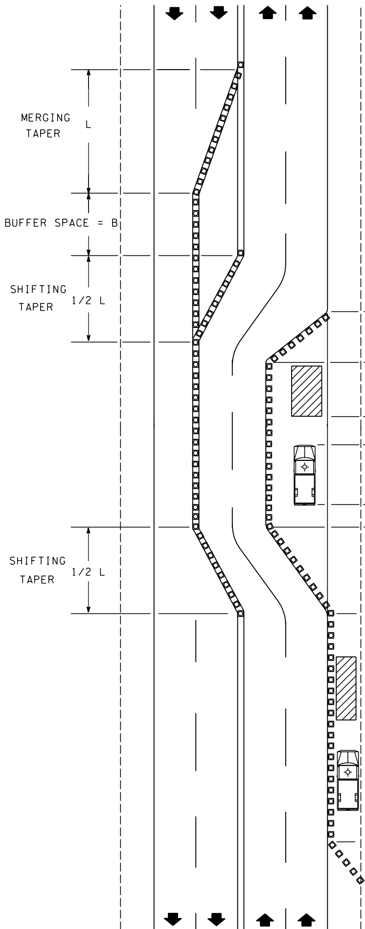
TAPER & BUFFER SPACE DETAILS
