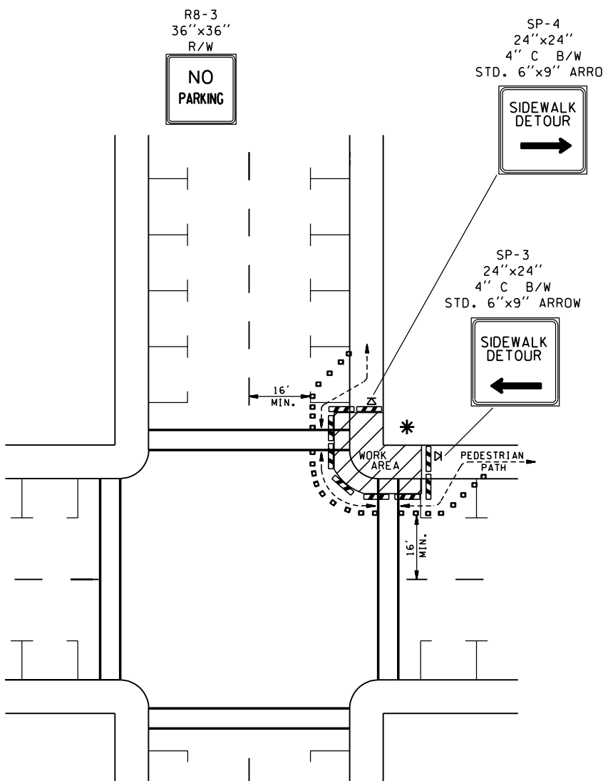
PEDESTRIAN DETOUR (NONWORKING HOURS)
