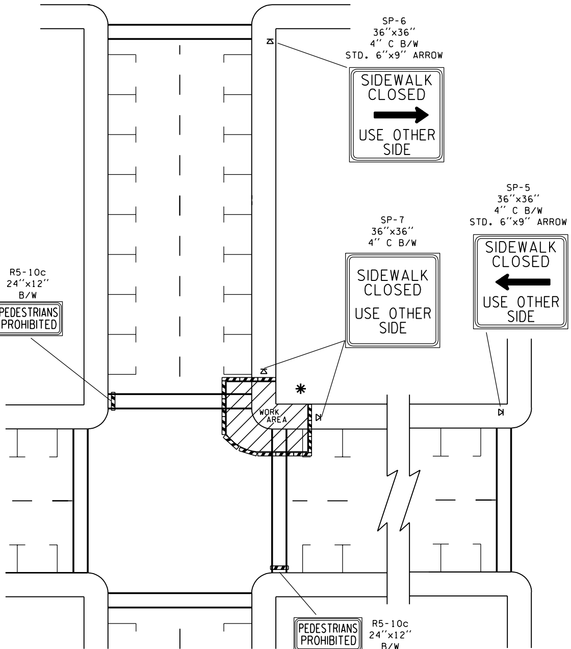
PEDESTRIAN DETOUR (WORKING HOURS)
